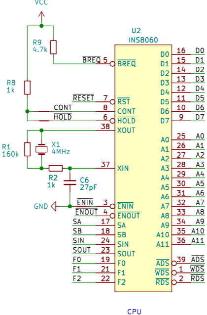
CPU
