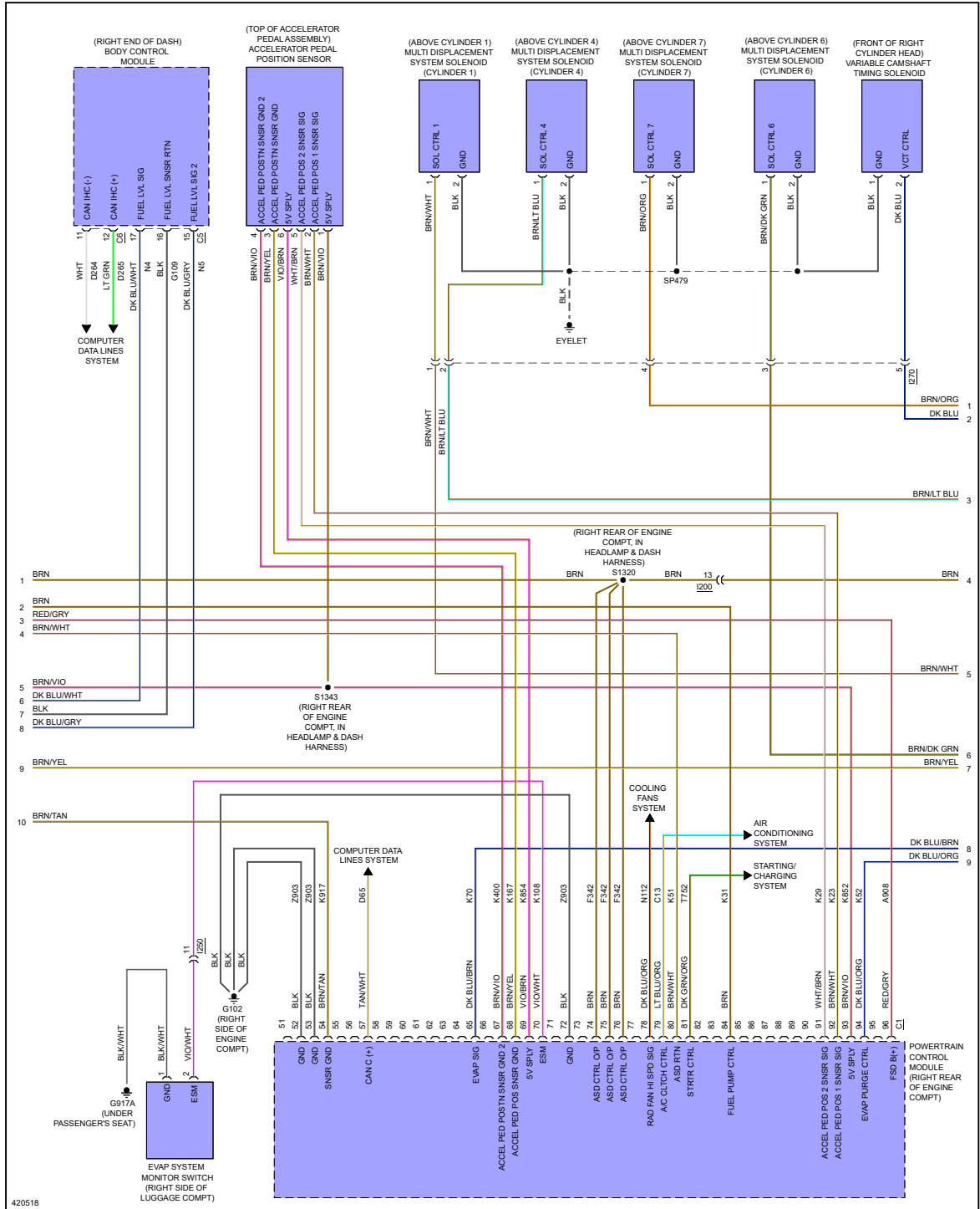
Fig 2: 5.7L, Engine Performance Circuit (2 of 5)
