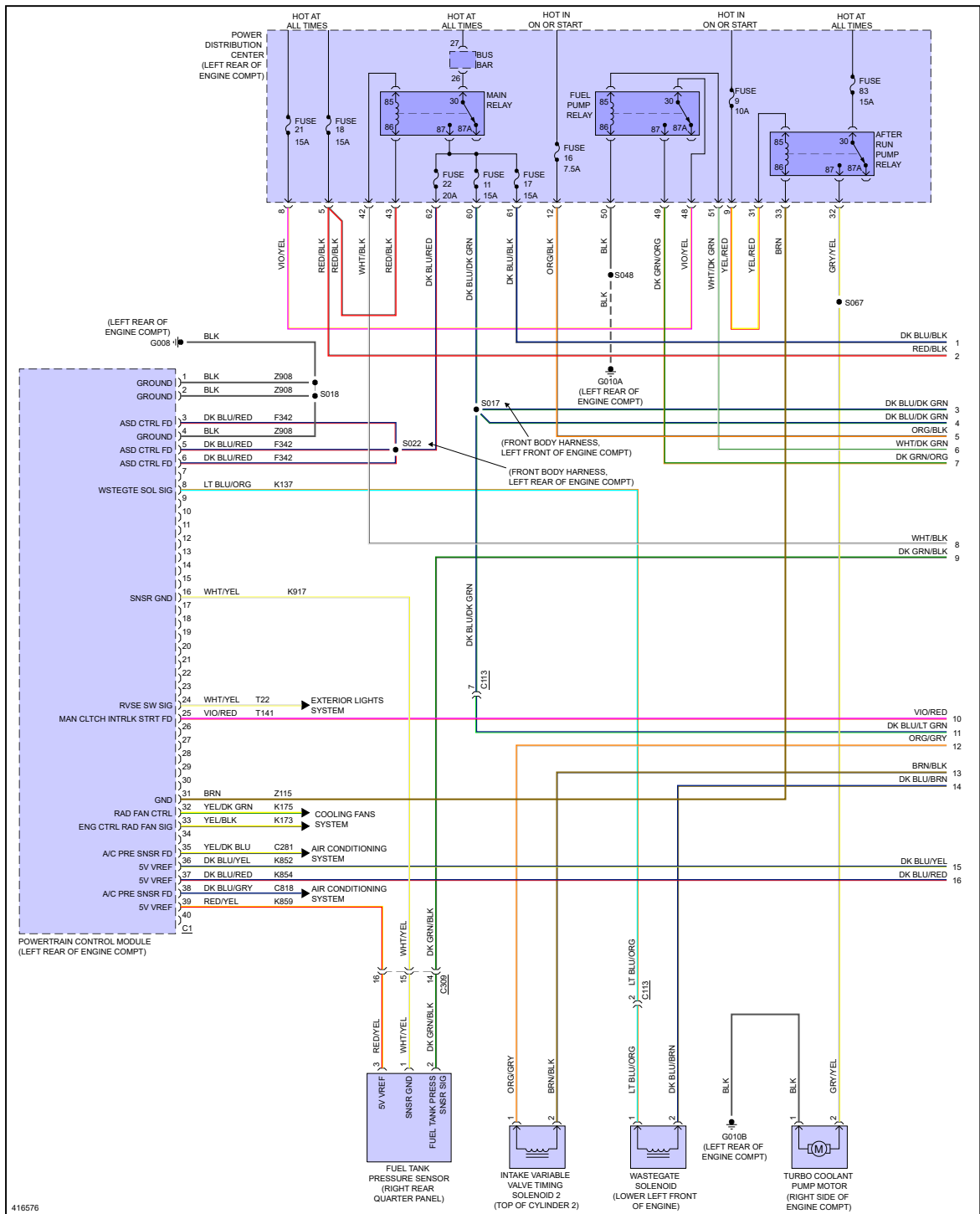
Fig 1: 1.4L Turbo, Engine Performance Circuit (1 of 5)
