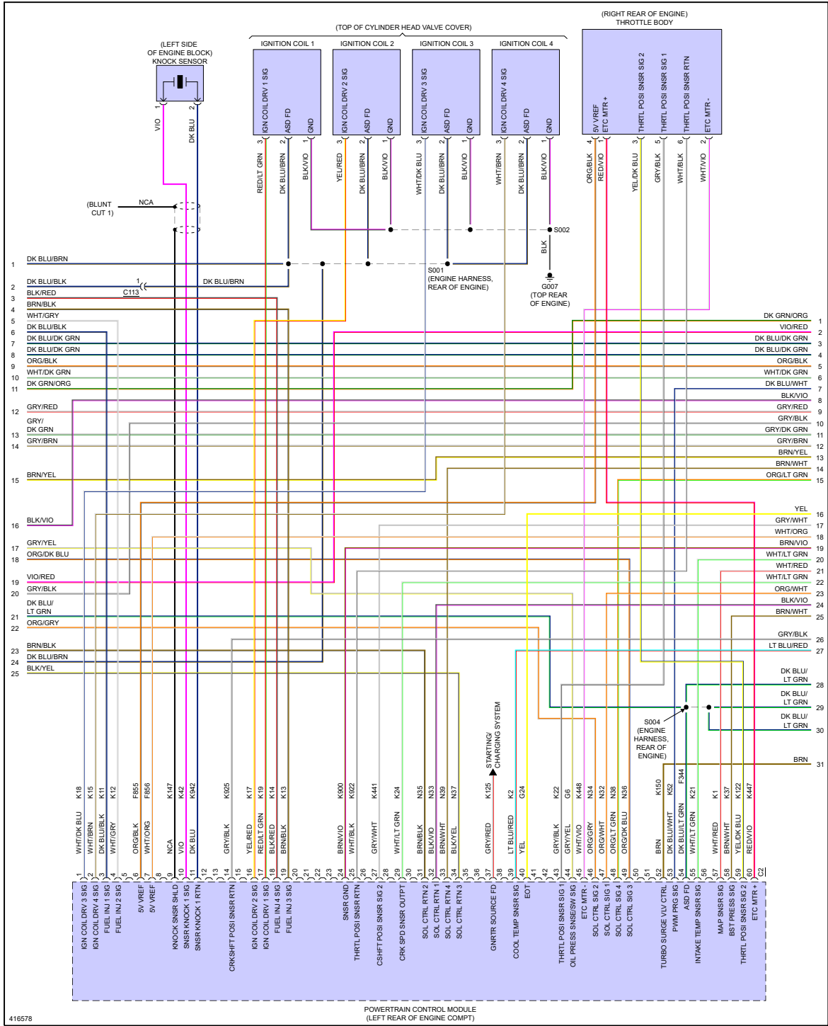
Fig 3: 1.4L Turbo, Engine Performance Circuit (3 of 5)
