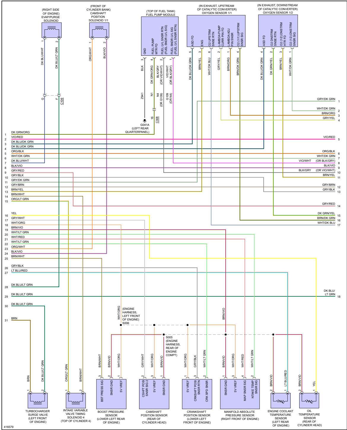
Fig 4: 1.4L Turbo, Engine Performance Circuit (4 of 5)
