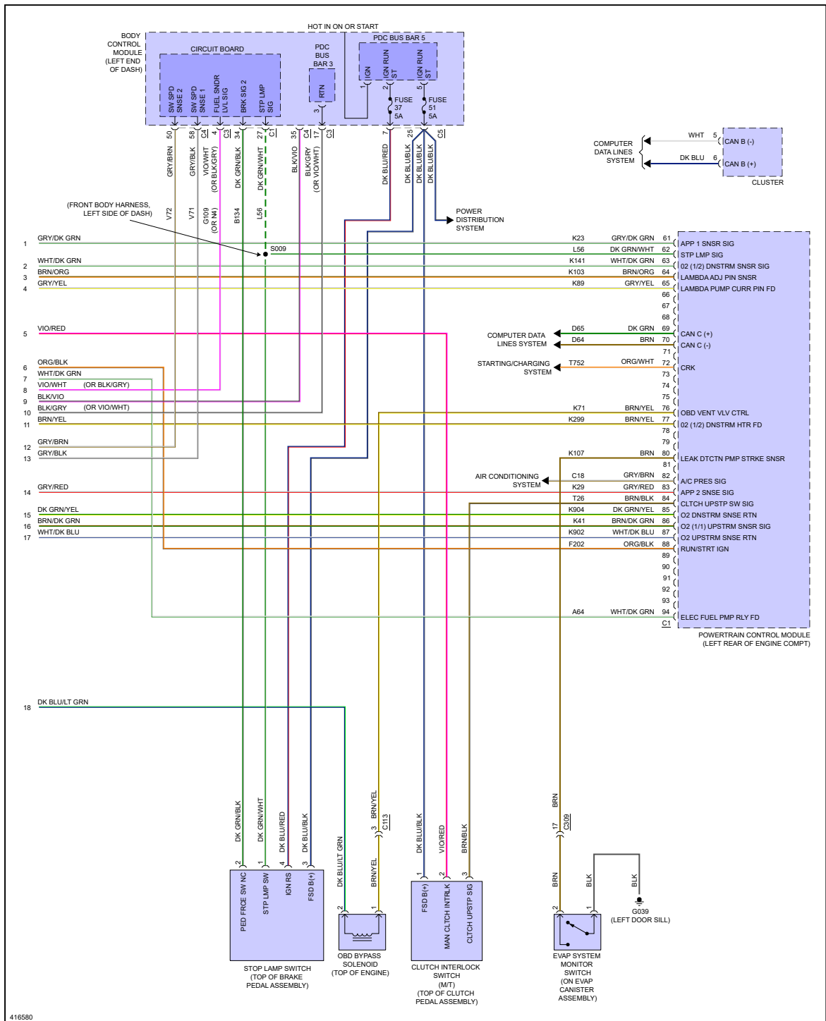
Fig 5: 1.4L Turbo, Engine Performance Circuit (5 of 5)
