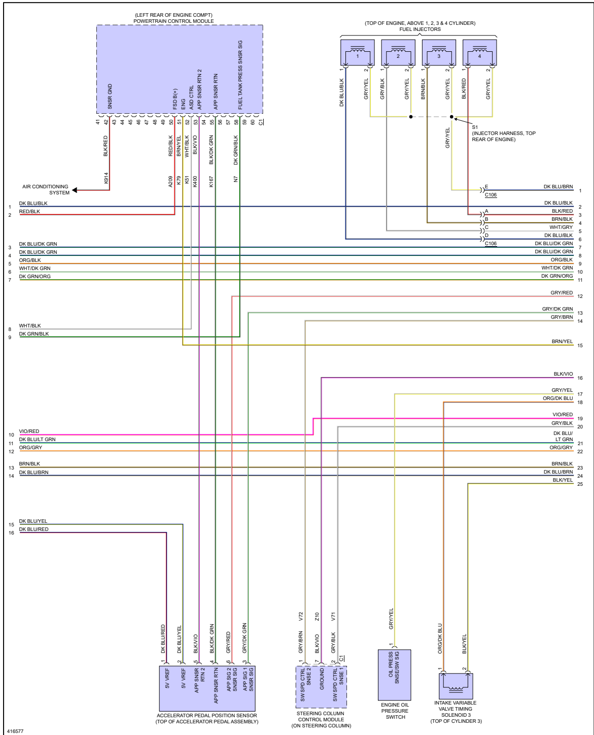
Fig 2: 1.4L Turbo, Engine Performance Circuit (2 of 5)
