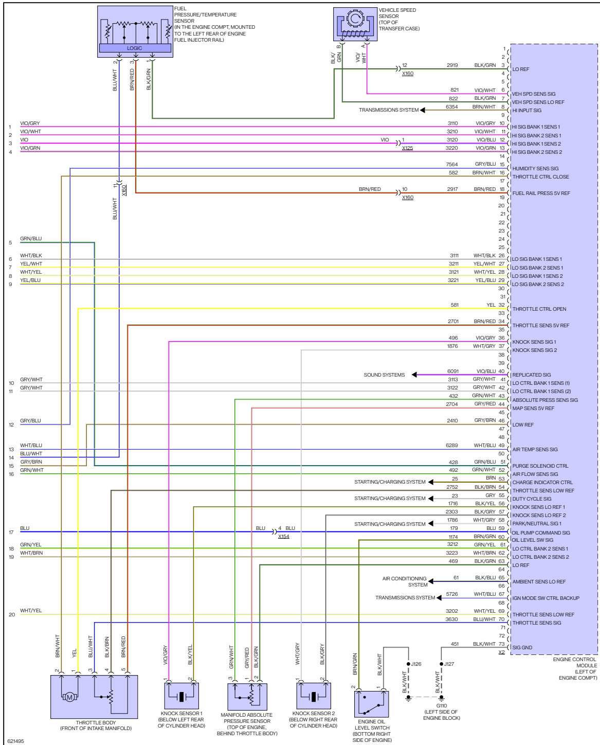
Fig 8: 5.3L VIN C, Engine Performance Circuit (8 of 8)
