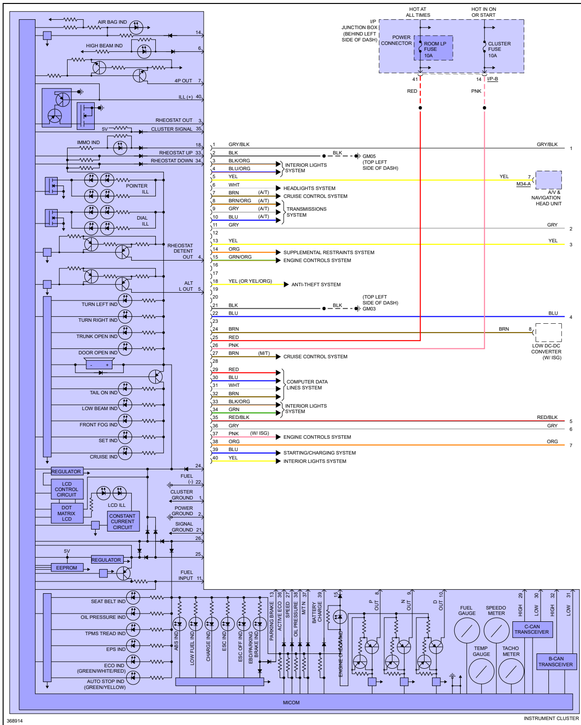
Fig 2: Instrument Cluster Circuit, W/ Super Vision (1 of 2)
