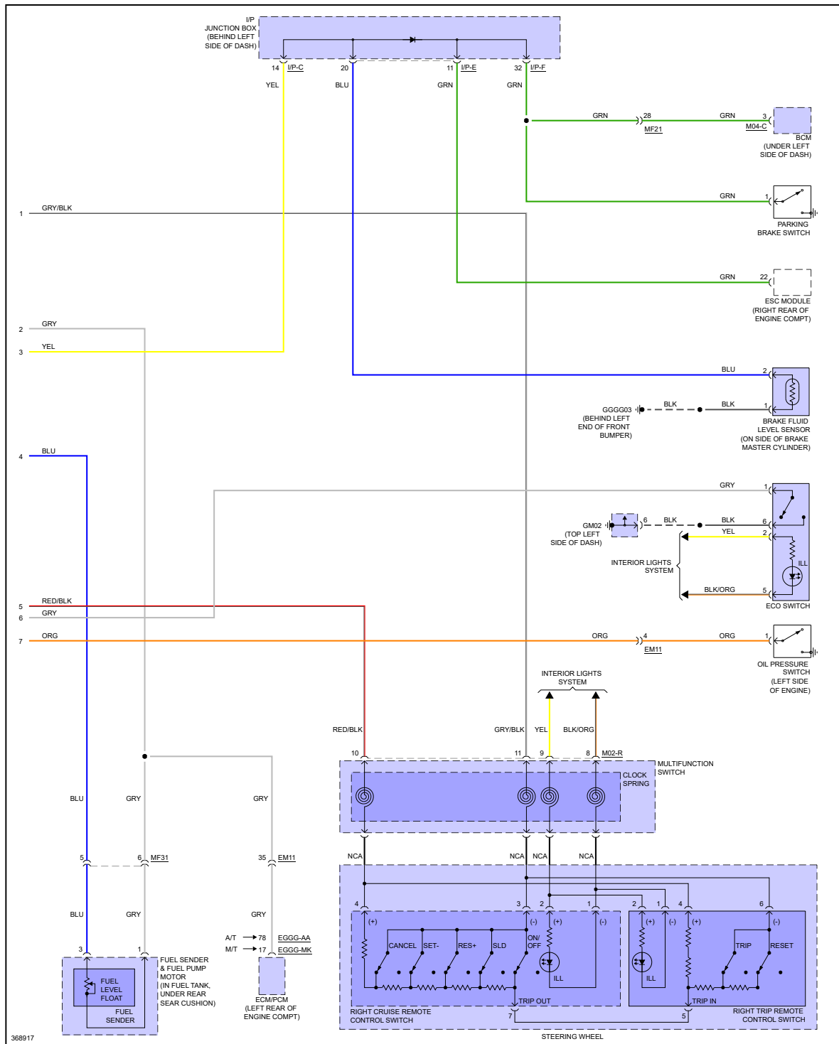
Fig 5: Instrument Cluster Circuit, W/O Super Vision (2 of 2)
