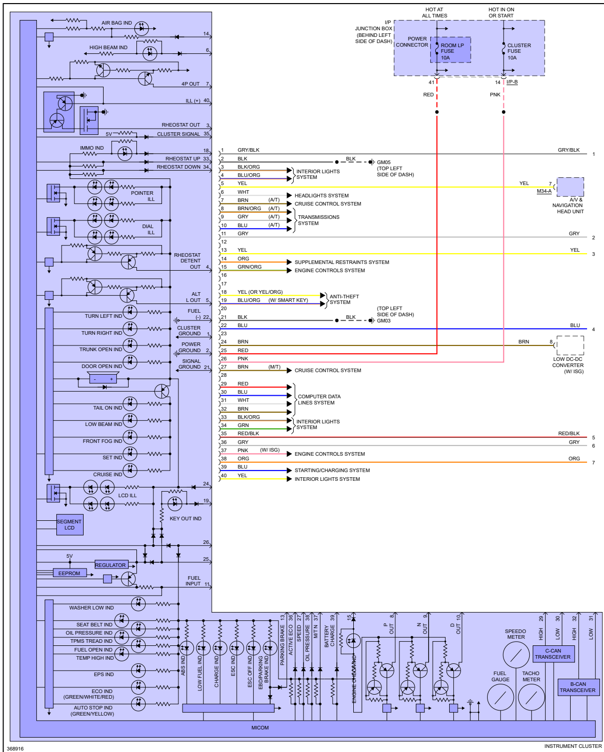
Fig 4: Instrument Cluster Circuit, W/O Super Vision (1 of 2)
