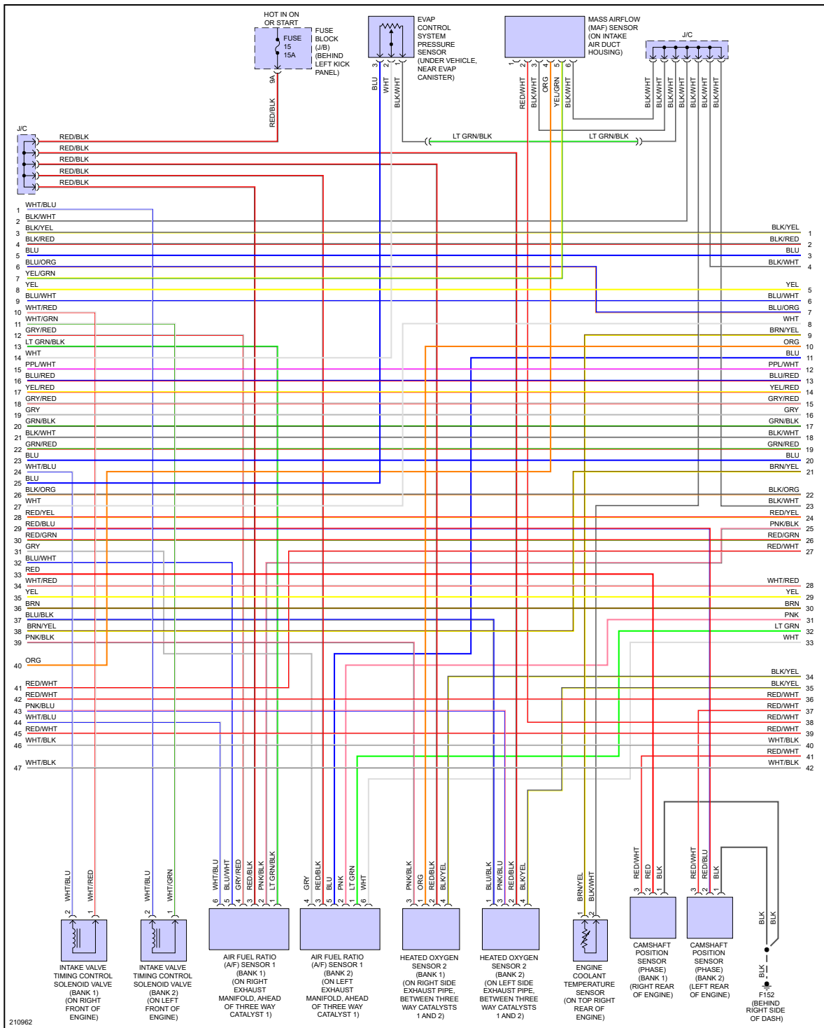
Fig 3: 3.5L, Engine Performance Circuit (3 of 4)
