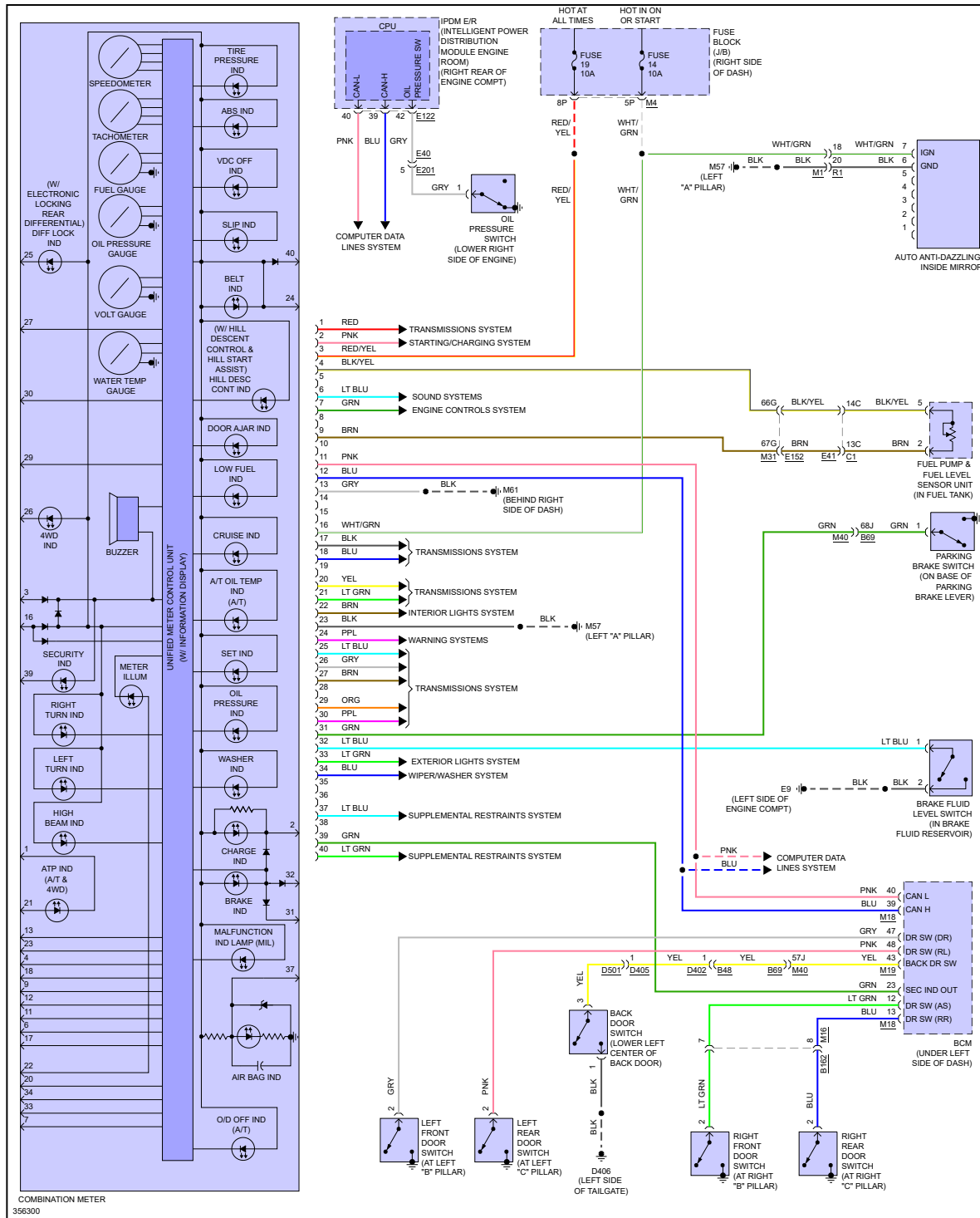
Fig 1: Instrument Cluster Circuit
