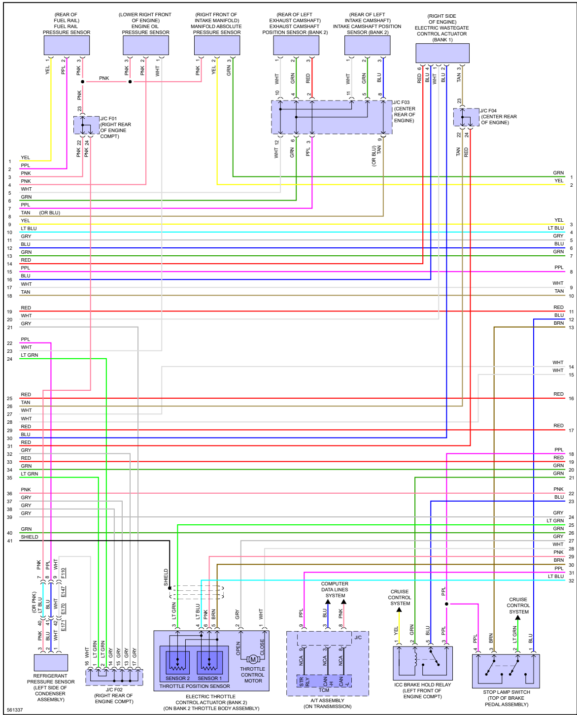
Fig 5: 3.0L Turbo, Engine Performance Circuit (5 of 8)
