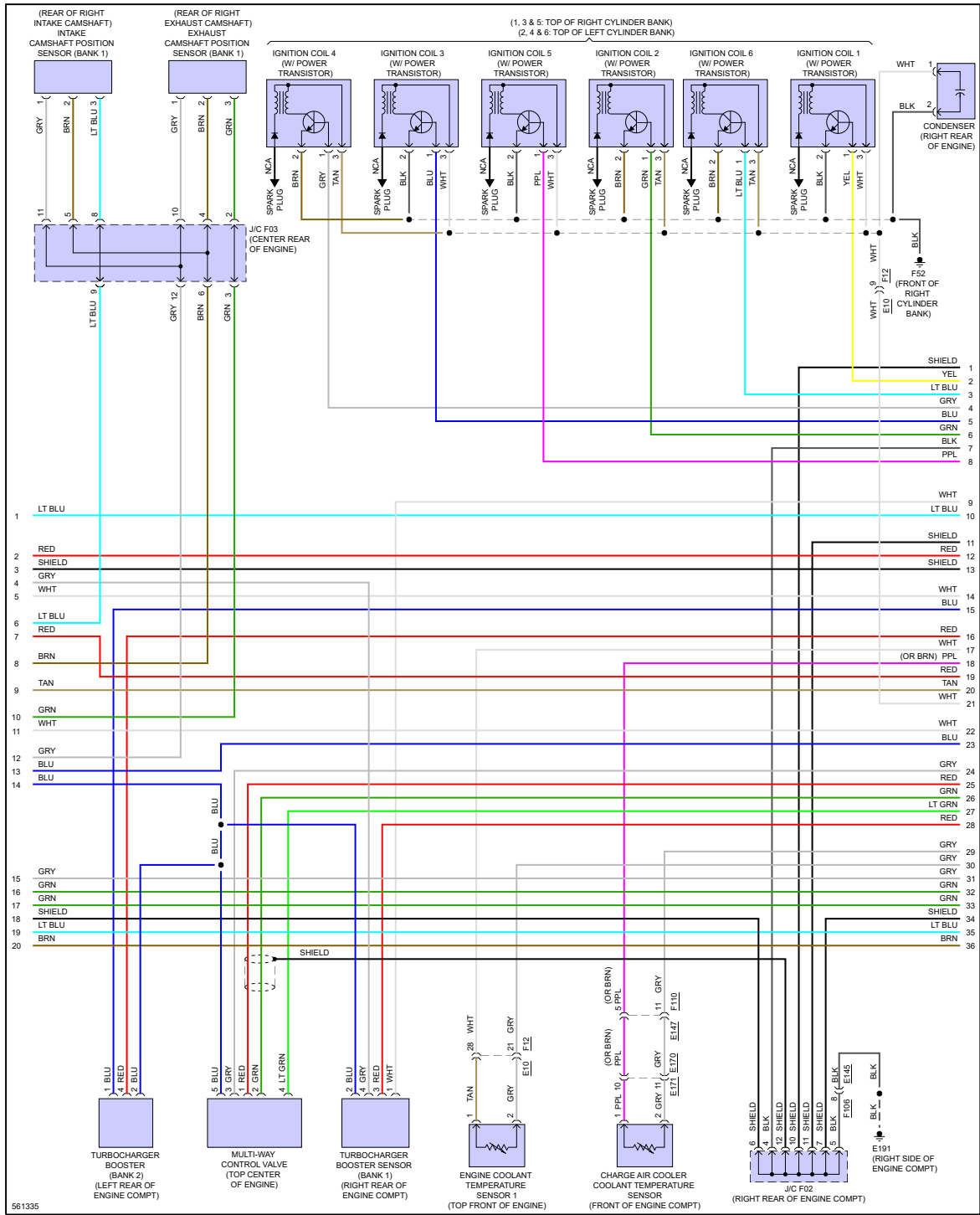
Fig 3: 3.0L Turbo, Engine Performance Circuit (3 of 8)
