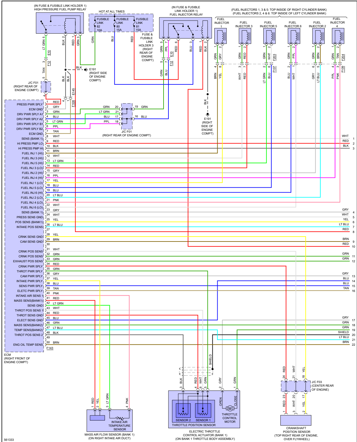
Fig 1: 3.0L Turbo, Engine Performance Circuit (1 of 8)
