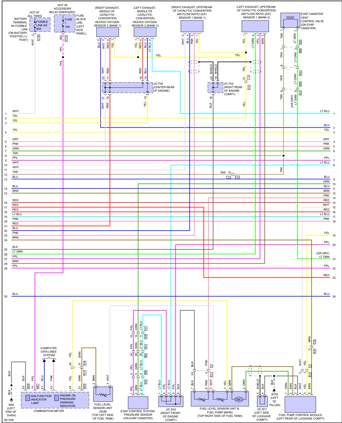
Fig 7: 3.0L Turbo, Engine Performance Circuit (7 of 8)
