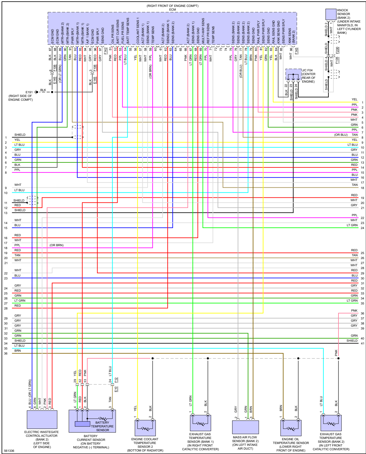
Fig 4: 3.0L Turbo, Engine Performance Circuit (4 of 8)
