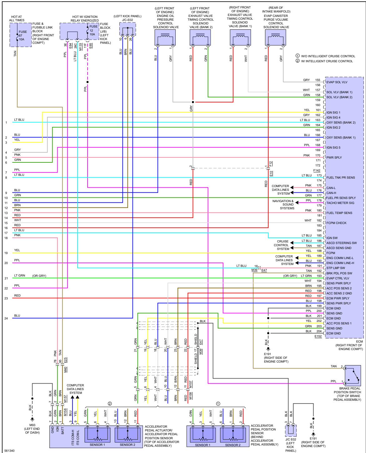
Fig 8: 3.0L Turbo, Engine Performance Circuit (8 of 8)
