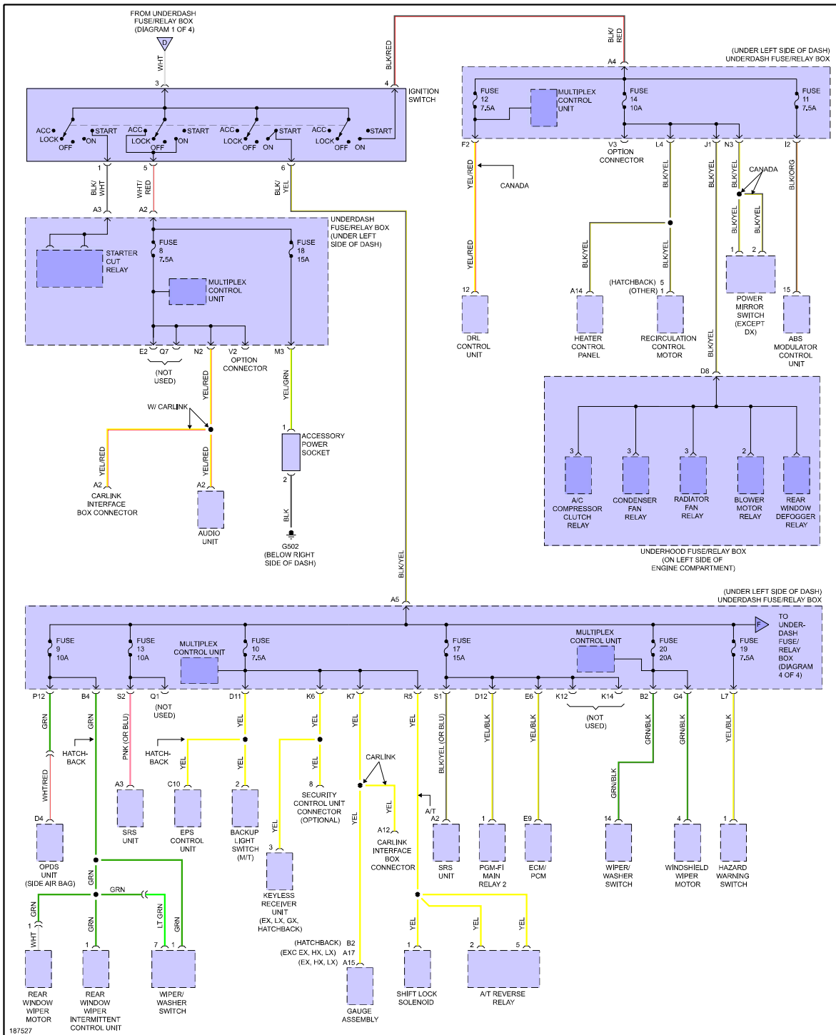
Fig 3: Power Distribution Circuit, Except Hybrid (3 of 4)
