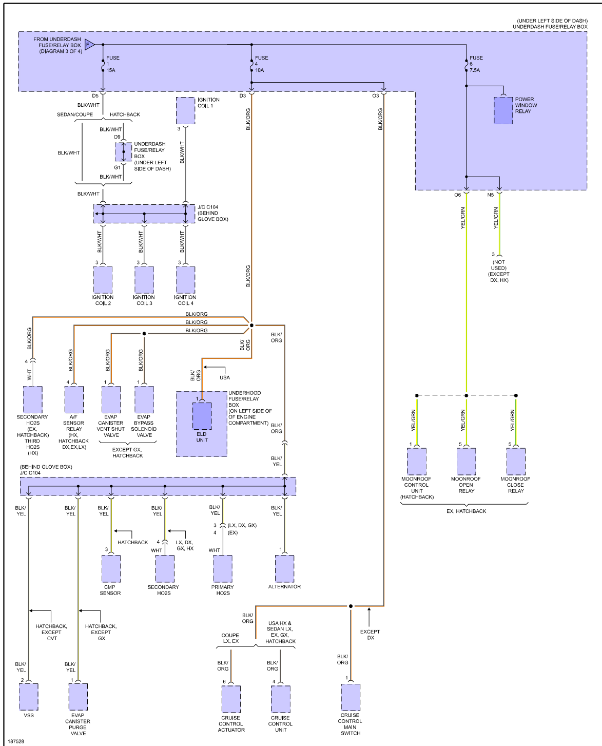
Fig 4: Power Distribution Circuit, Except Hybrid (4 of 4)
