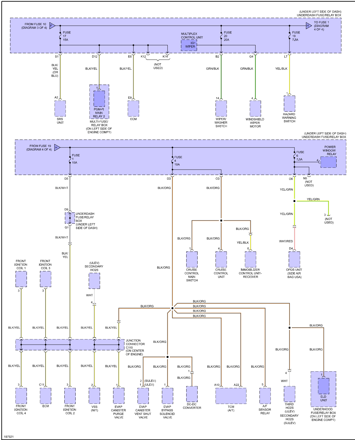
Fig 8: Power Distribution Circuit, Hybrid (4 of 4)
