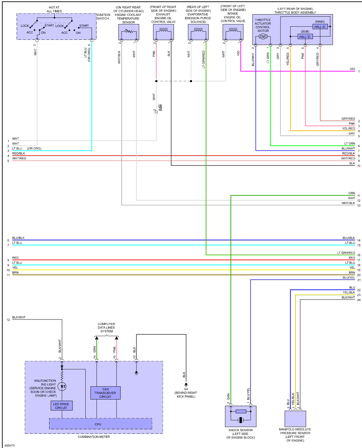
Fig 7: 2.0L Turbo, Engine Performance Circuit, Except Evolution (3 of 4)
