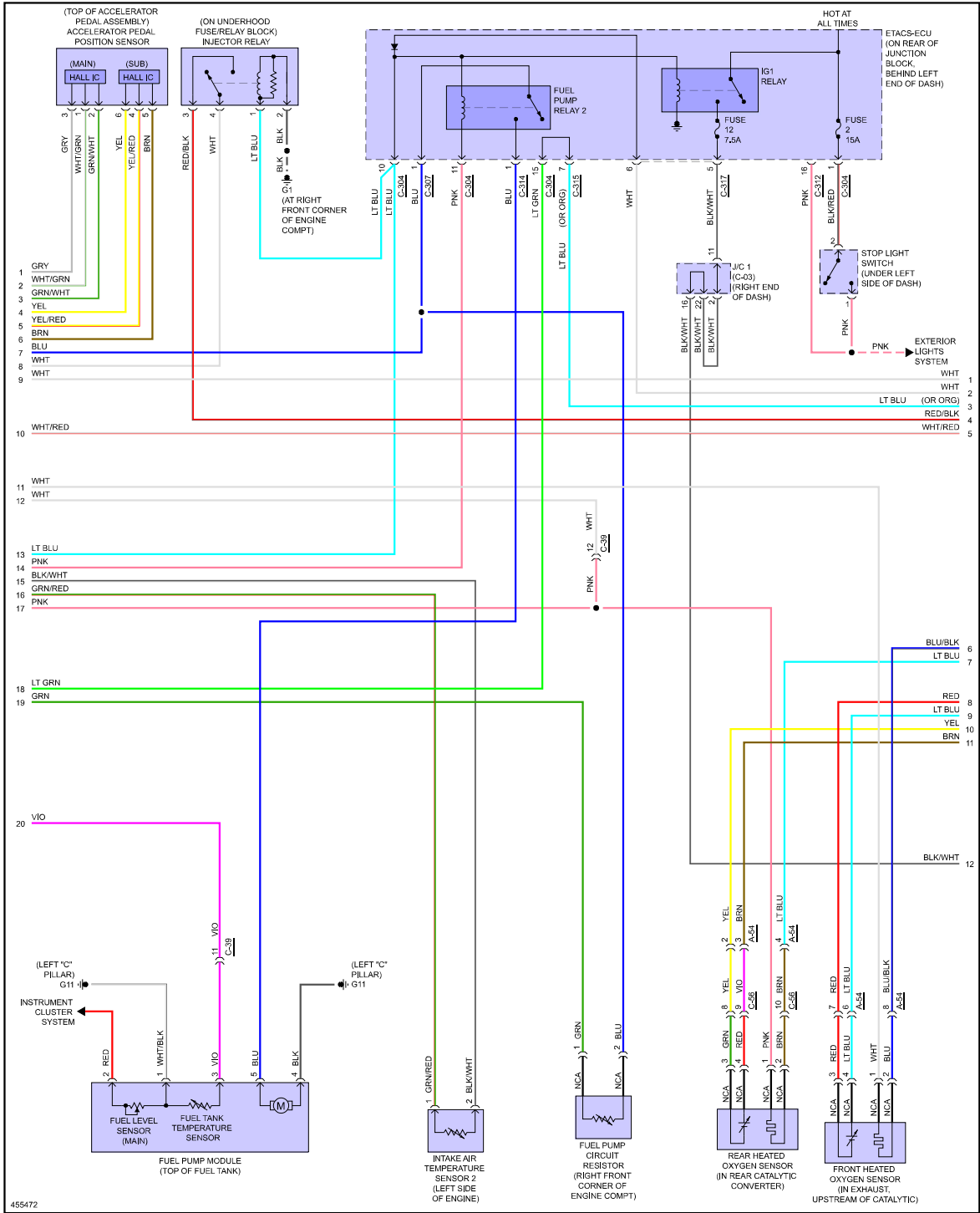
Fig 6: 2.0L Turbo, Engine Performance Circuit, Except Evolution (2 of 4)
