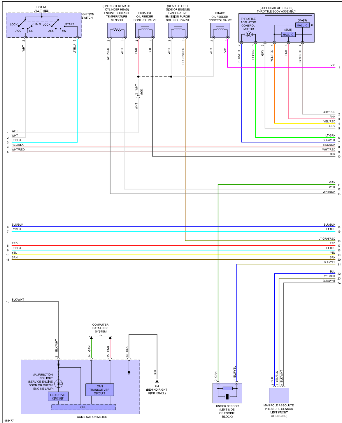
Fig 3: 2.0L Turbo, Engine Performance Circuit, Evolution (3 of 4)
