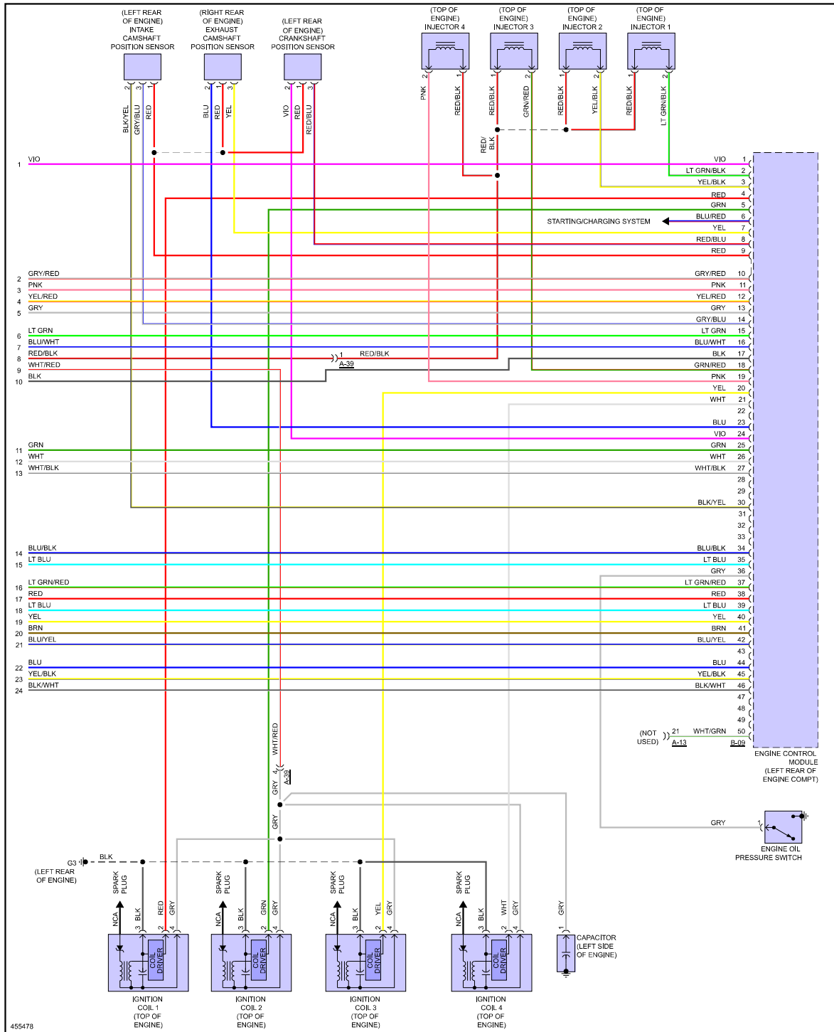
Fig 4: 2.0L Turbo, Engine Performance Circuit, Evolution (4 of 4)
