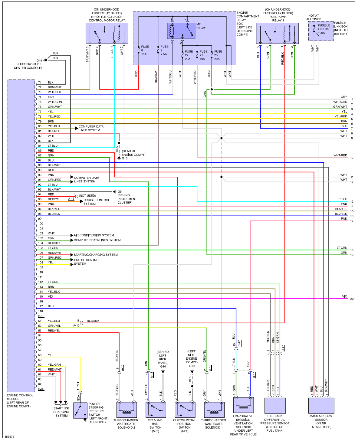
Fig 1: 2.0L Turbo, Engine Performance Circuit, Evolution (1 of 4)
