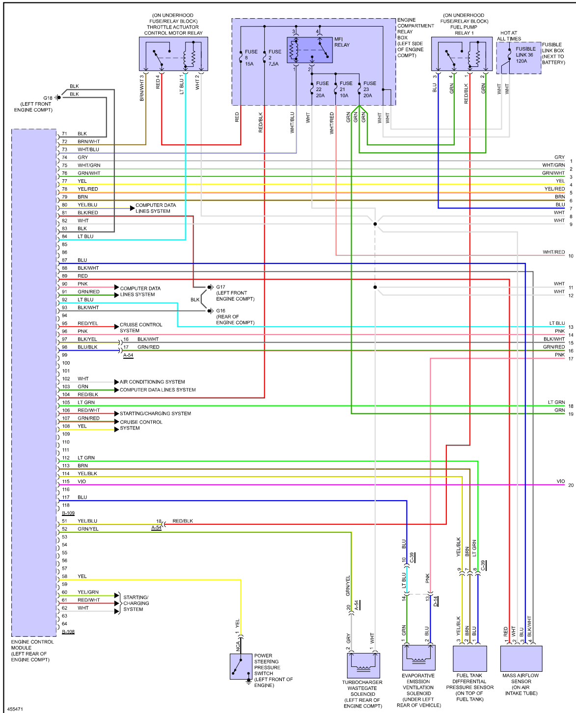
Fig 5: 2.0L Turbo, Engine Performance Circuit, Except Evolution (1 of 4)
