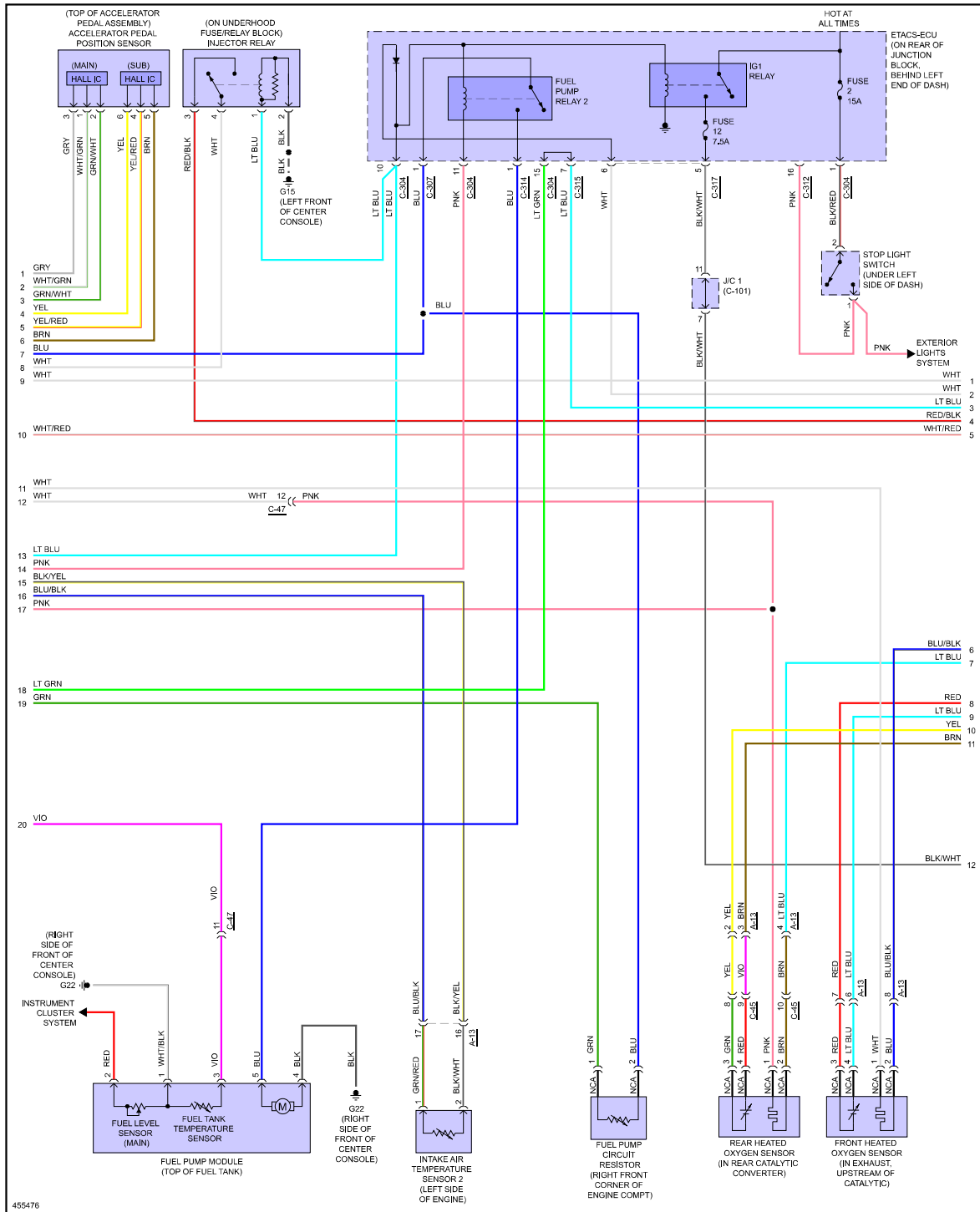
Fig 2: 2.0L Turbo, Engine Performance Circuit, Evolution (2 of 4)
