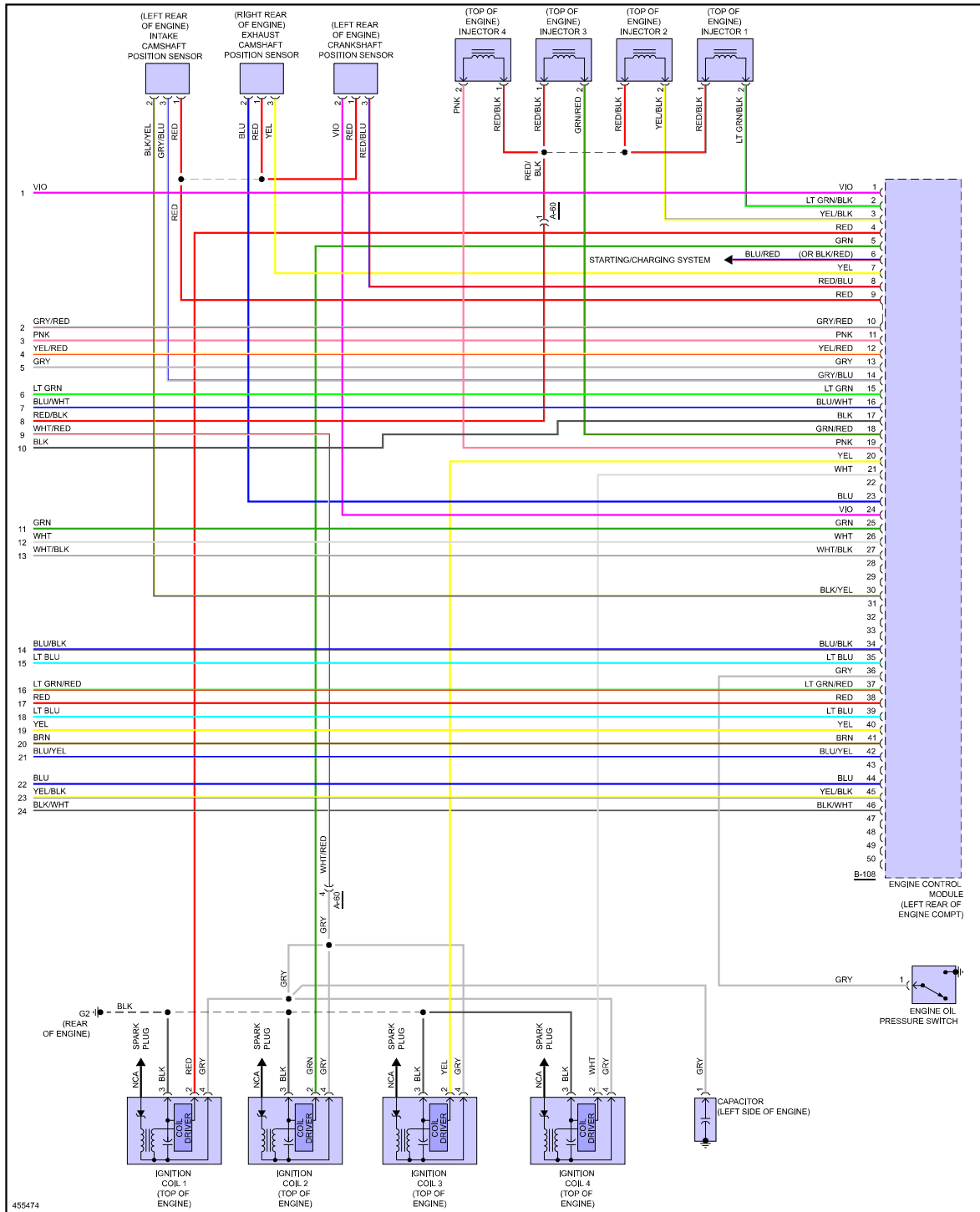
Fig 8: 2.0L Turbo, Engine Performance Circuit, Except Evolution (4 of 4)
