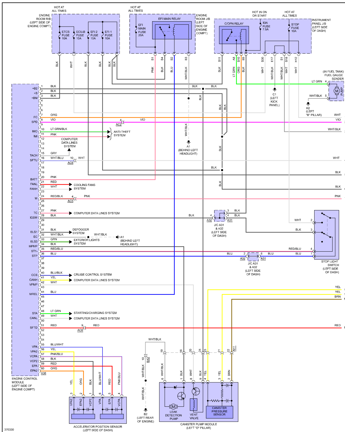
Fig 1: 2.4L, Engine Performance Circuit (1 of 4)
