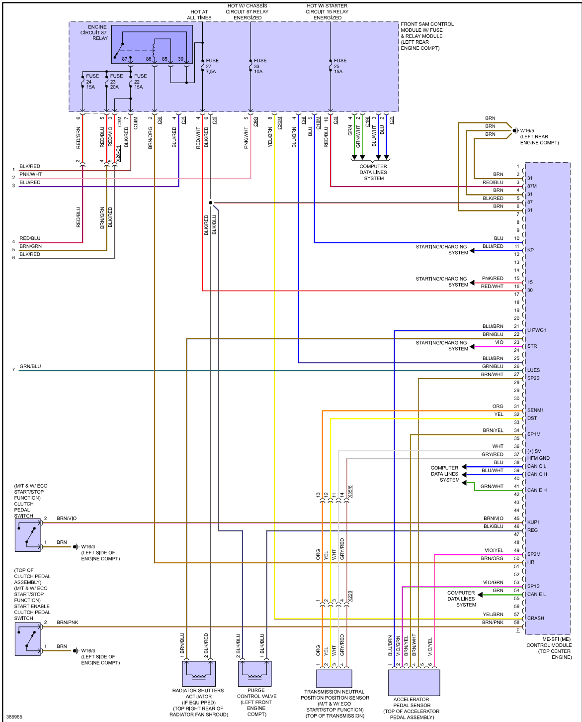
Fig 4: 1.8L Turbo, Engine Performance Circuit (4 of 4)
