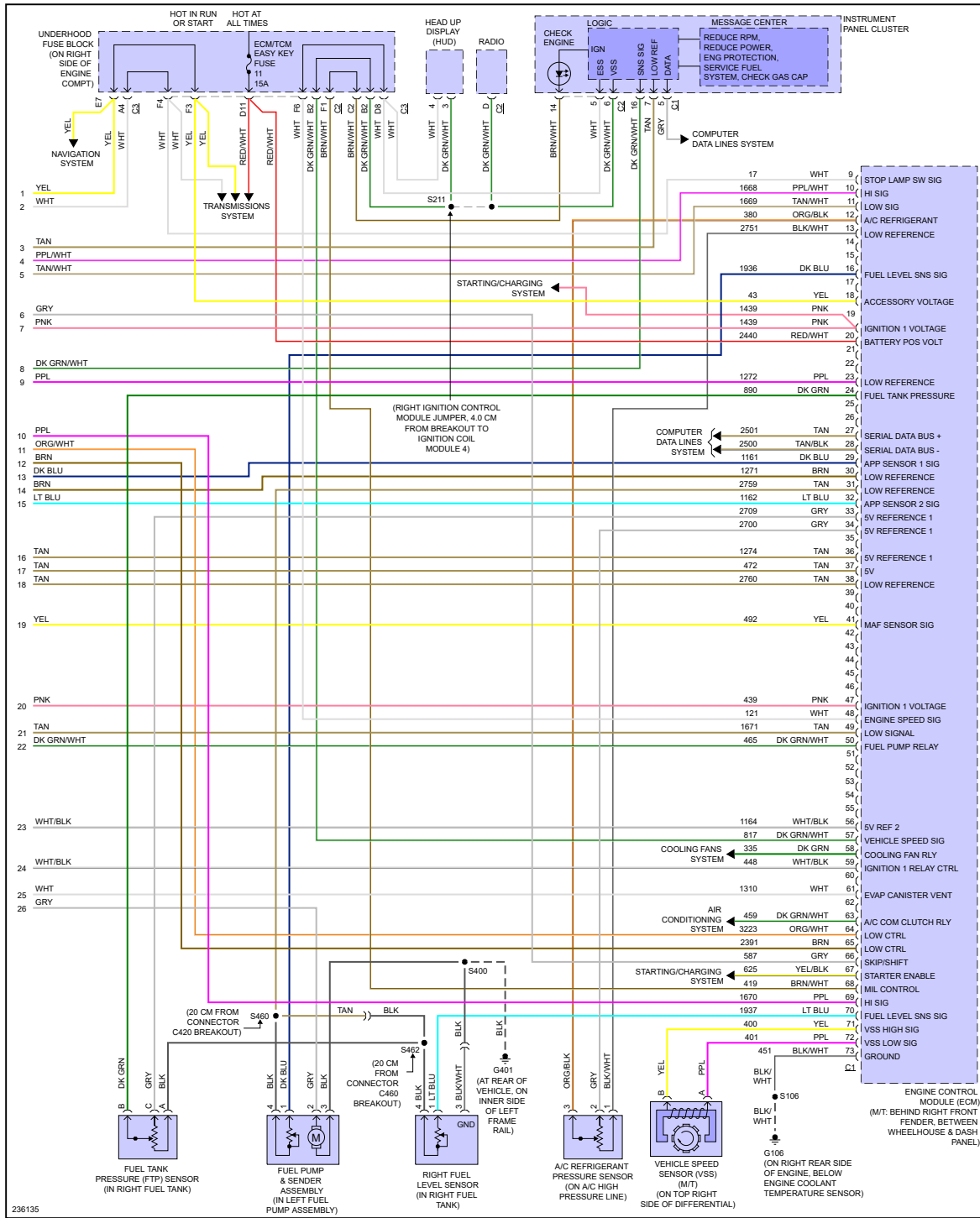
Fig 4: 6.0L VIN U, Engine Performance Circuit (4 of 4)
