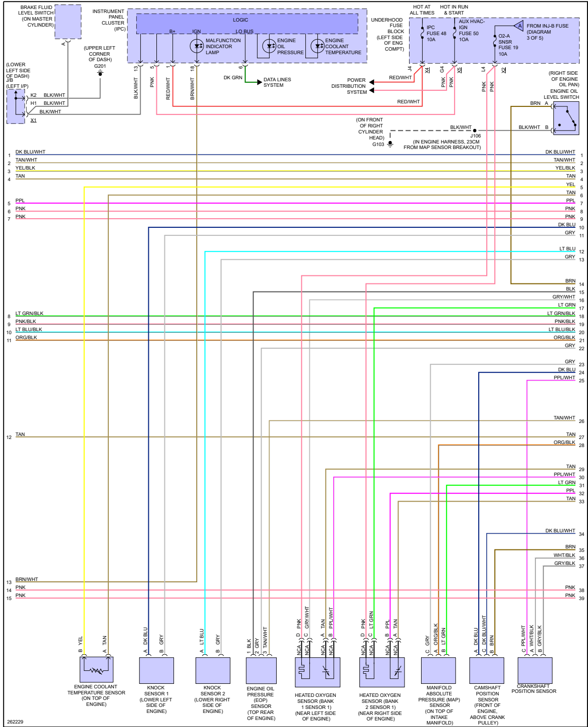
Fig 4: 5.3L VIN M, Engine Performance Circuit (4 of 5)
