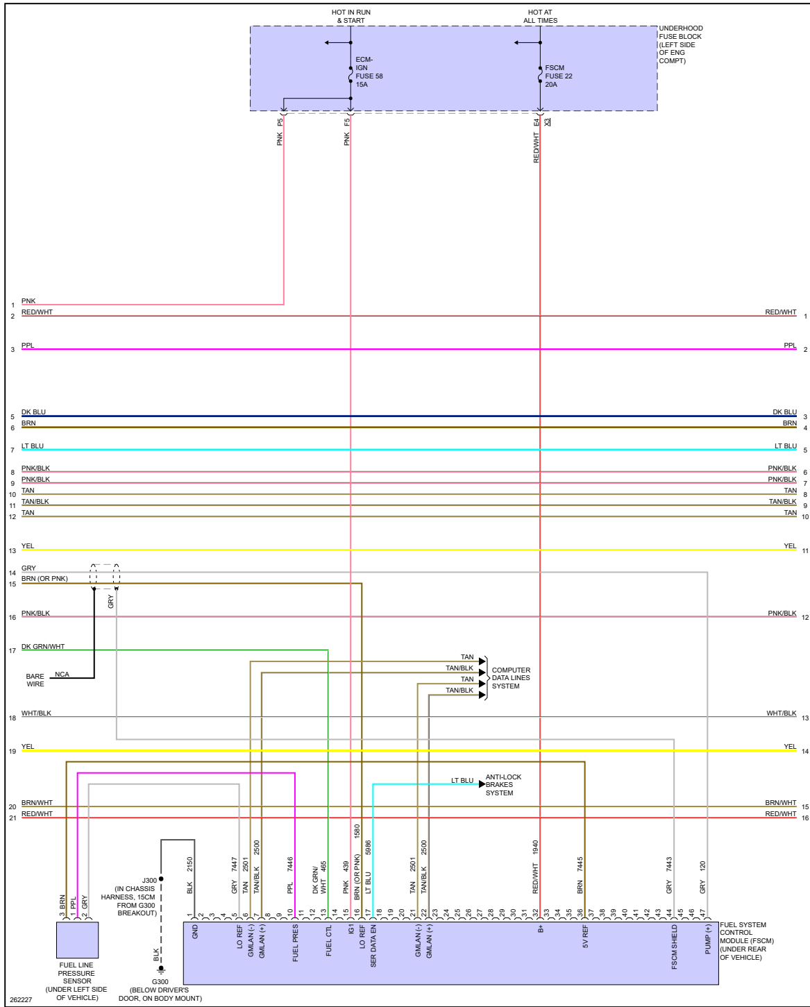
Fig 2: 5.3L VIN M, Engine Performance Circuit (2 of 5)
