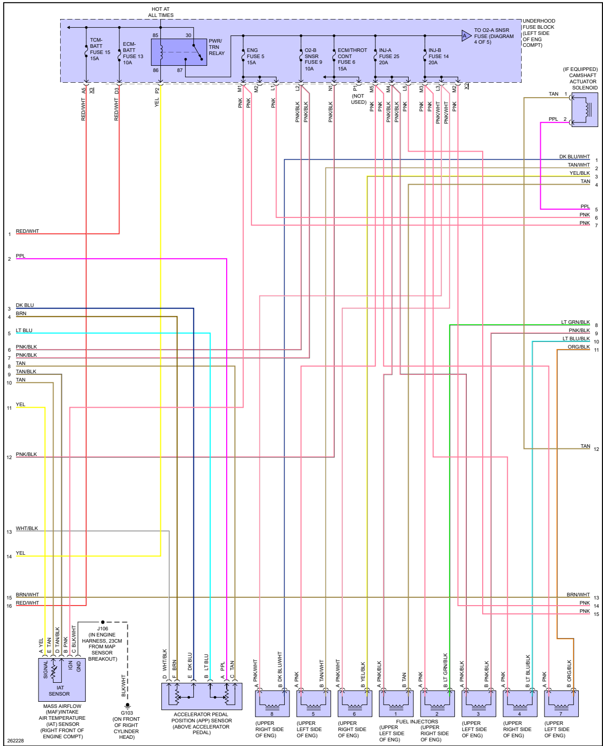
Fig 3: 5.3L VIN M, Engine Performance Circuit (3 of 5)
