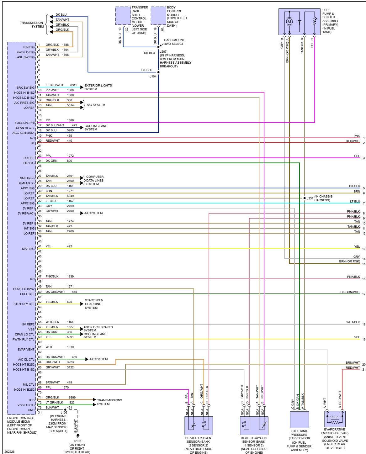
Fig 1: 5.3L VIN M, Engine Performance Circuit (1 of 5)
