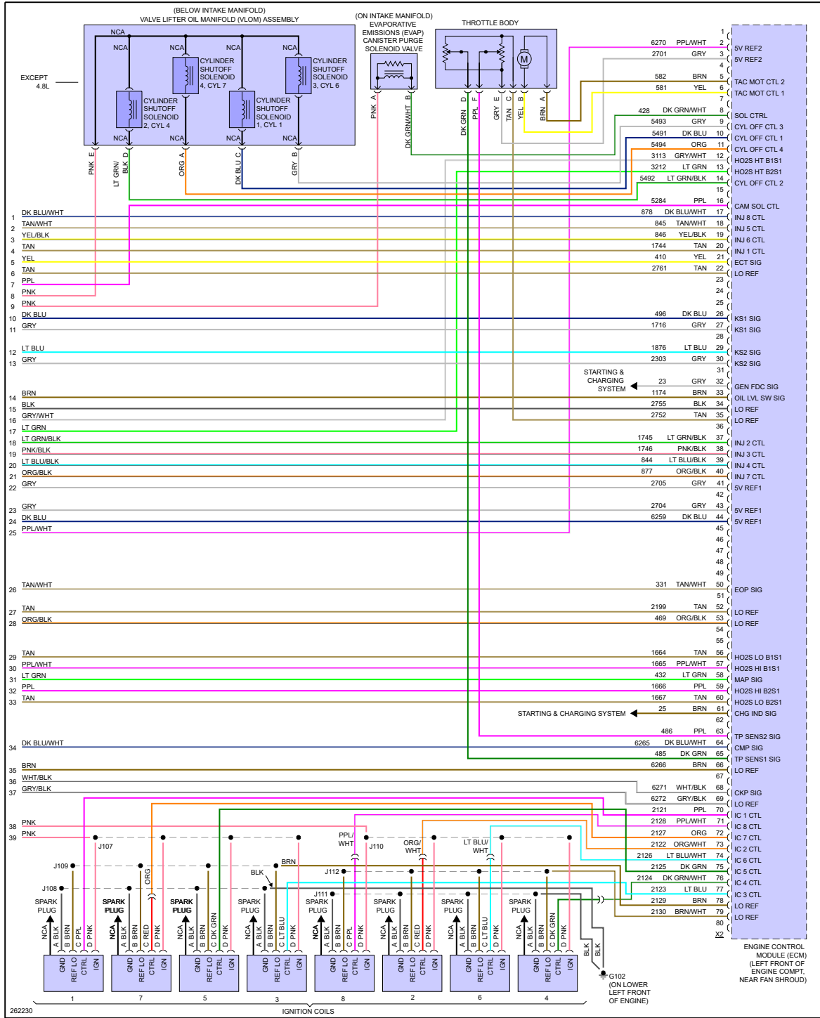
Fig 5: 5.3L VIN M, Engine Performance Circuit (5 of 5)
