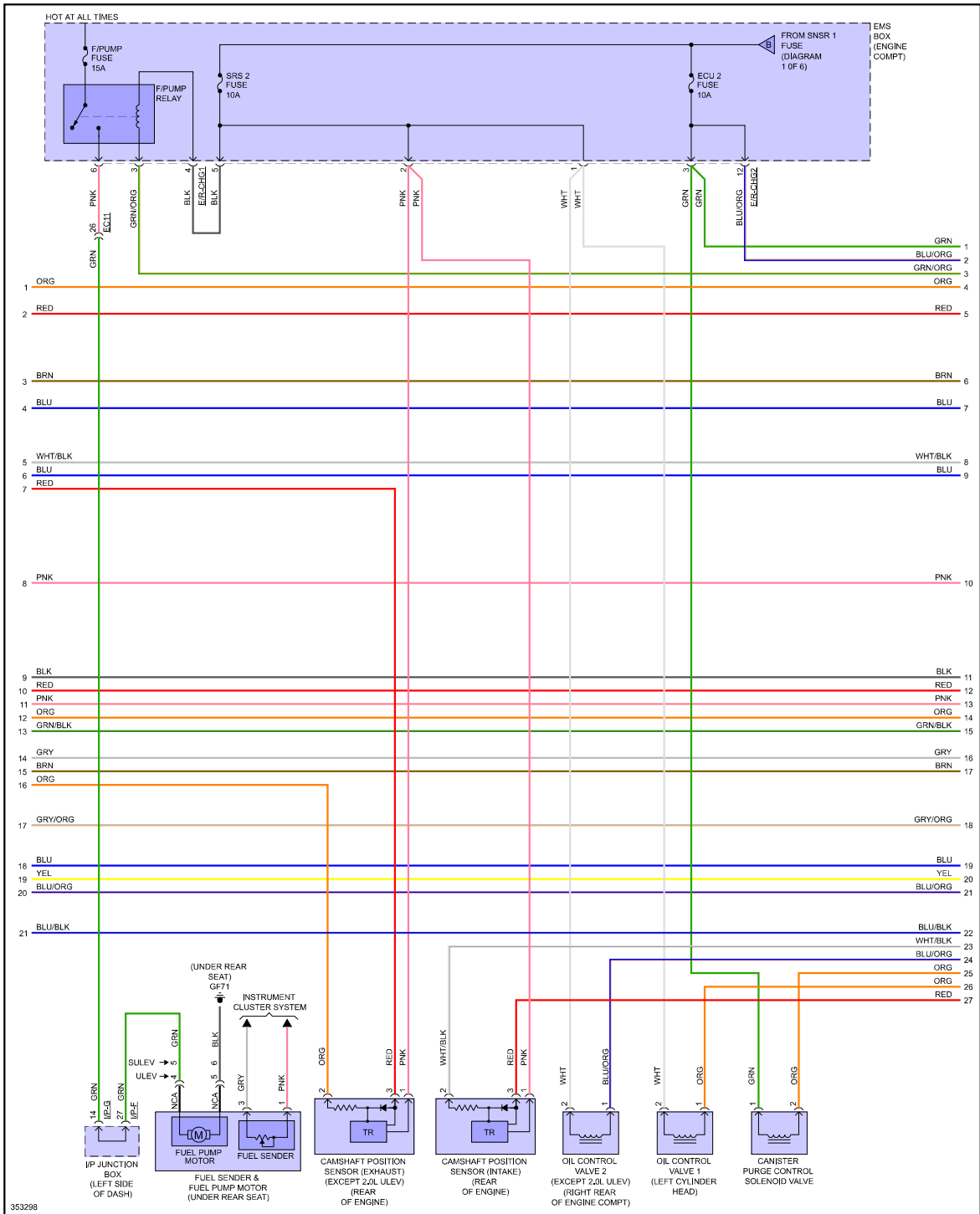
Fig 2: 2.4L, Engine Performance Circuit (2 of 6)
