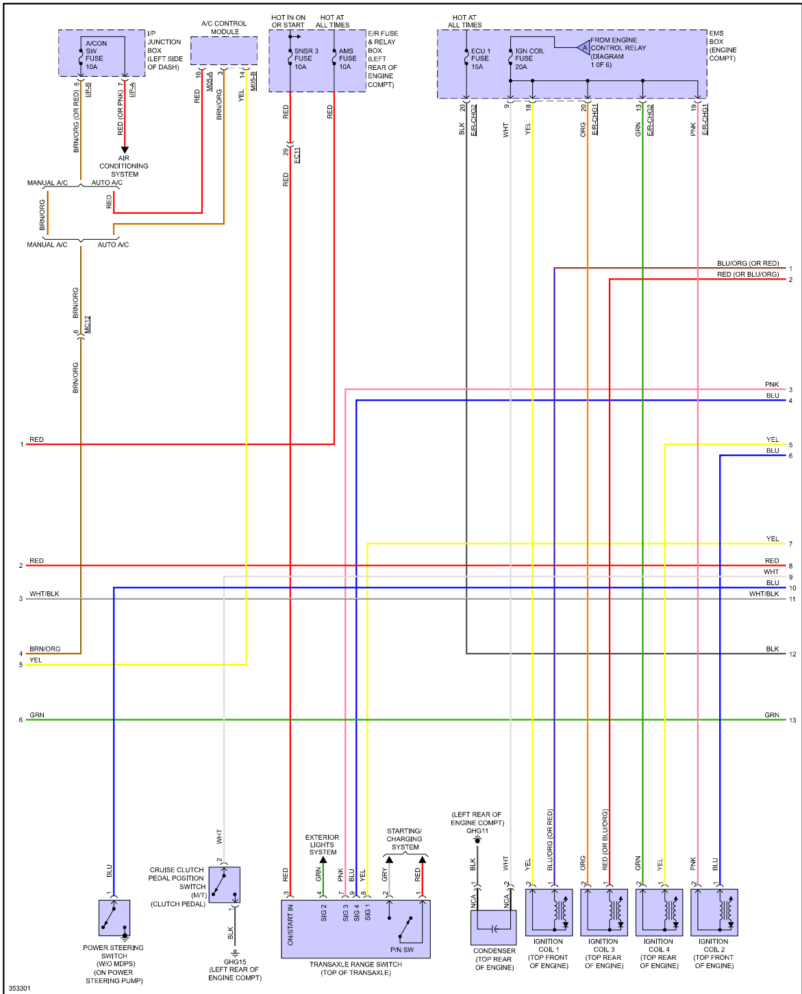
Fig 5: 2.4L, Engine Performance Circuit (5 of 6)
