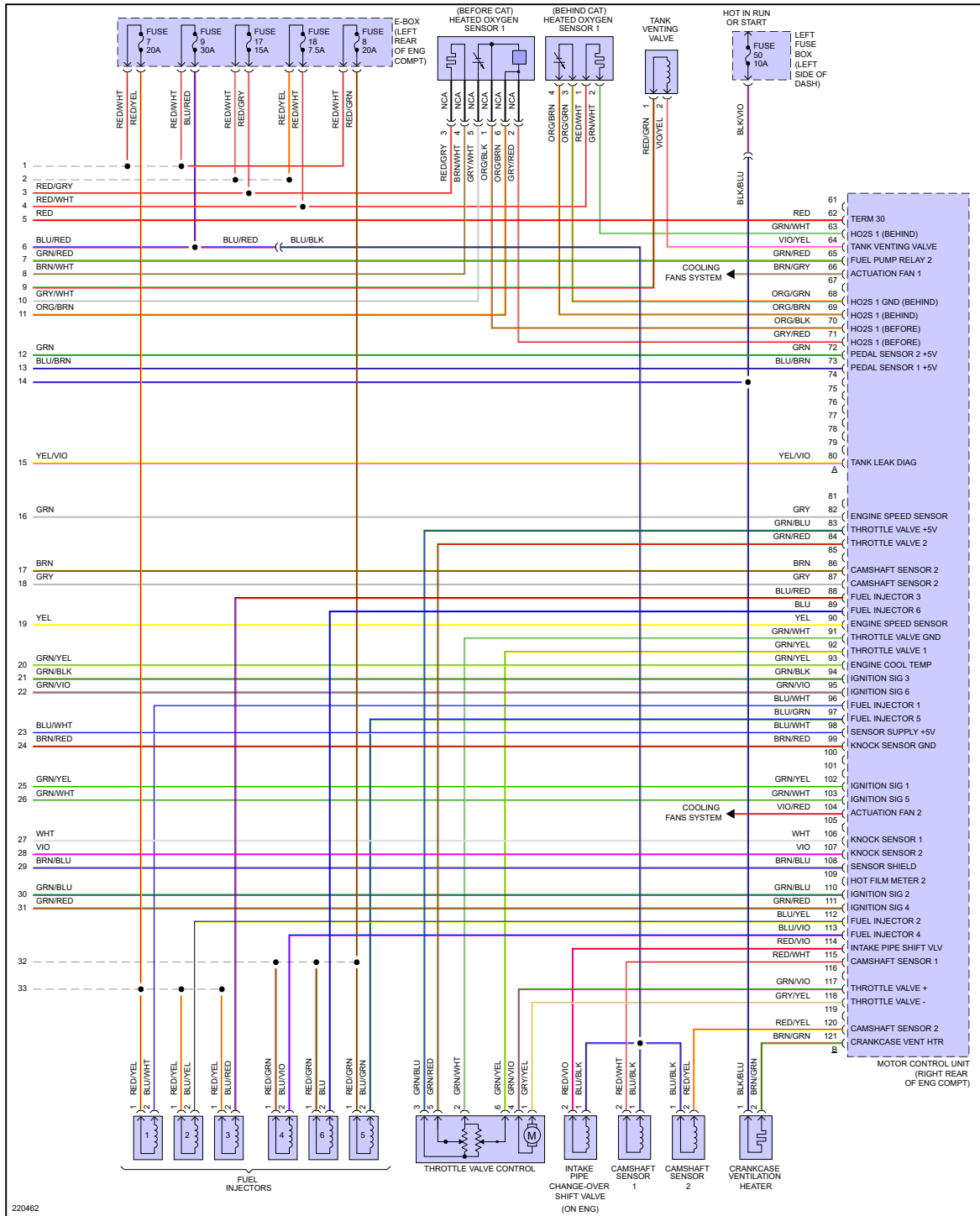
Fig 4: 3.2L, Engine Performance Circuit (4 of 4)
