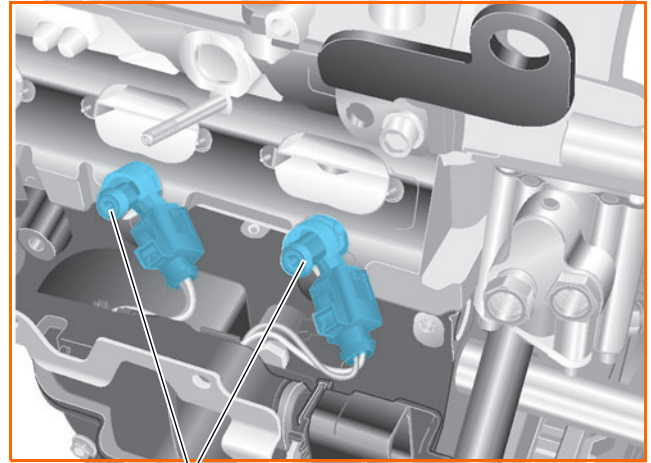
High-pressure injectors
