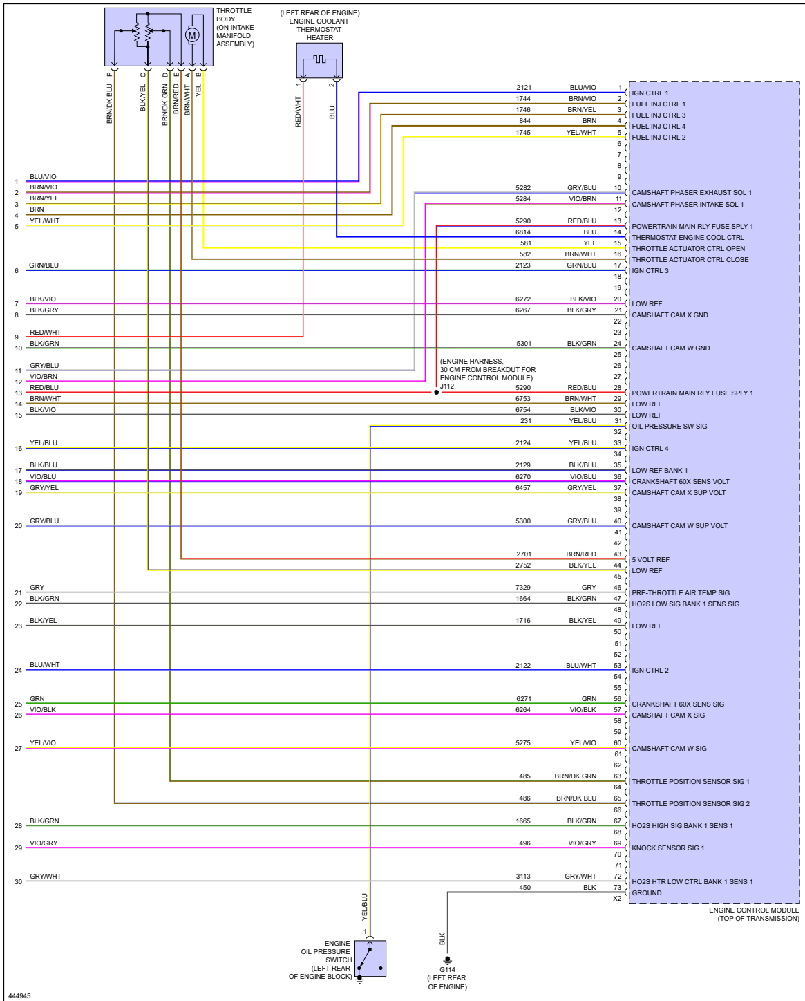
Fig 6: 1.4L VIN B, Engine Performance Circuit (6 of 6)
