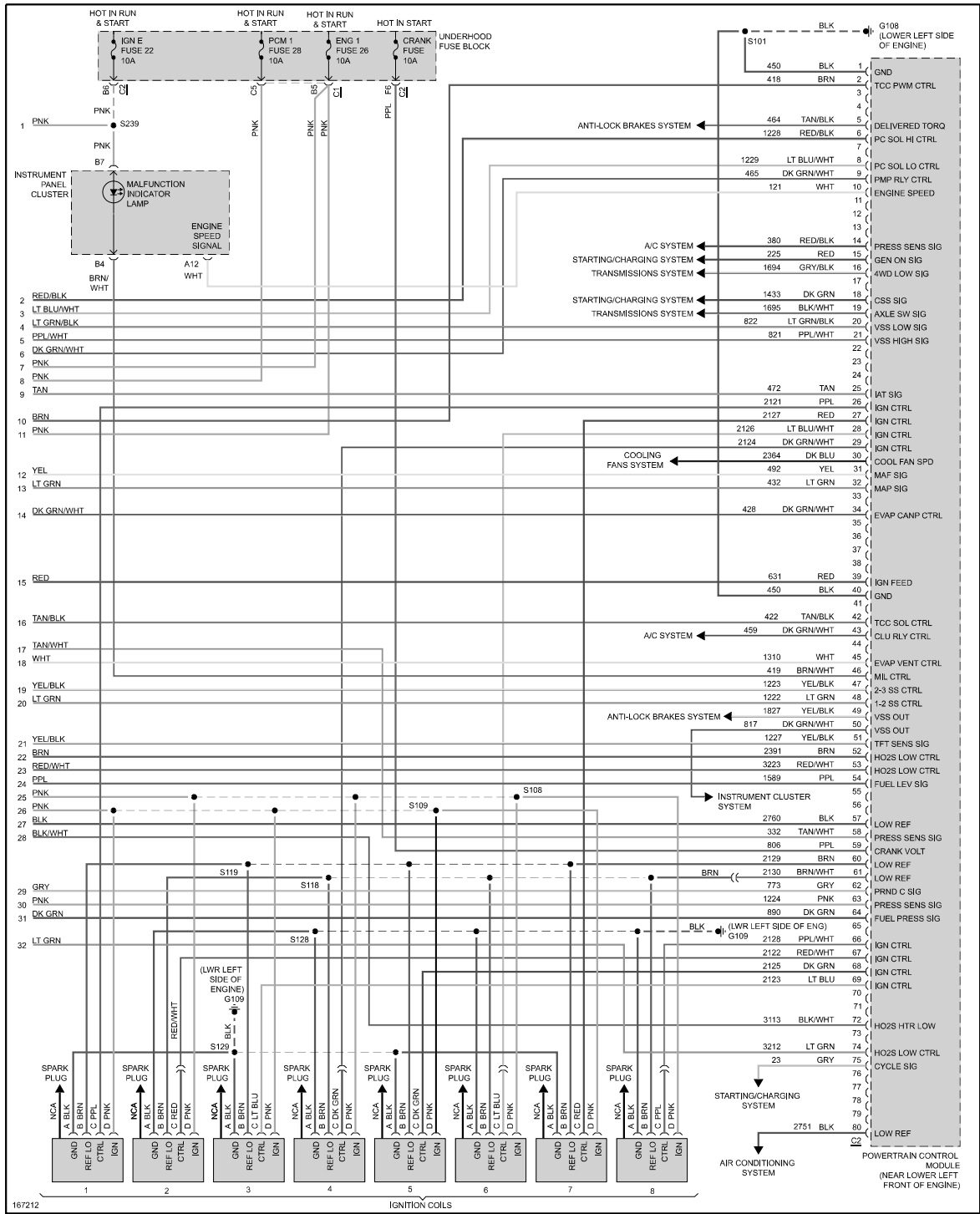
Fig 5: 5.3L VIN P, Engine Performance Circuit (5 of 5)
