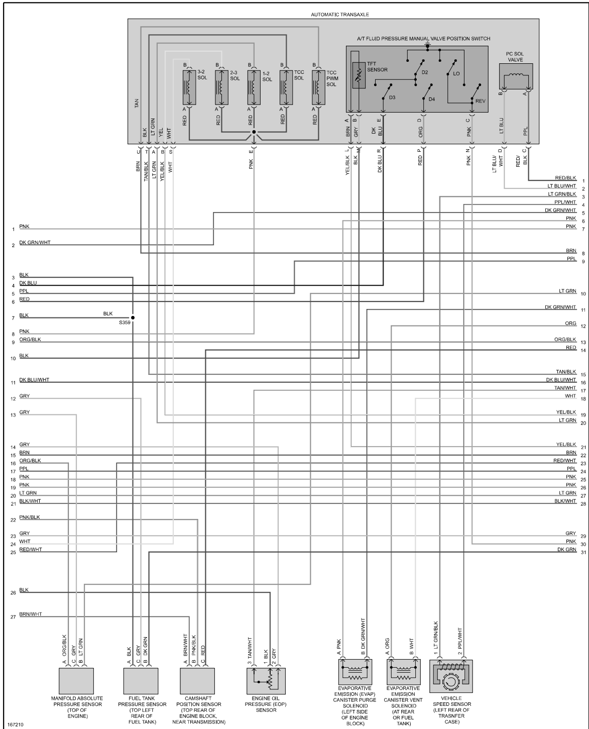
Fig 3: 5.3L VIN P, Engine Performance Circuit (3 of 5)
