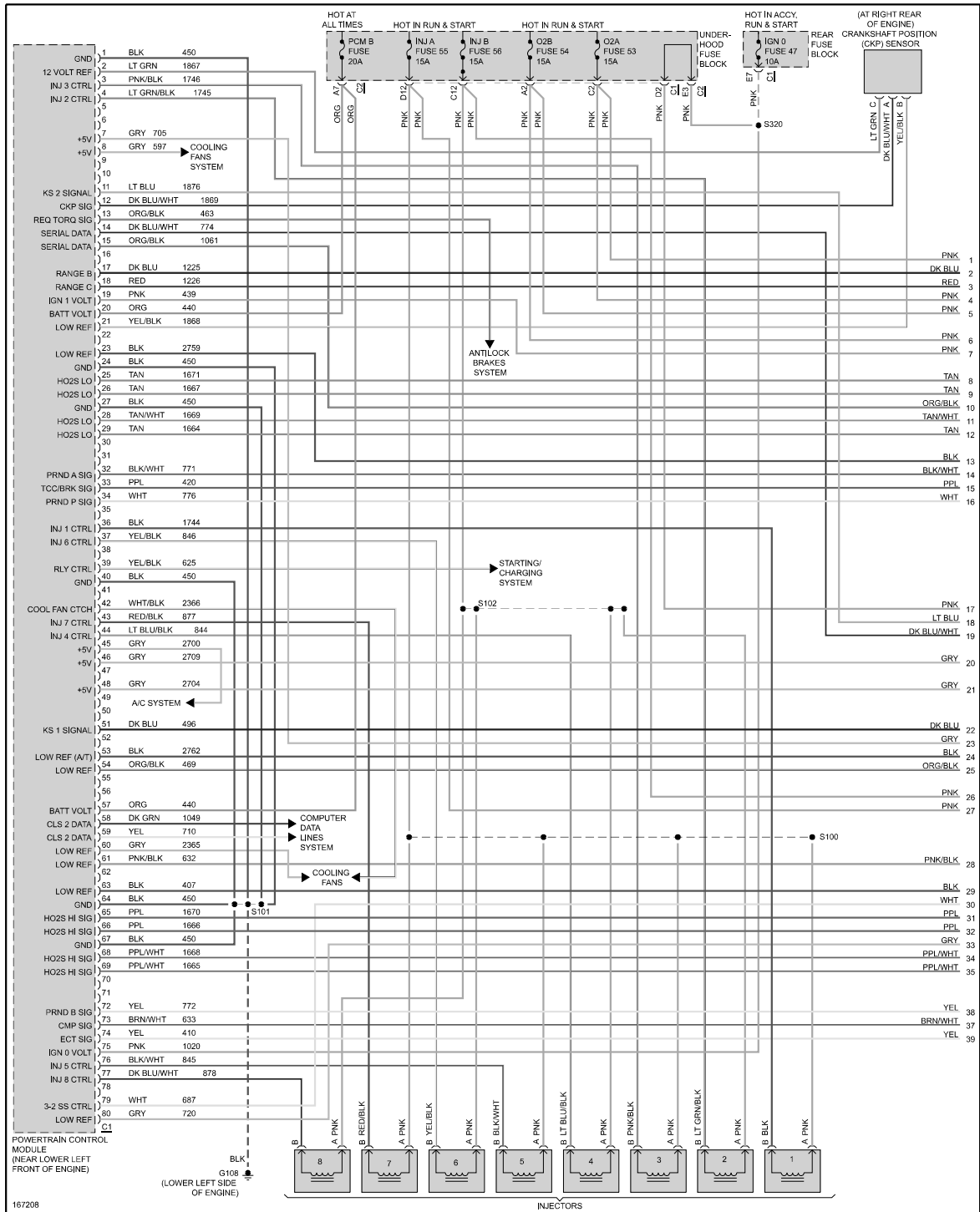
Fig 1: 5.3L VIN P, Engine Performance Circuit (1 of 5)
