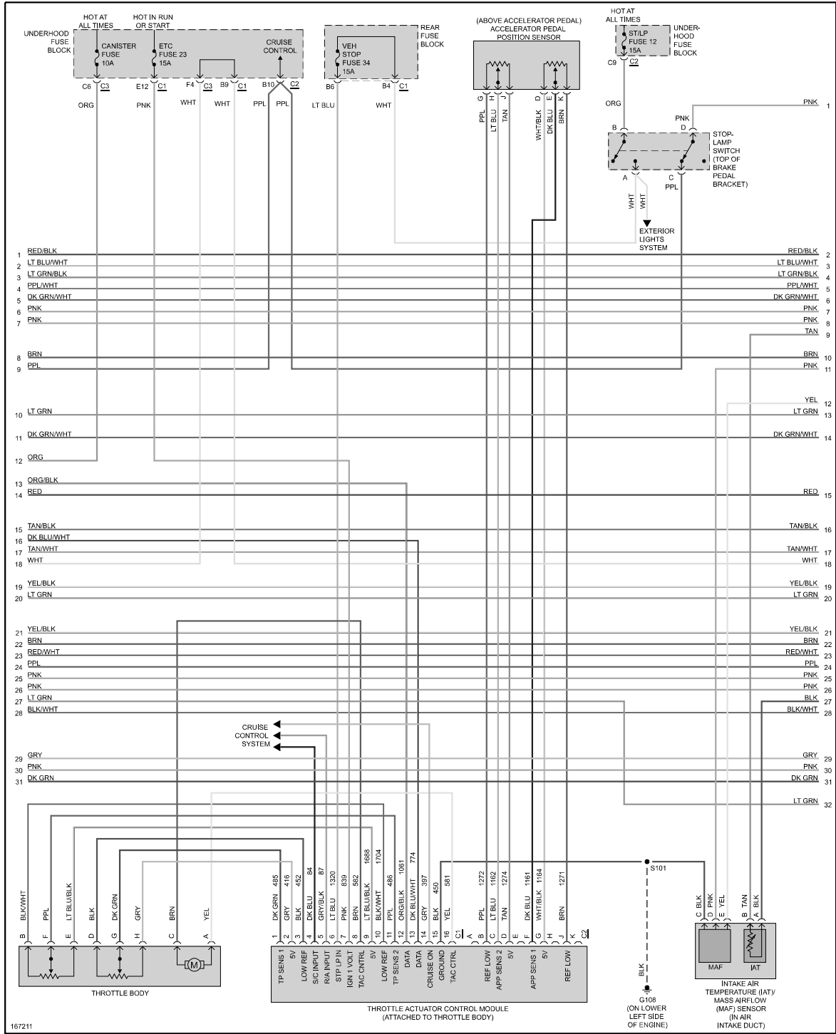
Fig 4: 5.3L VIN P, Engine Performance Circuit (4 of 5)
