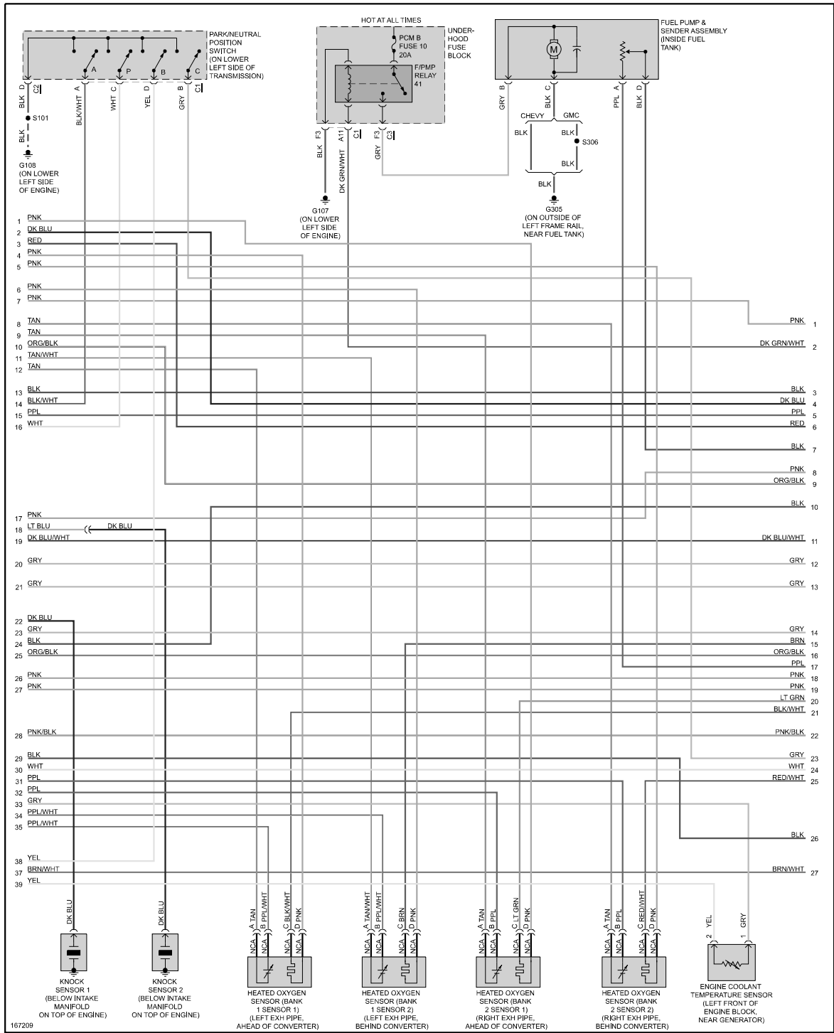
Fig 2: 5.3L VIN P, Engine Performance Circuit (2 of 5)
