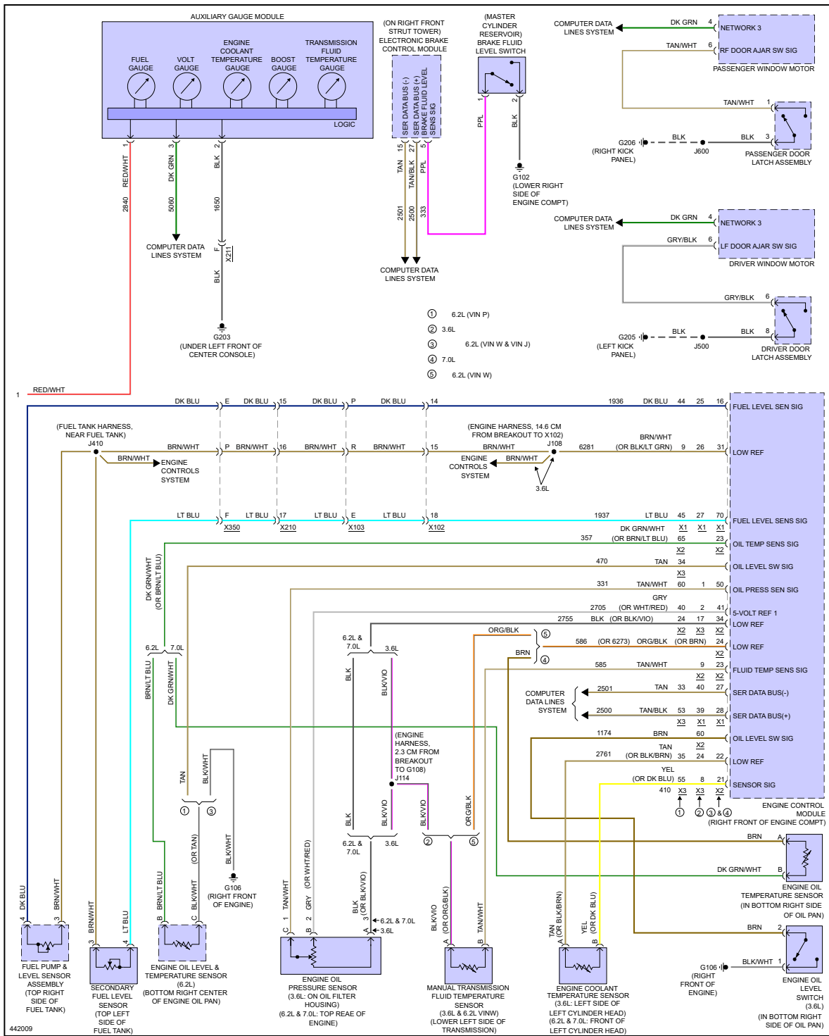
Fig 3: Instrument Cluster Circuit (2 of 2)
