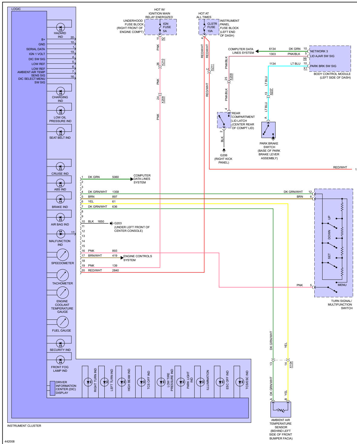
Fig 2: Instrument Cluster Circuit (1 of 2)
