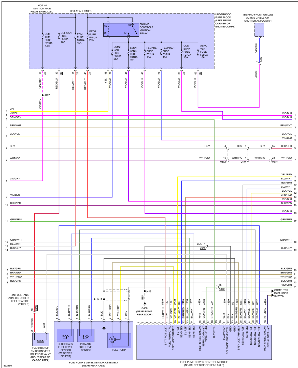
Fig 2: 1.3L VIN L, Engine Performance Circuit (2 of 7)
