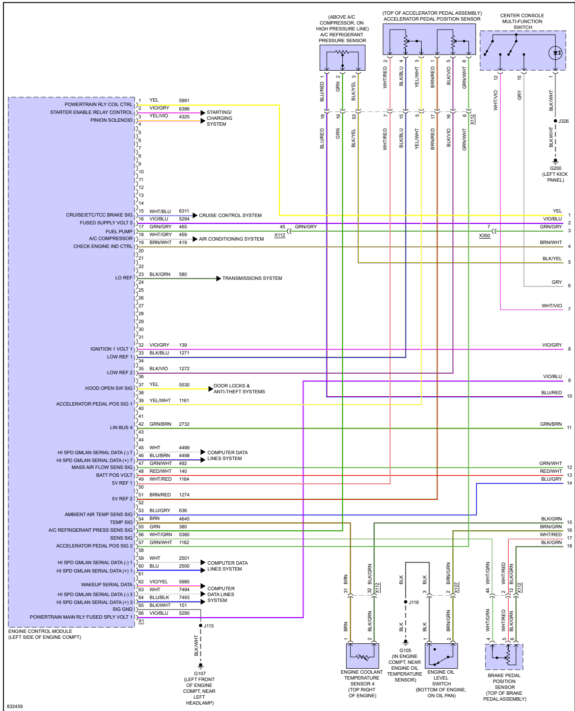
Fig 1: 1.3L VIN L, Engine Performance Circuit (1 of 7)
