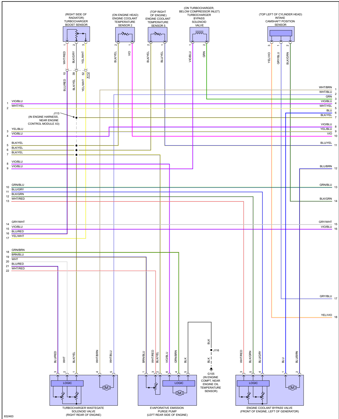
Fig 5: 1.3L VIN L, Engine Performance Circuit (5 of 7)
