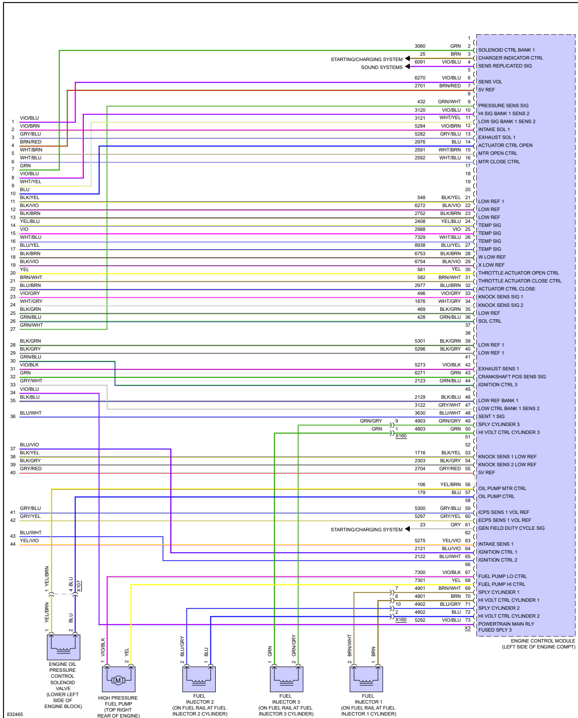
Fig 7: 1.3L VIN L, Engine Performance Circuit (7 of 7)
