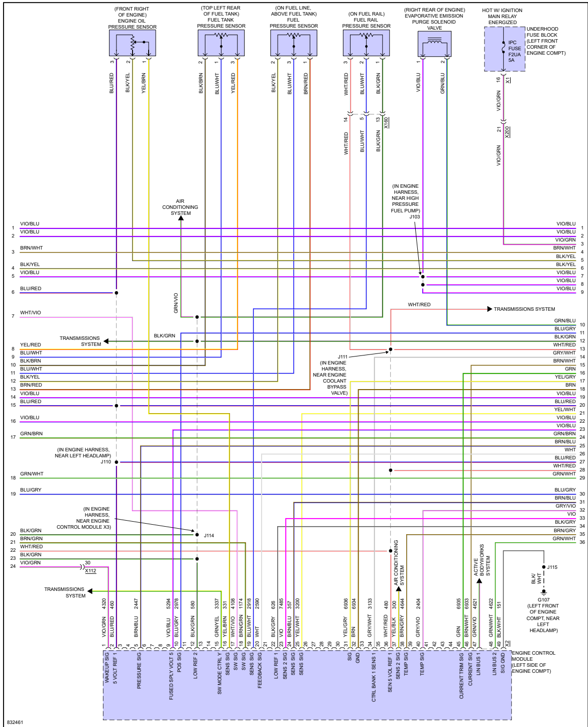
Fig 3: 1.3L VIN L, Engine Performance Circuit (3 of 7)
