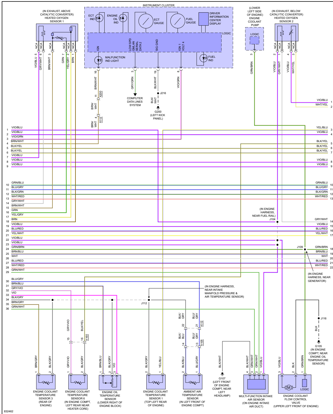
Fig 4: 1.3L VIN L, Engine Performance Circuit (4 of 7)
