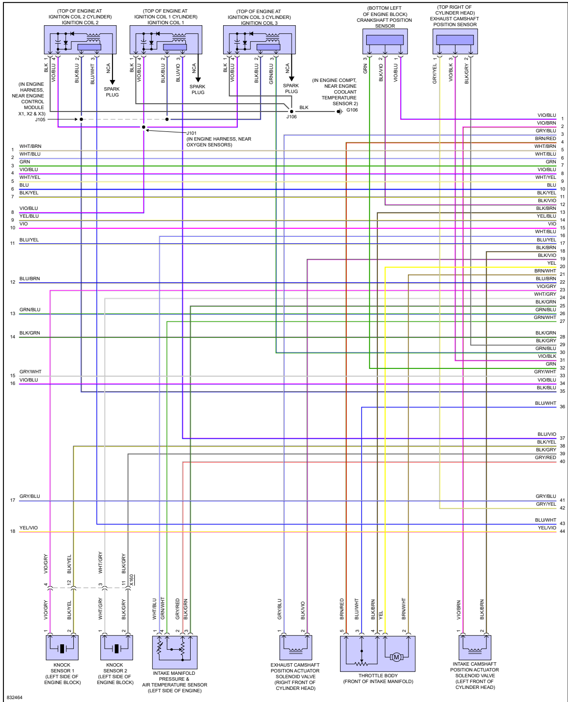
Fig 6: 1.3L VIN L, Engine Performance Circuit (6 of 7)
