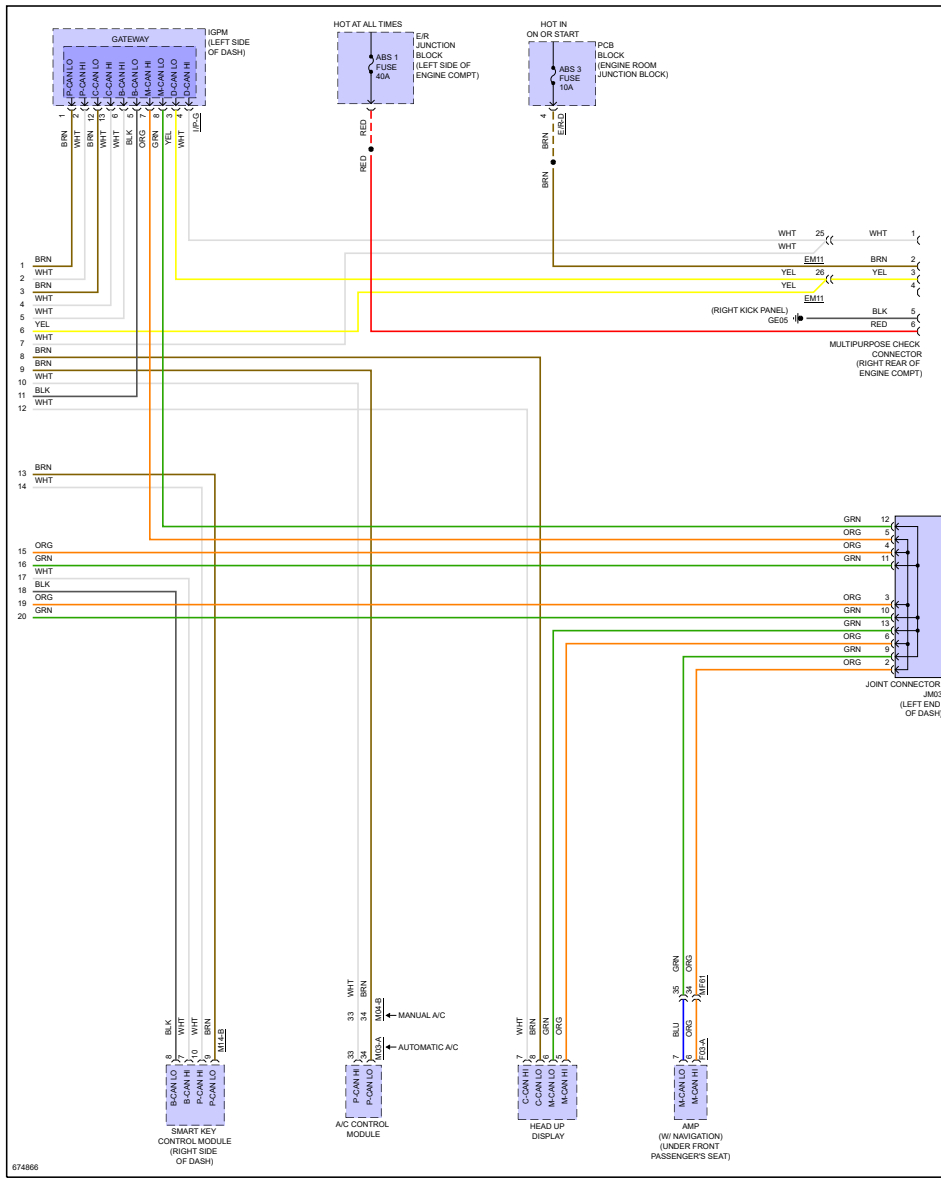
Fig 4: Computer Data Lines Circuit (4 of 4)
