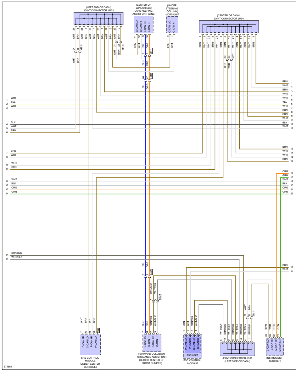
Fig 2: Computer Data Lines Circuit (2 of 4)
