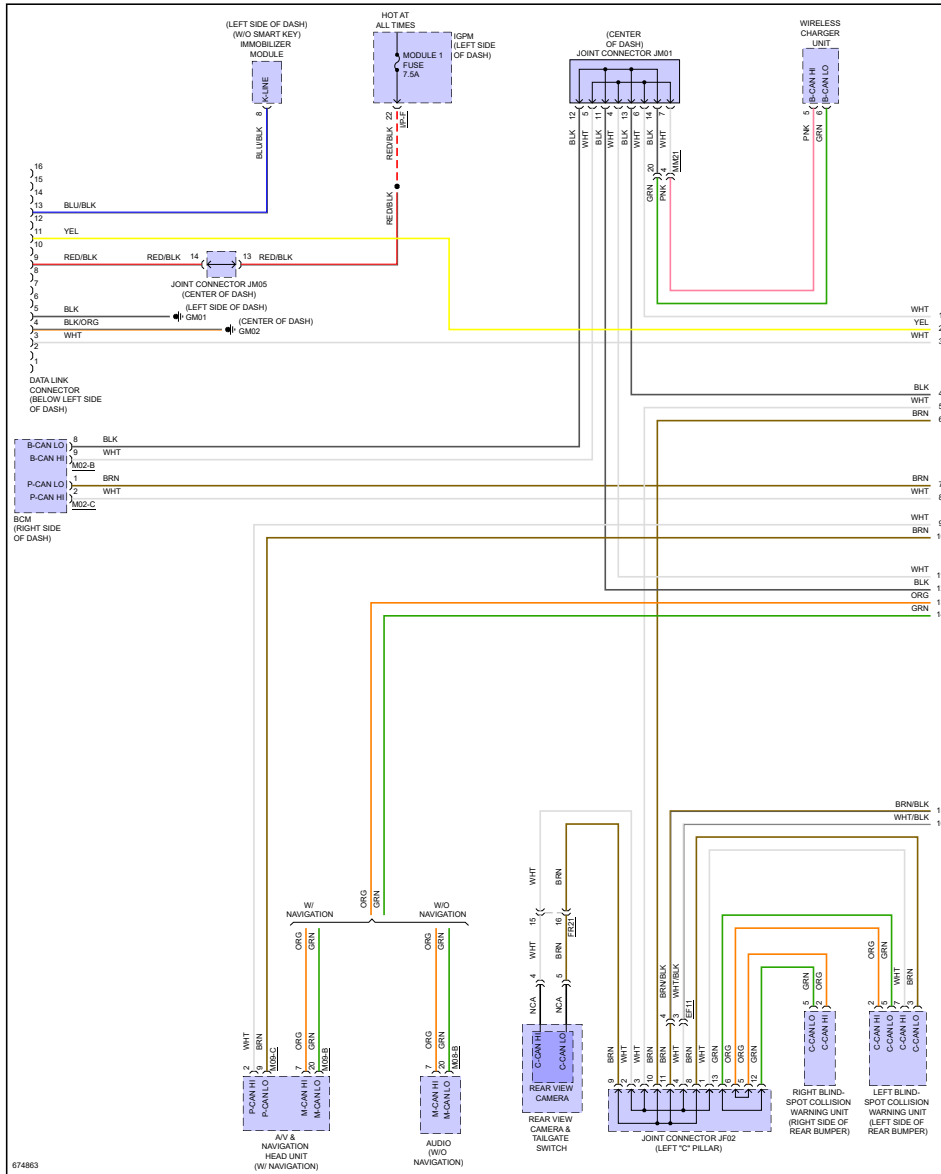
Fig 1: Computer Data Lines Circuit (1 of 4)
