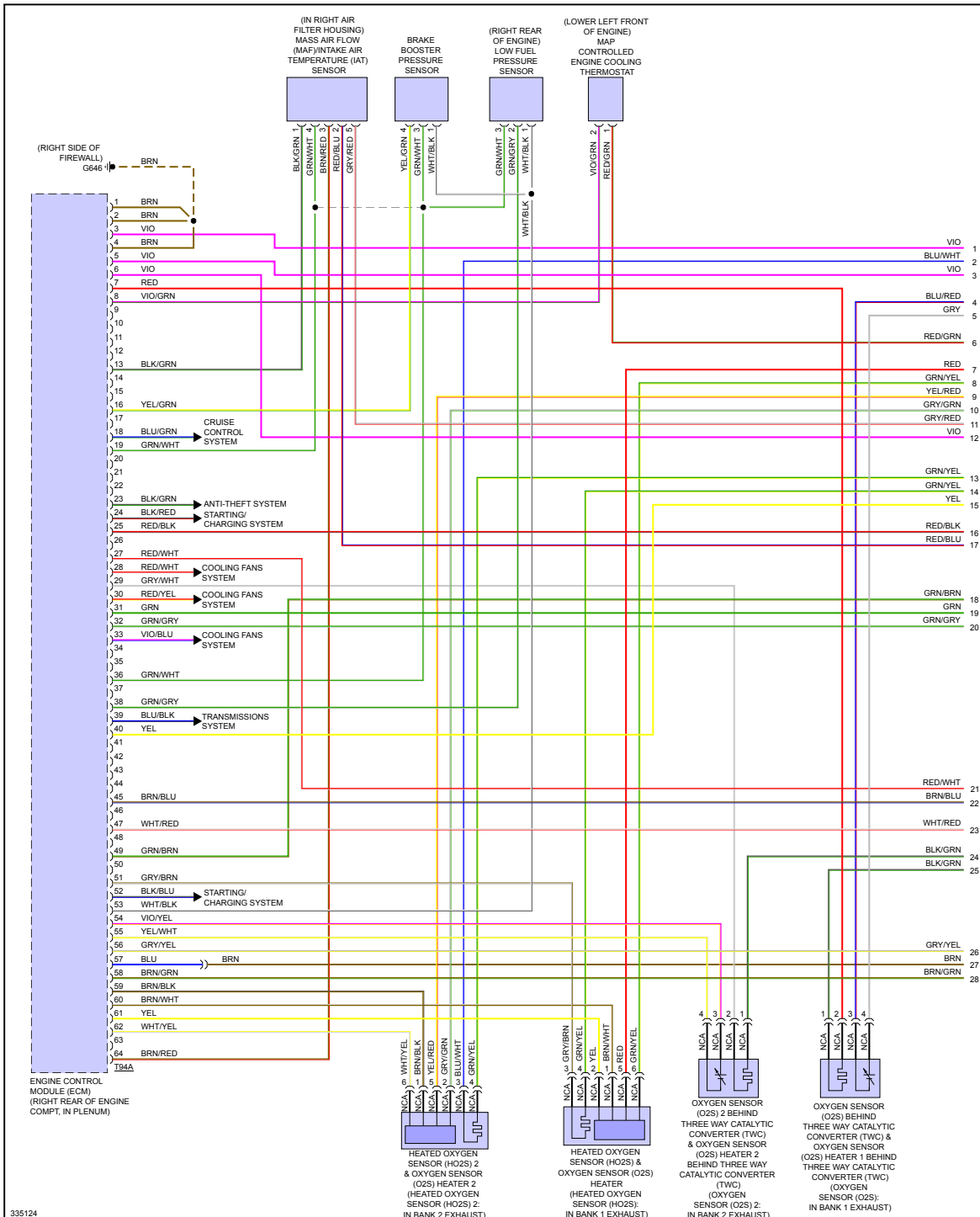
Fig 1: 5.2L, Engine Performance Circuit (1 of 8)
