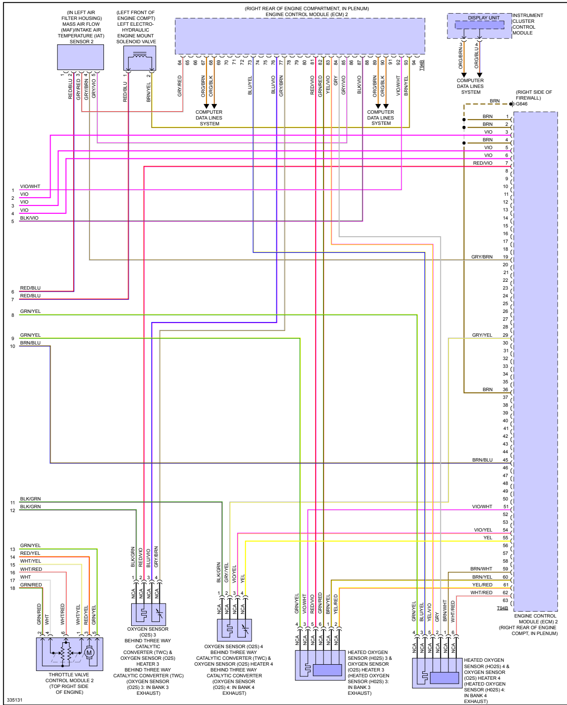
Fig 8: 5.2L, Engine Performance Circuit (8 of 8)
