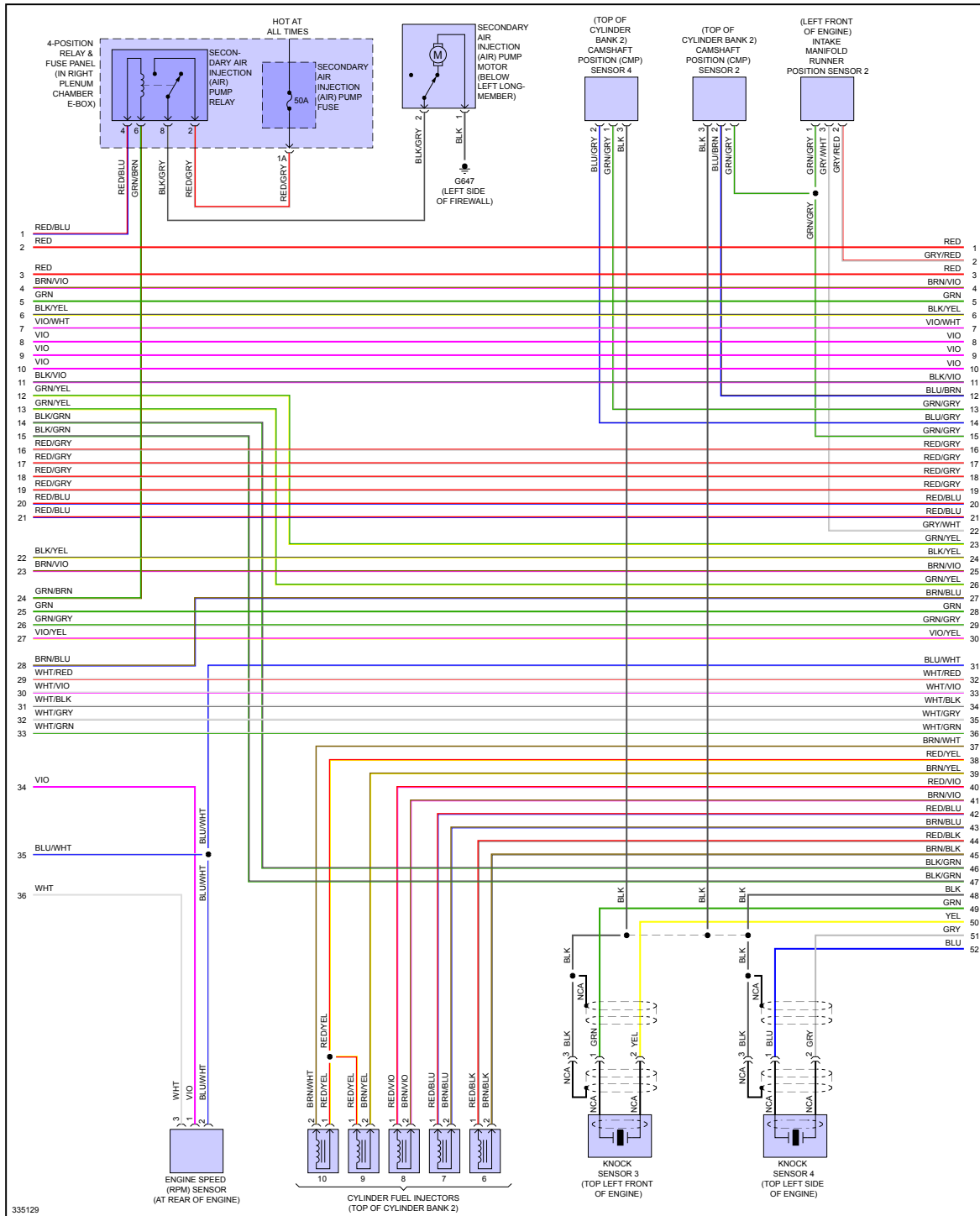
Fig 6: 5.2L, Engine Performance Circuit (6 of 8)
