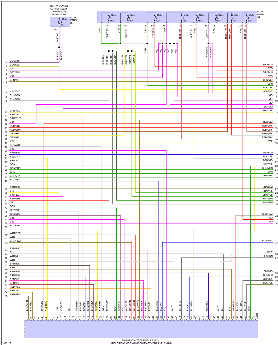
Fig 4: 5.2L, Engine Performance Circuit (4 of 8)
