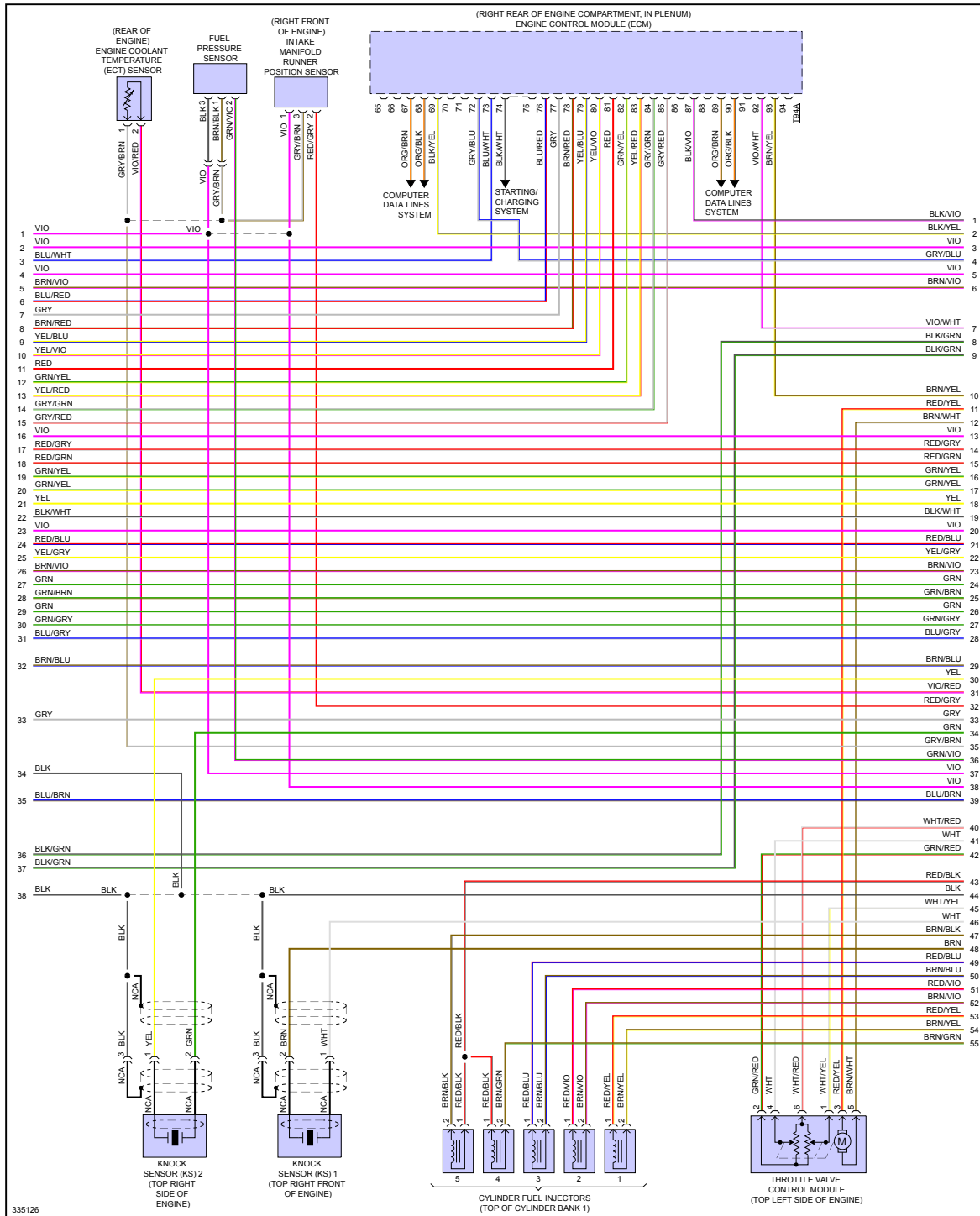
Fig 3: 5.2L, Engine Performance Circuit (3 of 8)
