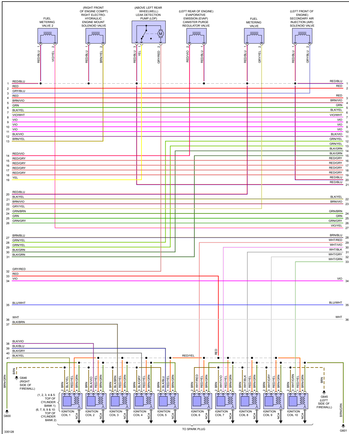
Fig 5: 5.2L, Engine Performance Circuit (5 of 8)
