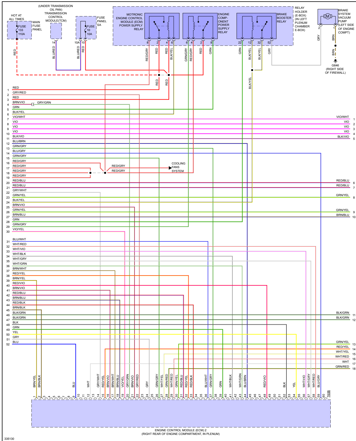
Fig 7: 5.2L, Engine Performance Circuit (7 of 8)
