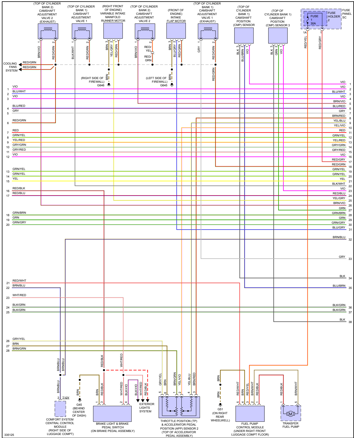
Fig 2: 5.2L, Engine Performance Circuit (2 of 8)
