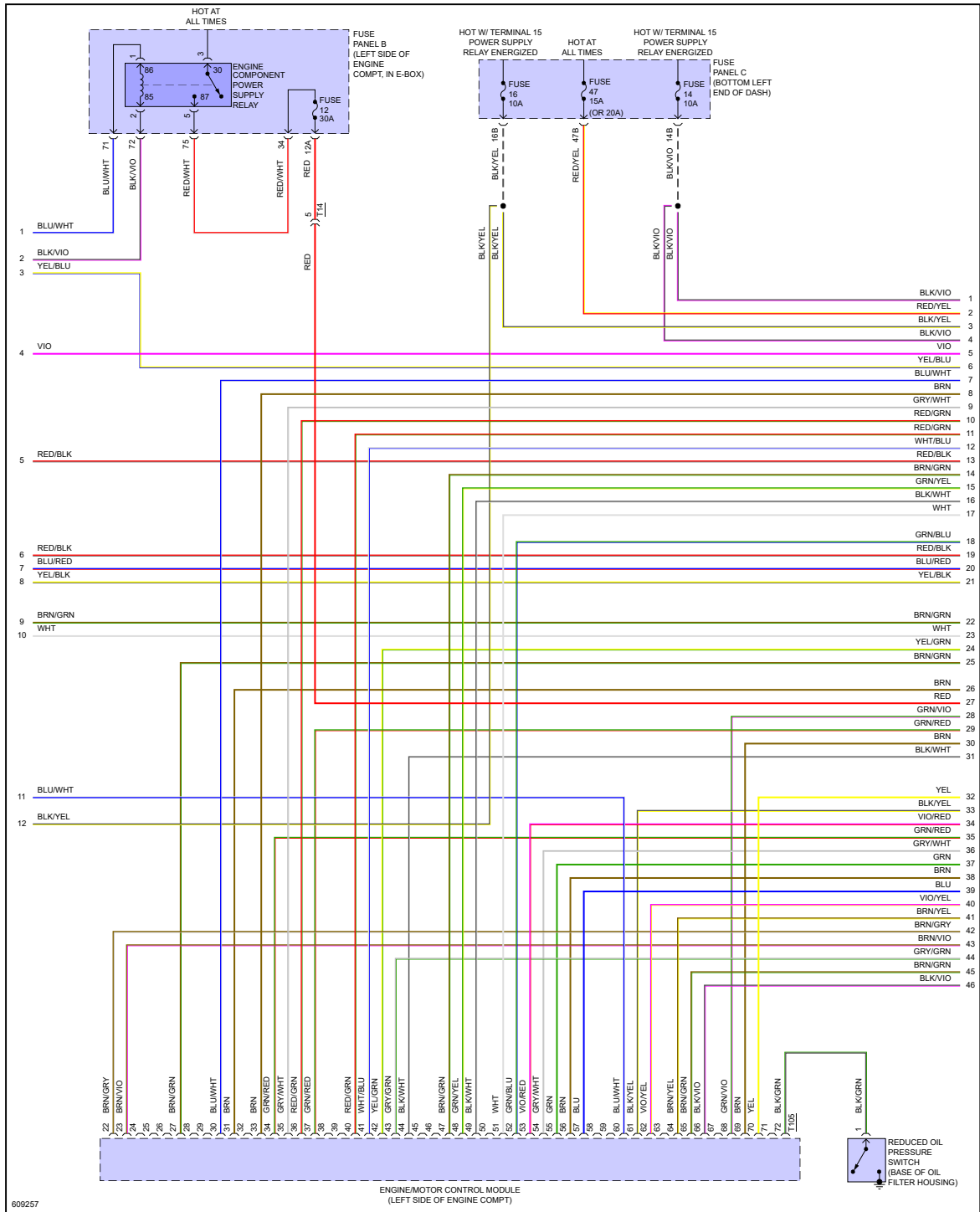
Fig 3: 2.0L Turbo, Engine Controls Circuit (3 of 6)
