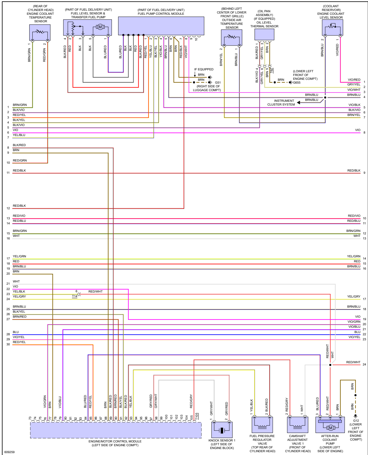
Fig 5: 2.0L Turbo, Engine Controls Circuit (5 of 6)
