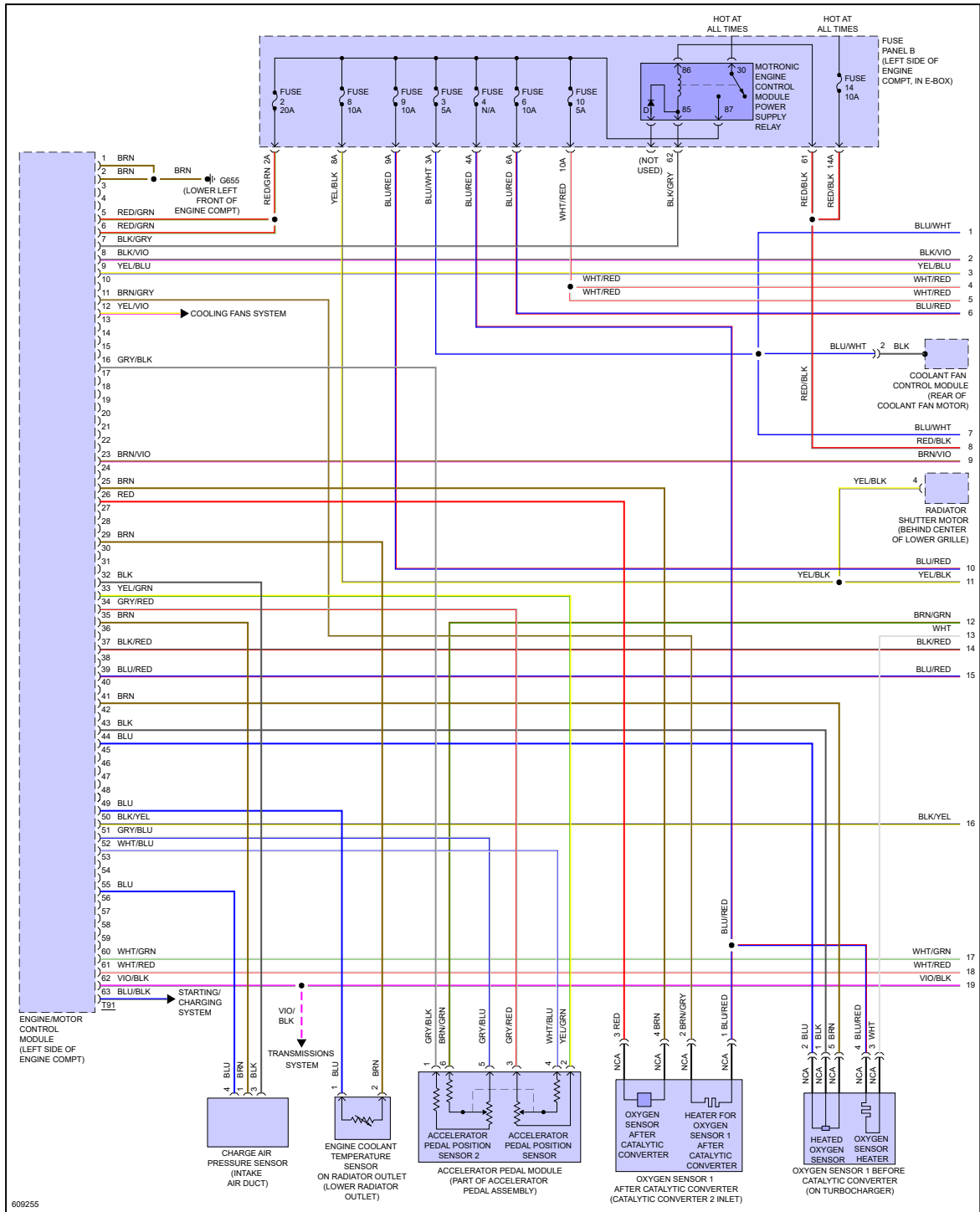
Fig 1: 2.0L Turbo, Engine Controls Circuit (1 of 6)
