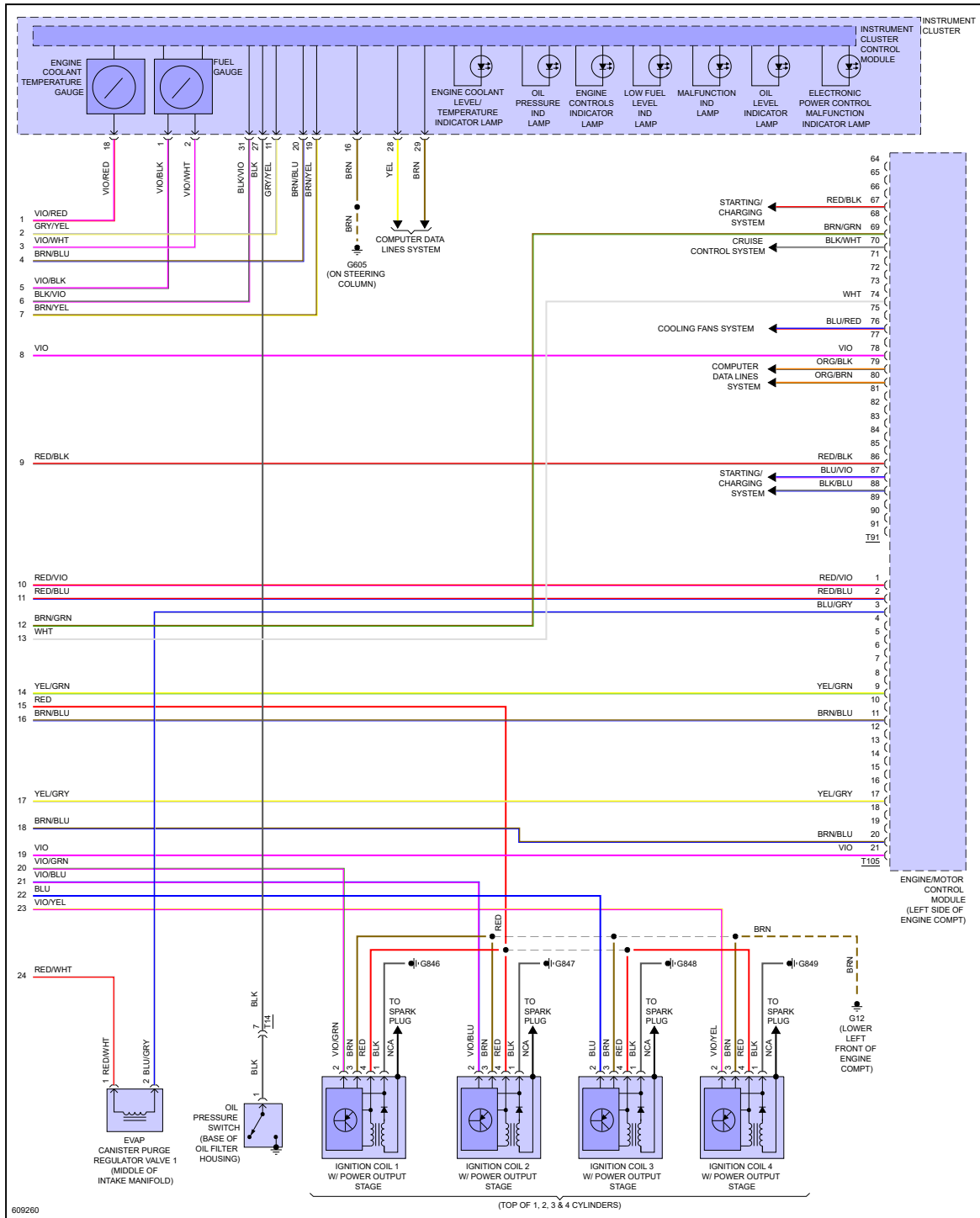
Fig 6: 2.0L Turbo, Engine Controls Circuit (6 of 6)
