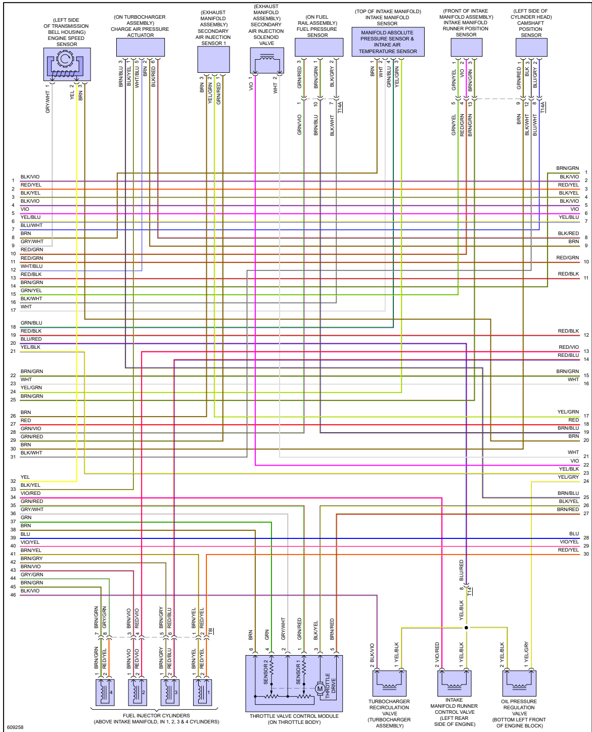
Fig 4: 2.0L Turbo, Engine Controls Circuit (4 of 6)
