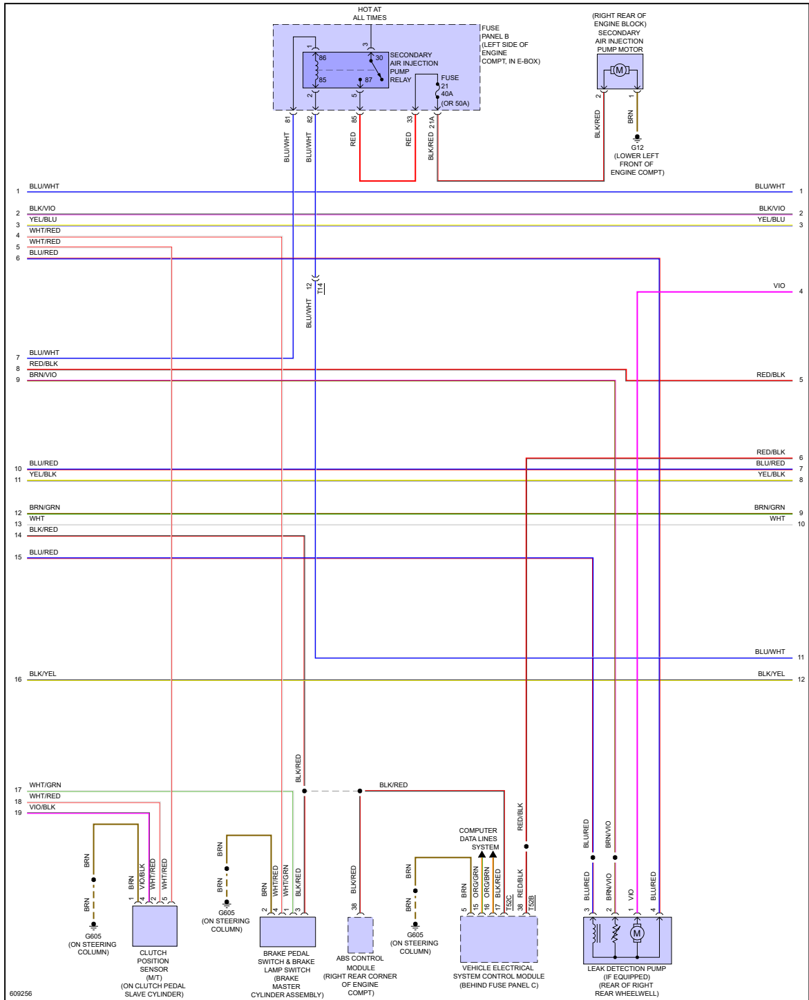
Fig 2: 2.0L Turbo, Engine Controls Circuit (2 of 6)
