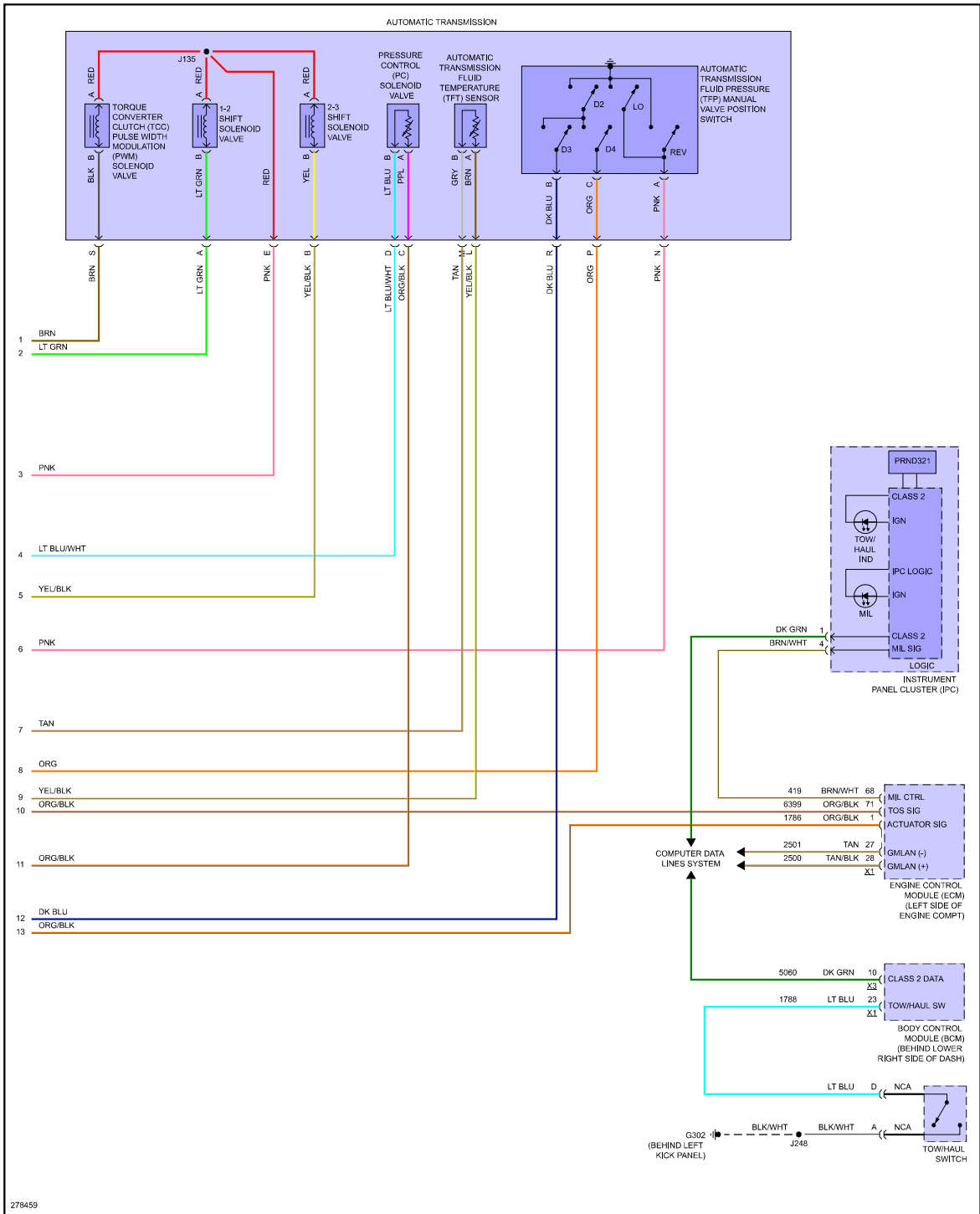
Fig 2: 6.0L VIN K, Transmission Circuit (2 of 2)
