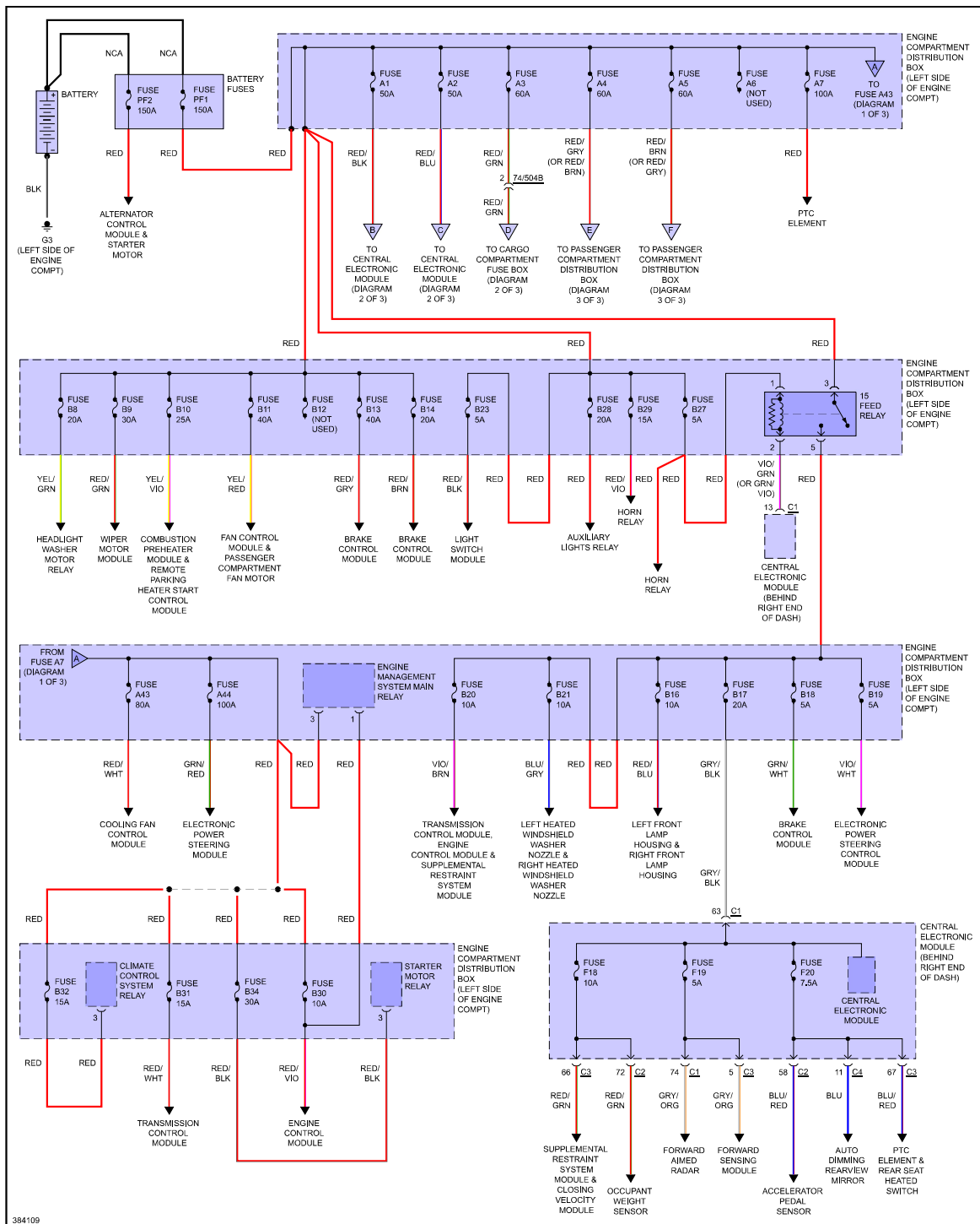
Fig 1: Power Distribution Circuit (1 of 3)
