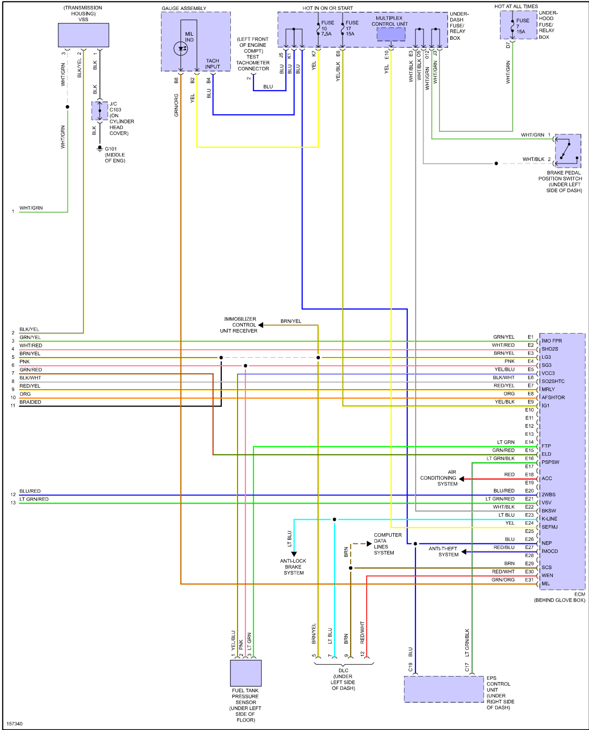
Fig 3: 2.0L, Engine Performance Circuit (3 of 3)
