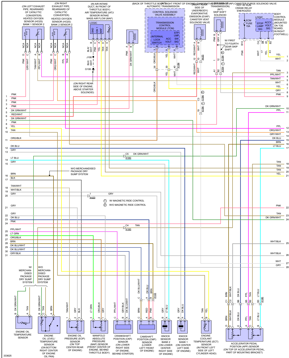
Fig 3: 6.2L VIN W, Engine Performance Circuit (3 of 4)
