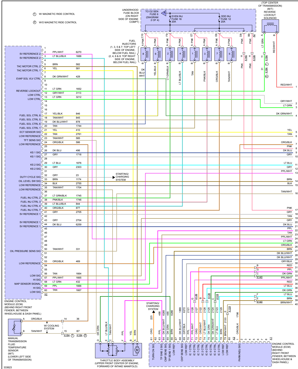
Fig 1: 6.2L VIN W, Engine Performance Circuit (1 of 4)
