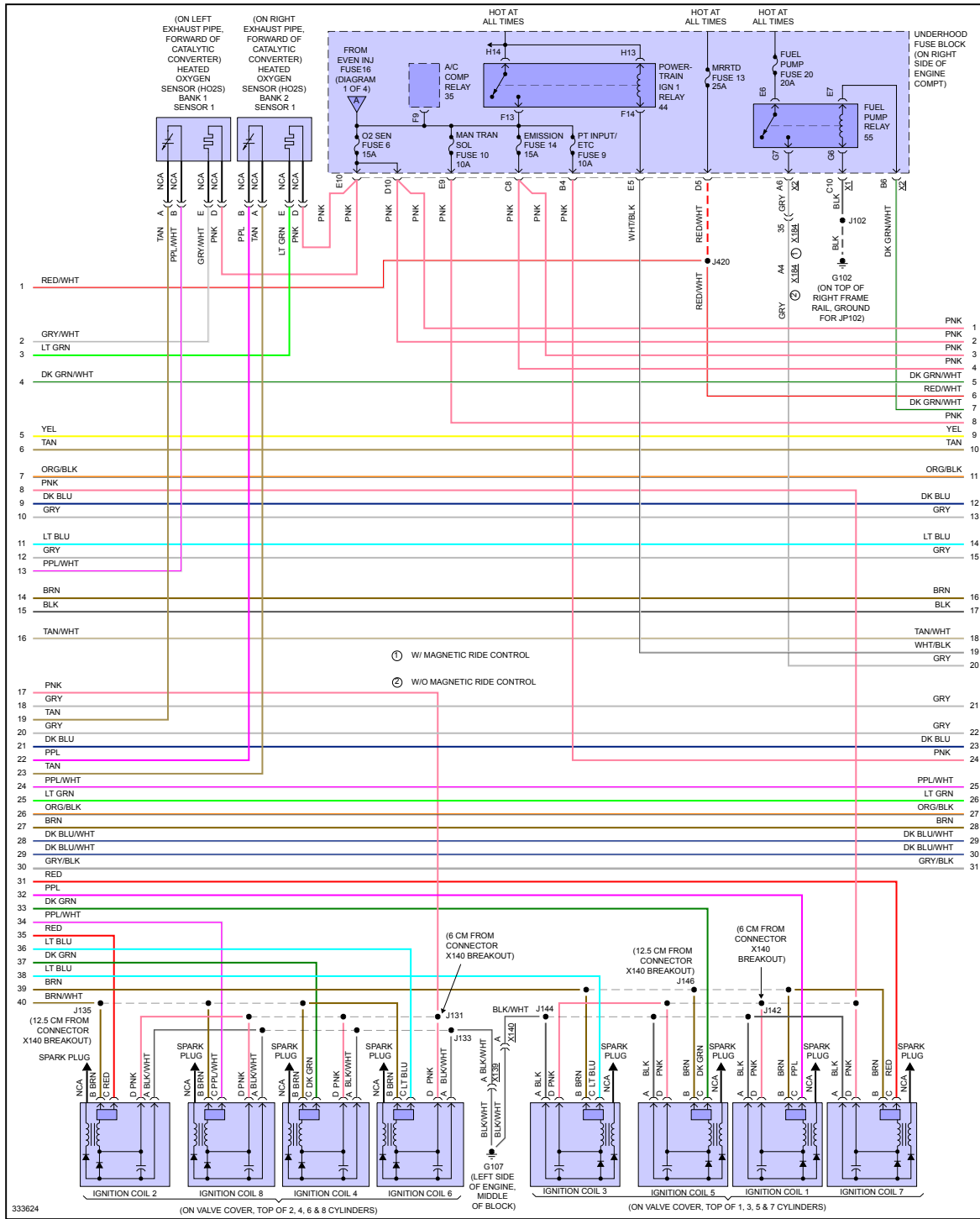
Fig 2: 6.2L VIN W, Engine Performance Circuit (2 of 4)
