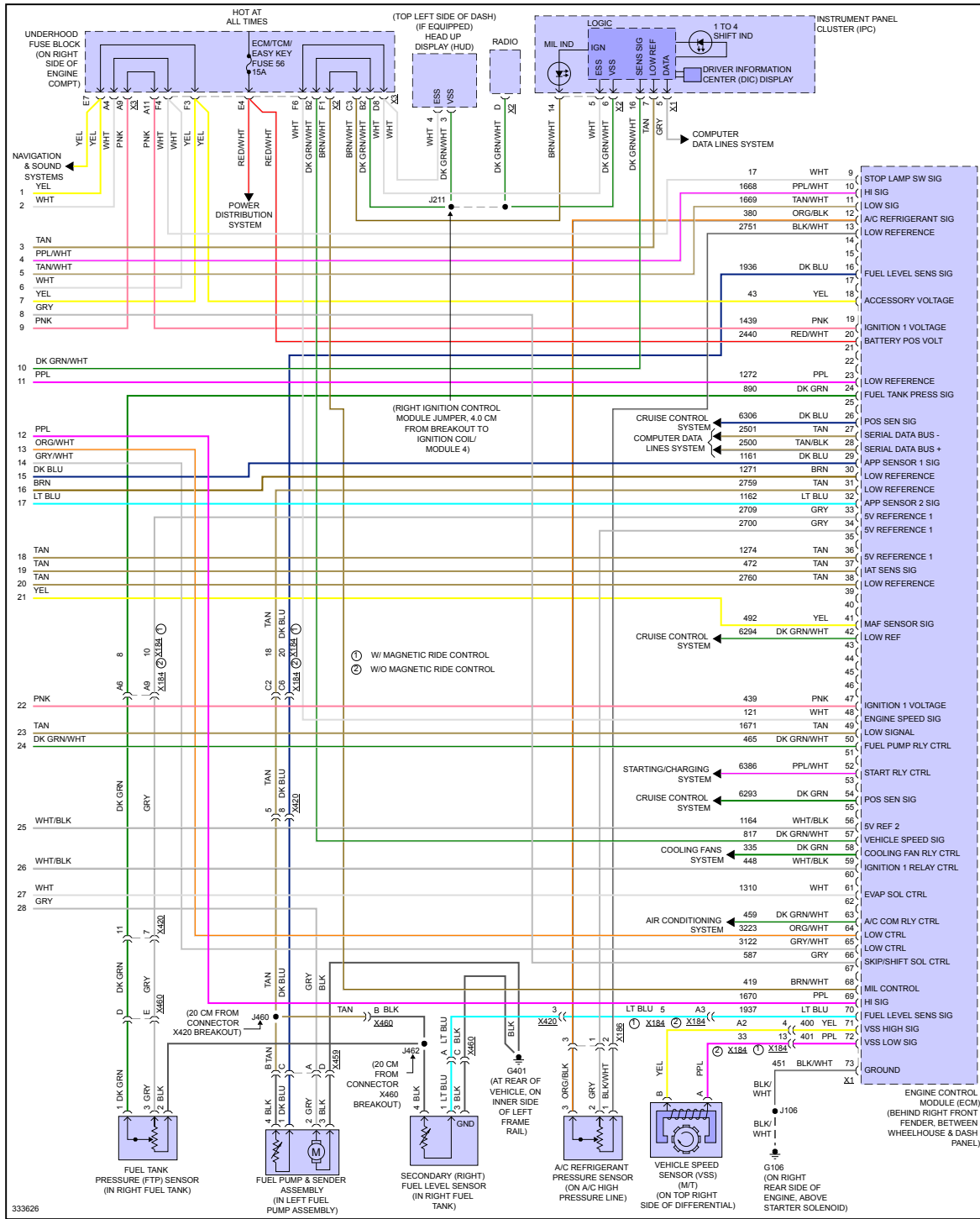
Fig 4: 6.2L VIN W, Engine Performance Circuit (4 of 4)
