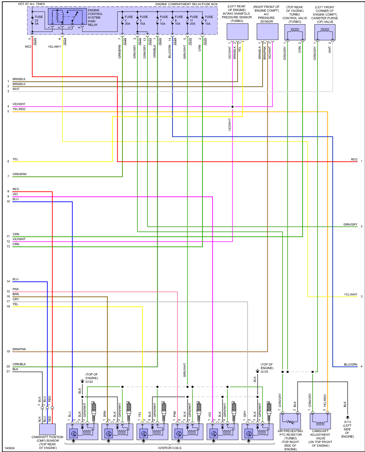
Fig 2: 2.9L, Engine Performance Circuits (2 of 3)
