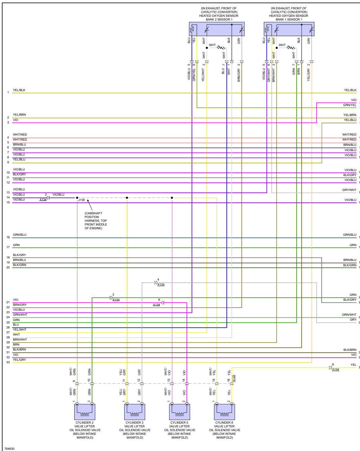
Fig 7: 6.2L VIN 4, Engine Performance Circuit (7 of 10)
