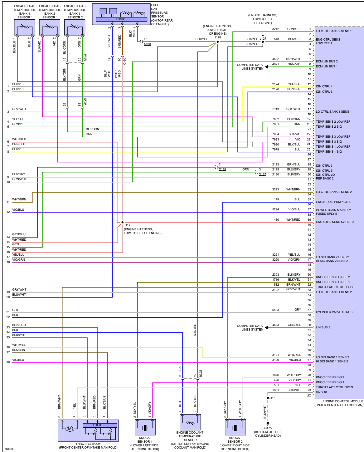
Fig 10: 6.2L VIN 4, Engine Performance Circuit (10 of 10)
