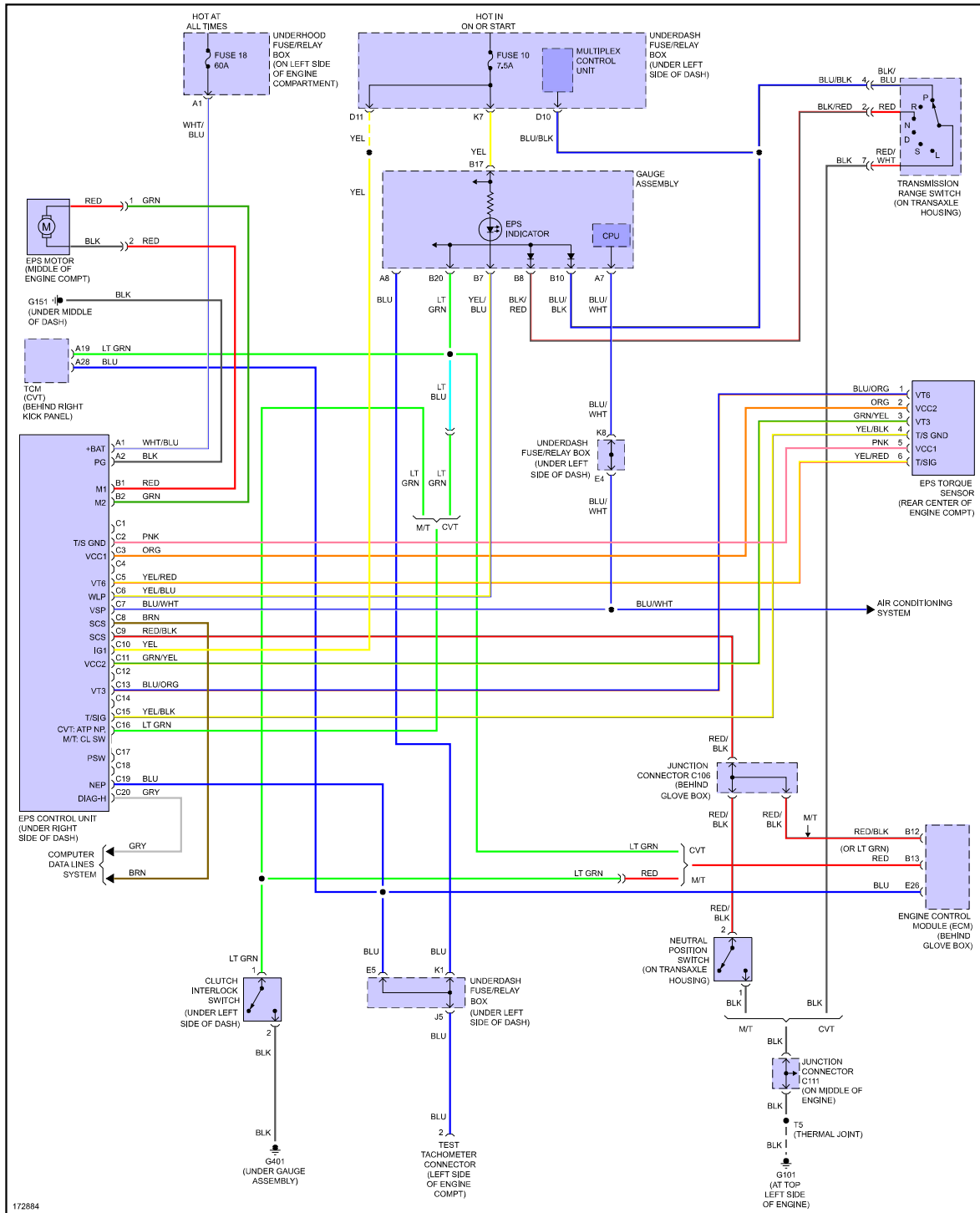
Fig 2: Electronic Power Steering Circuit, Hybrid
