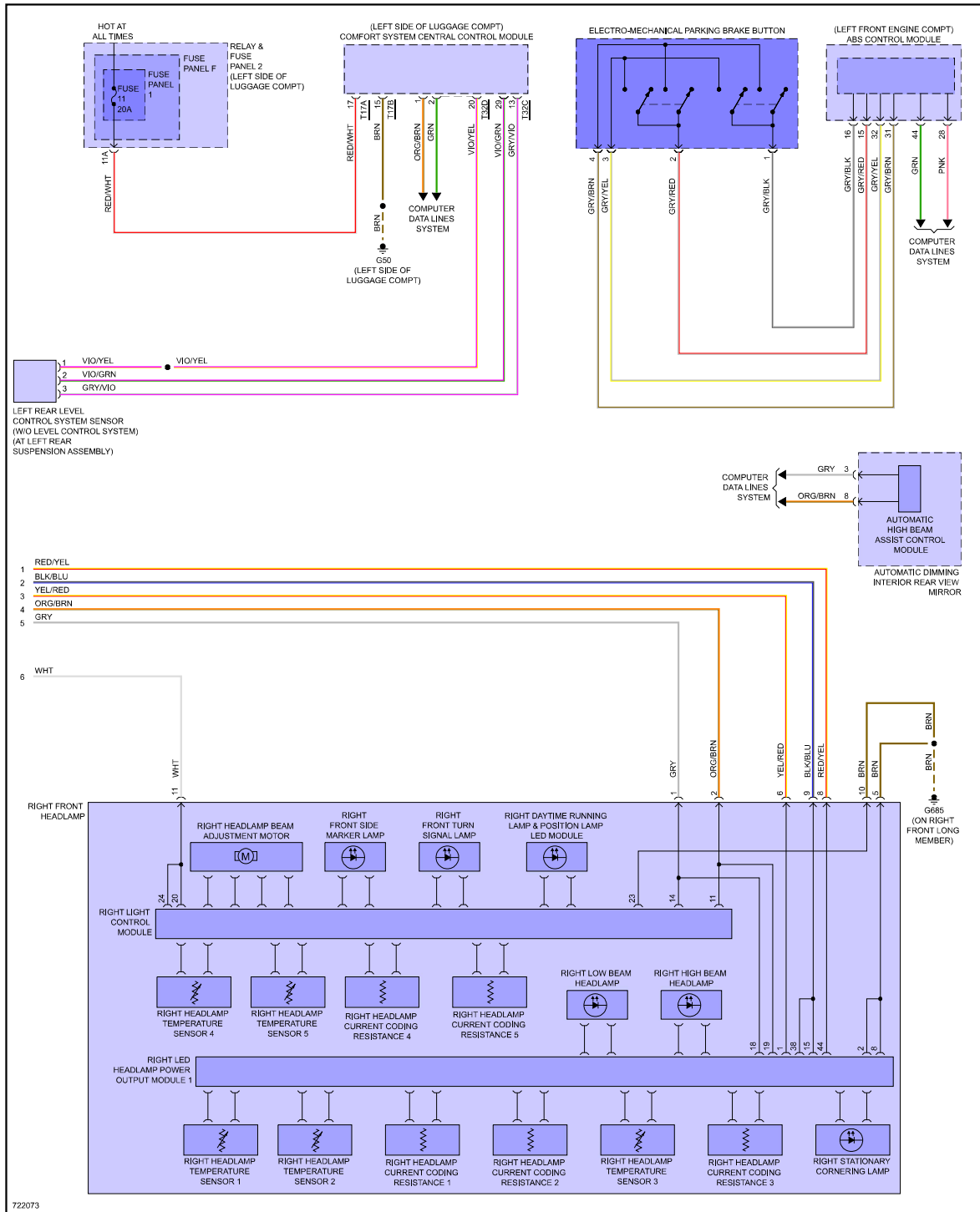
Fig 4: Headlights Circuit, W/O HID & Matrix Beam (2 of 2)
