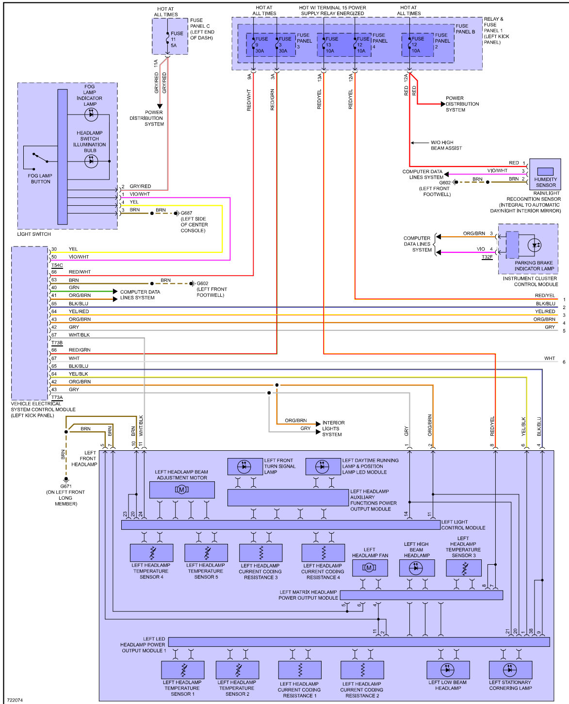
Fig 5: Headlights Circuit, W/O HID W/ Matrix Beam (1 of 2)
