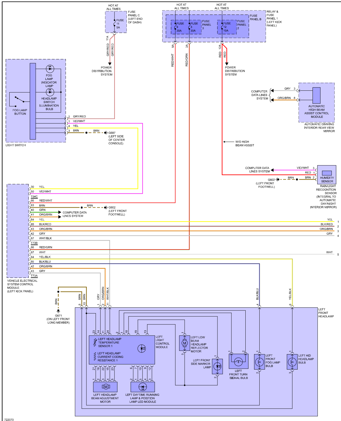
Fig 1: Headlights Circuit, W/ HID (1 of 2)
