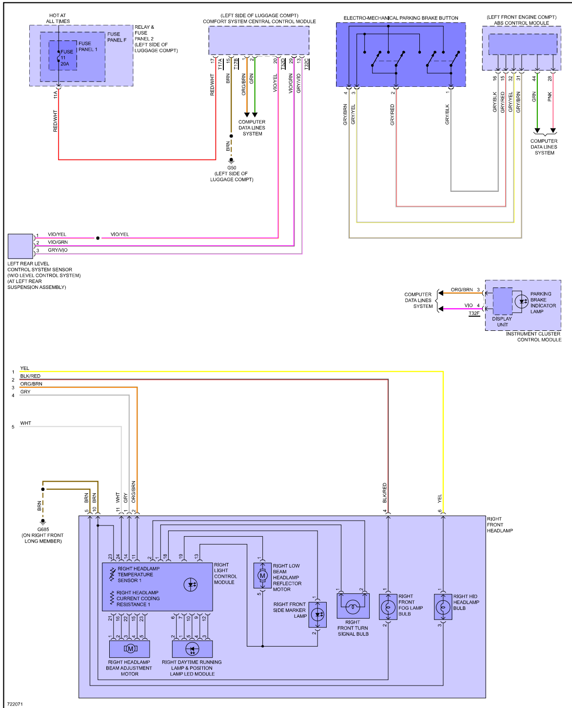
Fig 2: Headlights Circuit, W/ HID (2 of 2)
