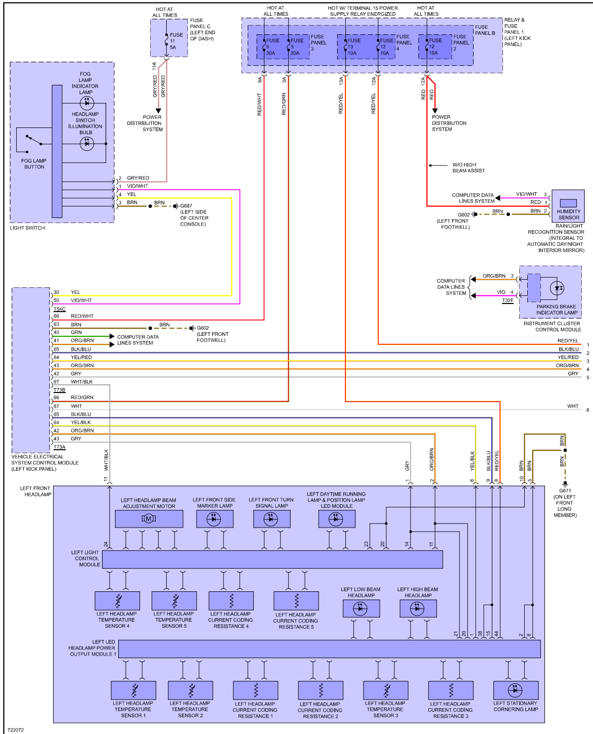
Fig 3: Headlights Circuit, W/O HID & Matrix Beam (1 of 2)
