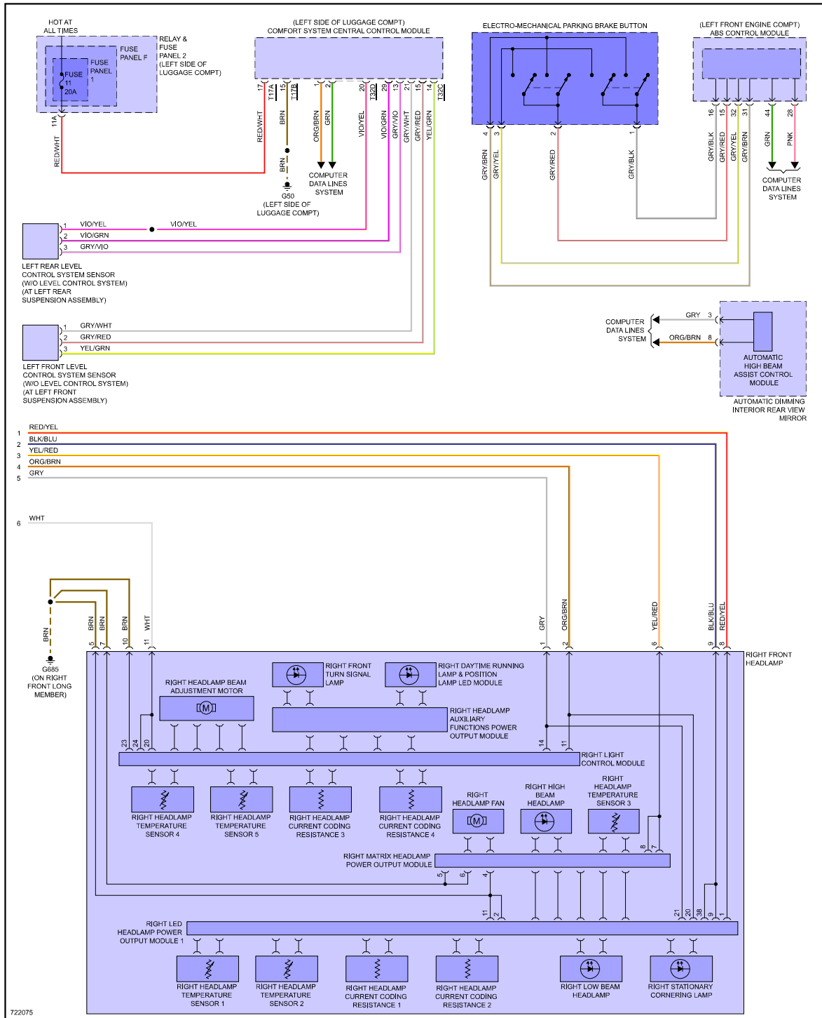
Fig 6: Headlights Circuit, W/O HID W/ Matrix Beam (2 of 2)
