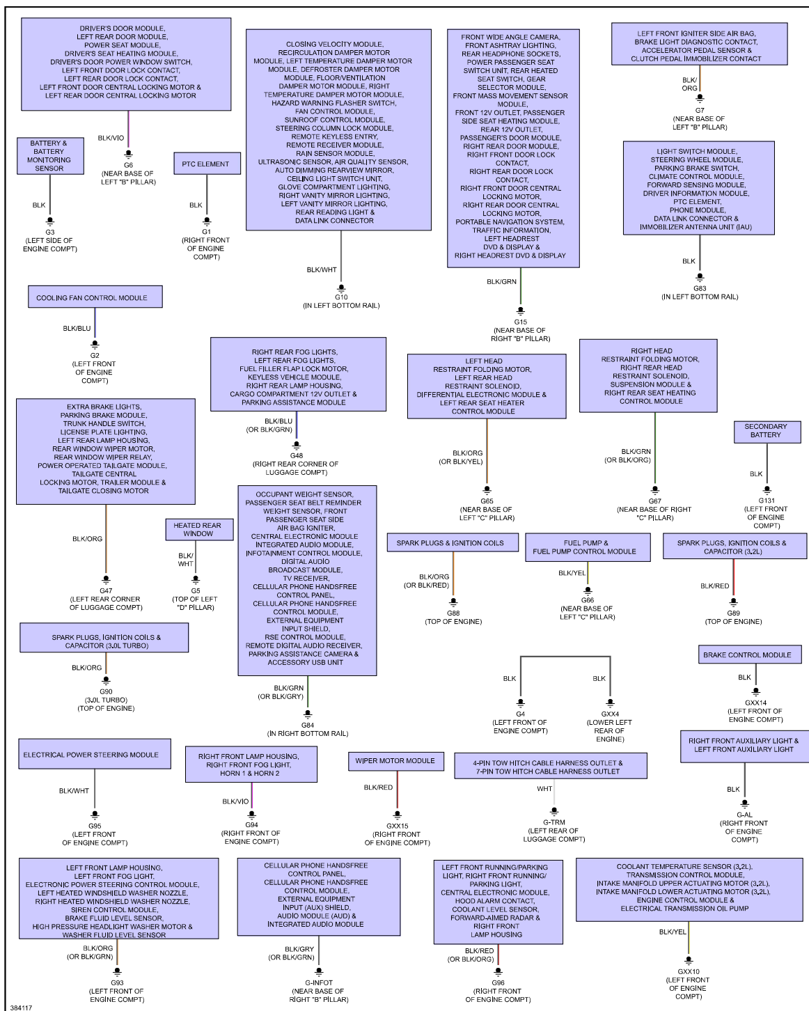
Fig 1: Ground Distribution Circuit
