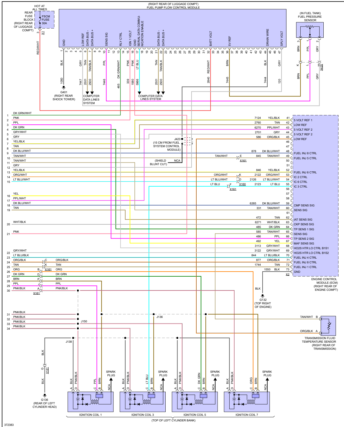
Fig 6: 6.2L VIN P, Engine Performance Circuit (6 of 6)
