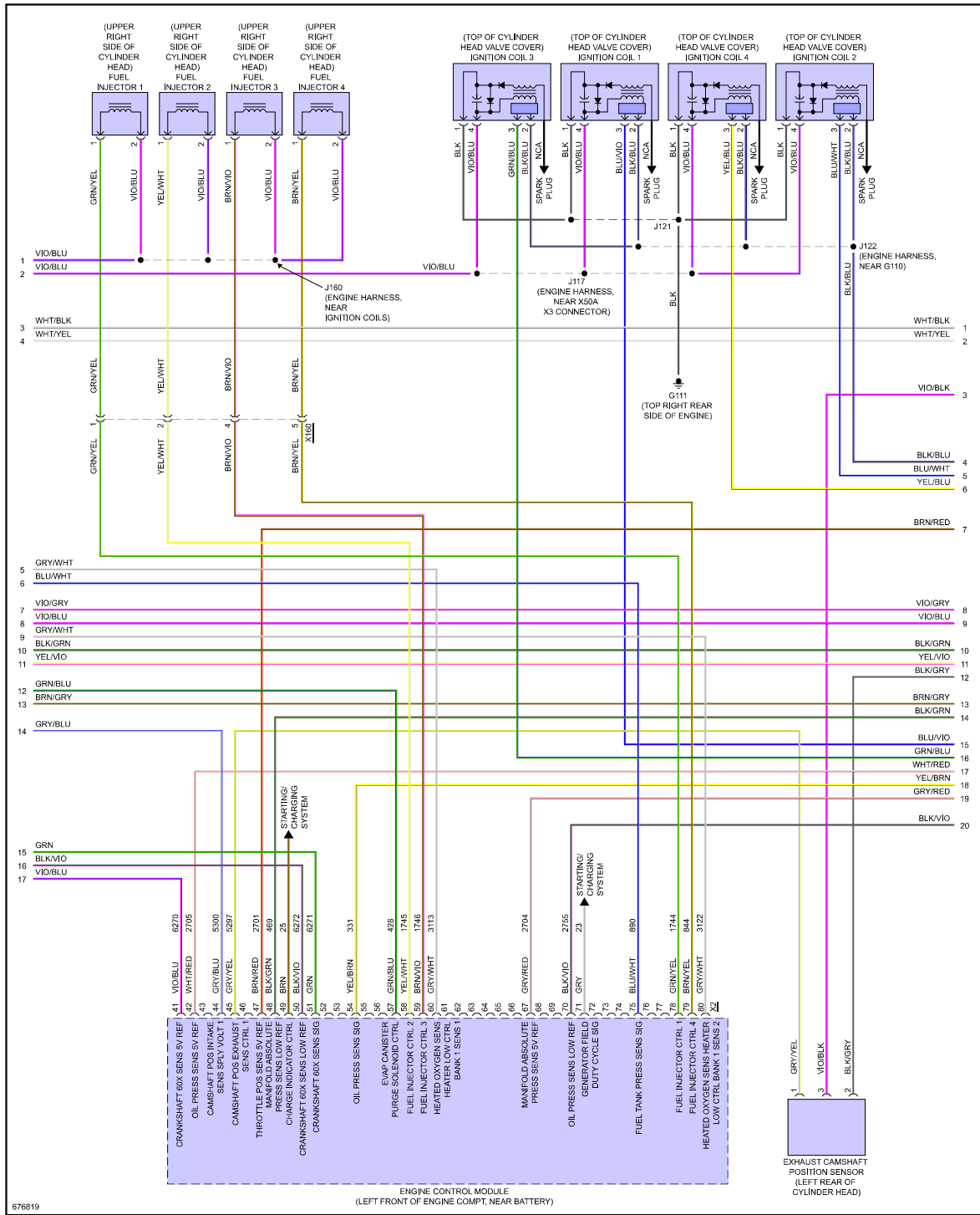
Fig 4: 1.4L VIN A, Engine Performance Circuit (4 of 5)
