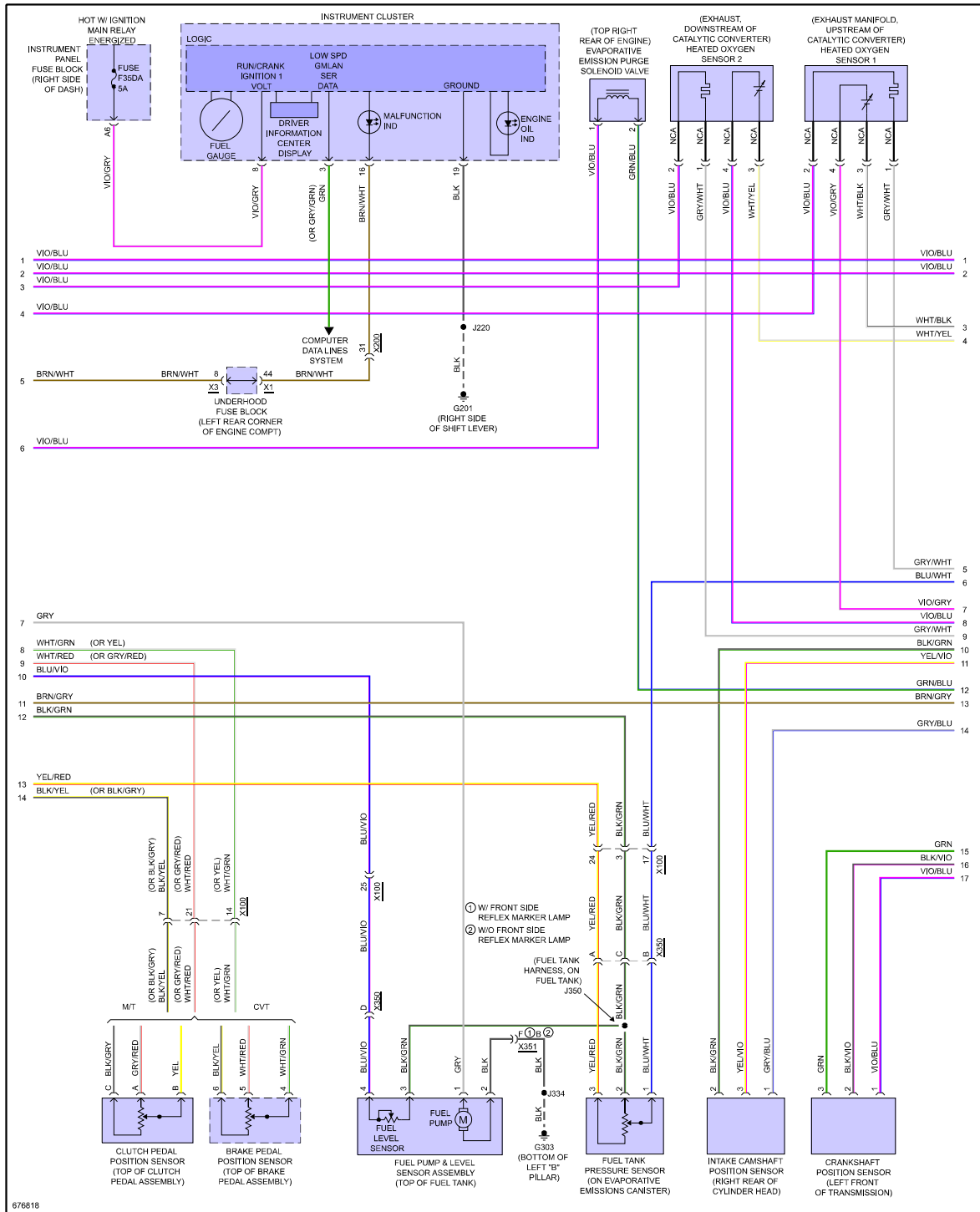
Fig 3: 1.4L VIN A, Engine Performance Circuit (3 of 5)
