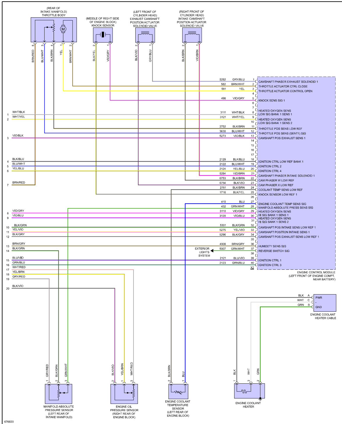
Fig 5: 1.4L VIN A, Engine Performance Circuit (5 of 5)
