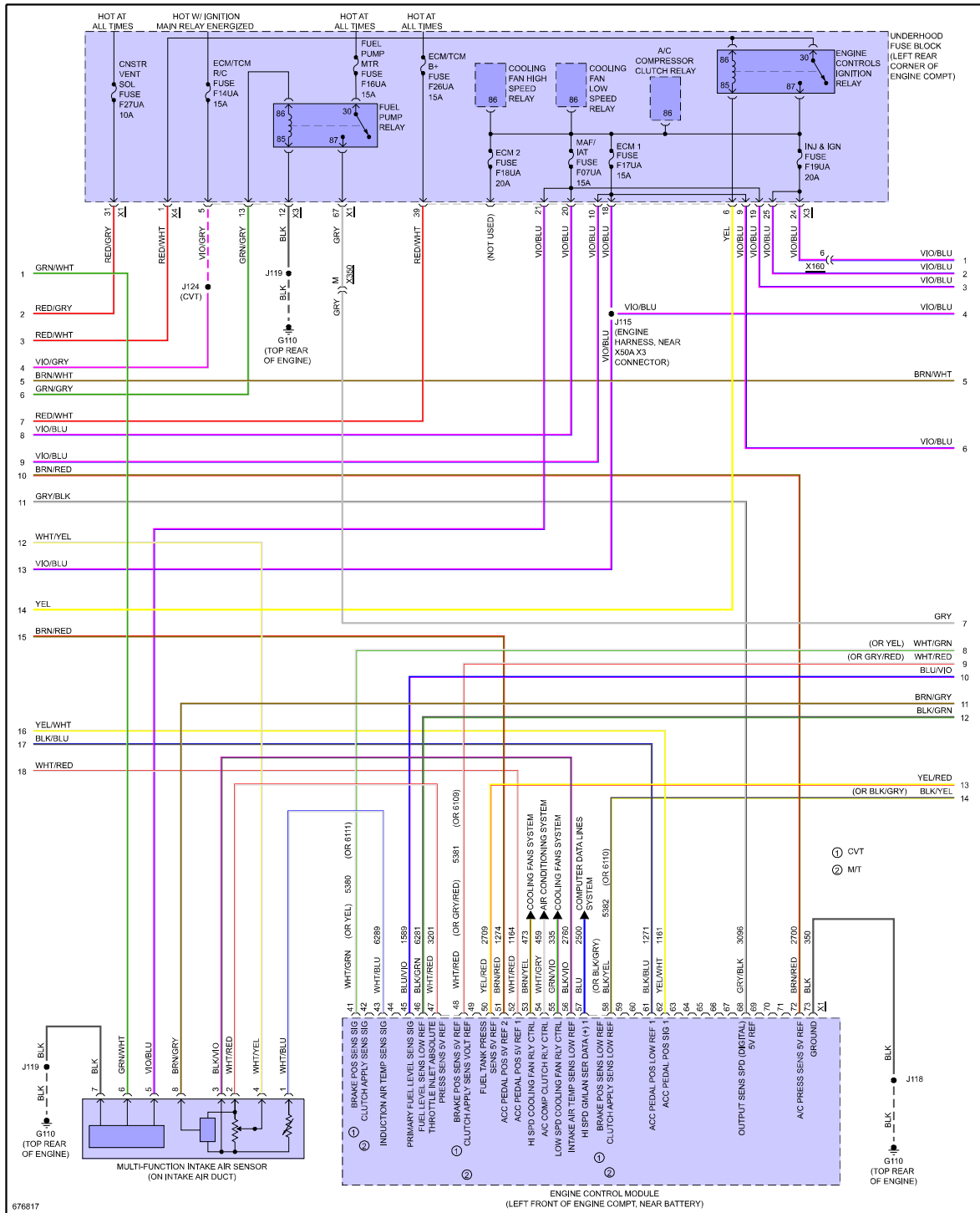
Fig 2: 1.4L VIN A, Engine Performance Circuit (2 of 5)
