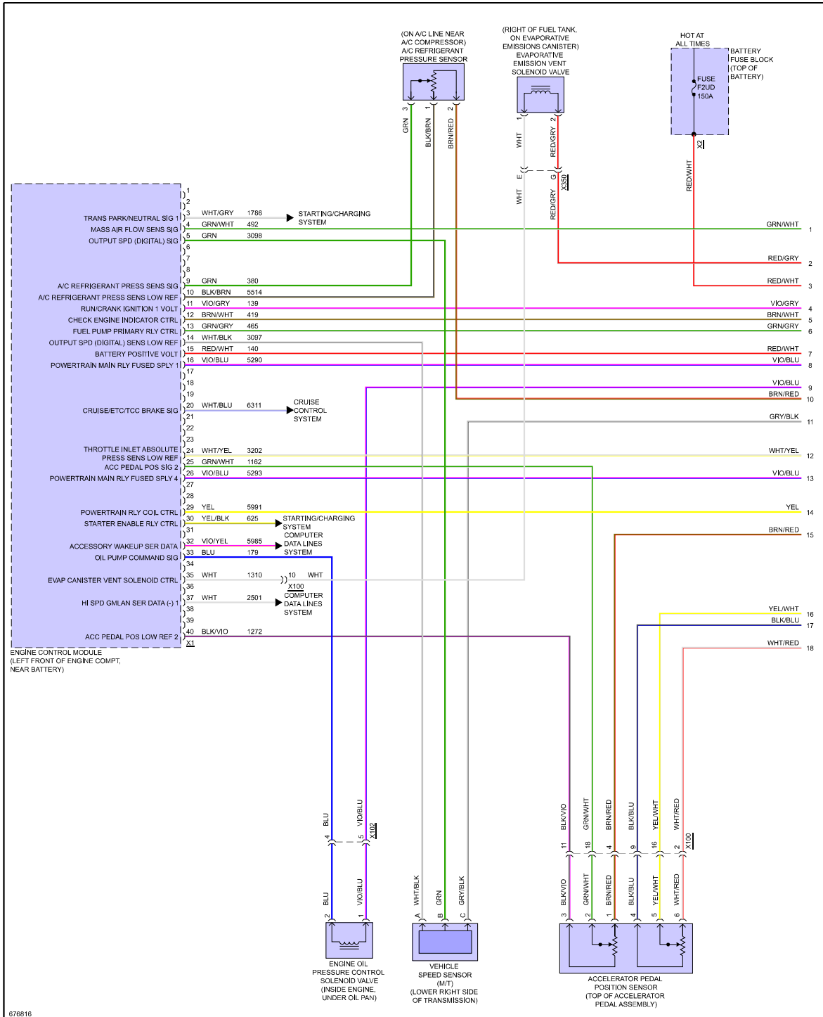
Fig 1: 1.4L VIN A, Engine Performance Circuit (1 of 5)
