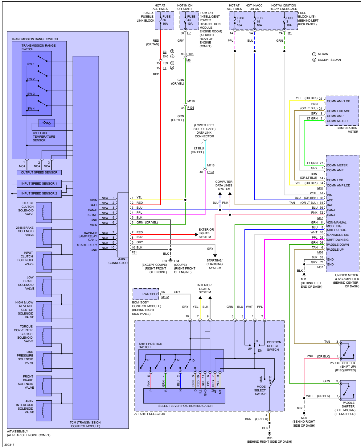
Fig 1: A/T Circuit
