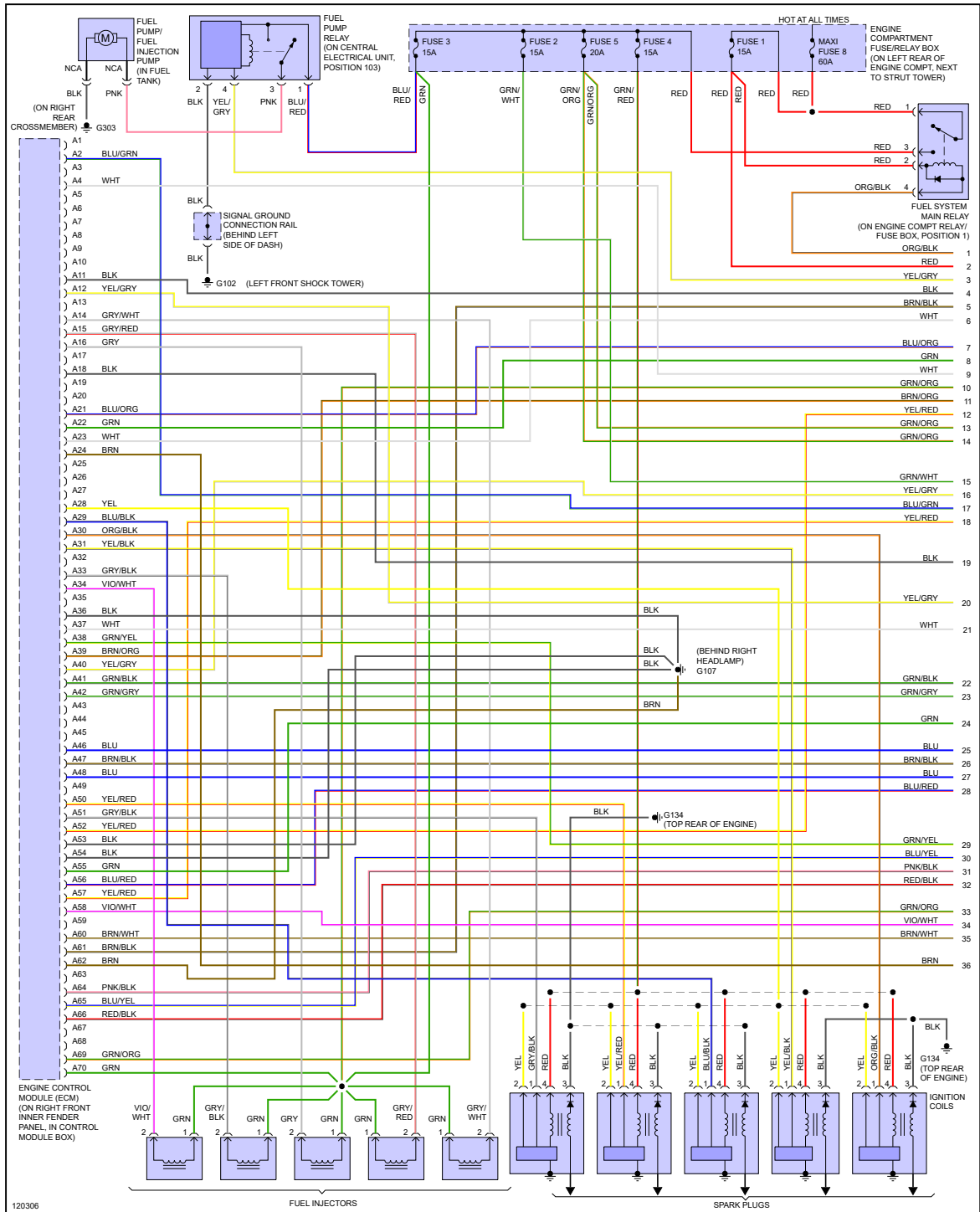
Fig 1: 2.4L, Engine Performance Circuit (1 of 3)
