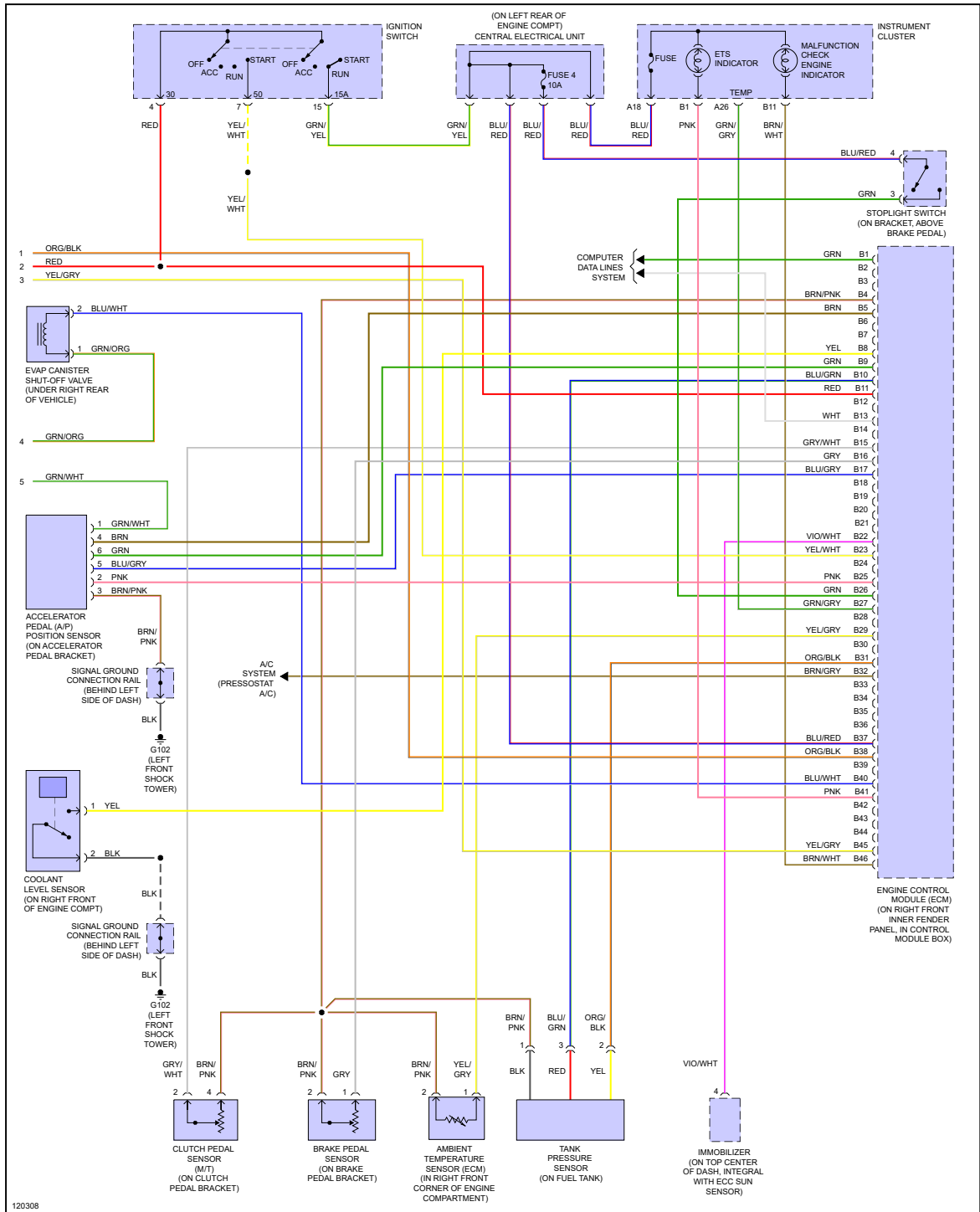
Fig 3: 2.4L, Engine Performance Circuit (3 of 3)
