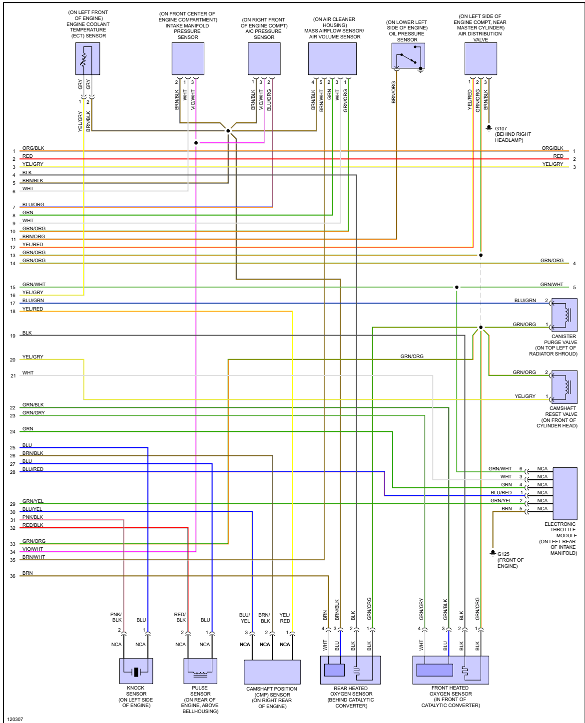
Fig 2: 2.4L, Engine Performance Circuit (2 of 3)
