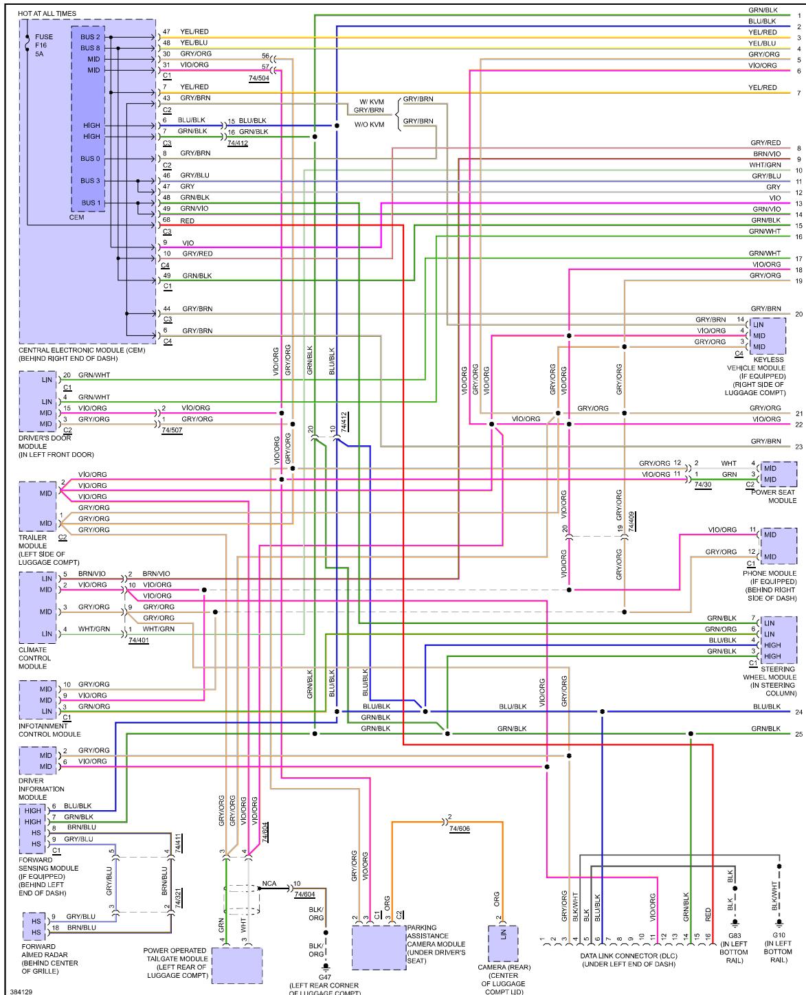
Fig 1: Computer Data Lines Circuit (1 of 3)
