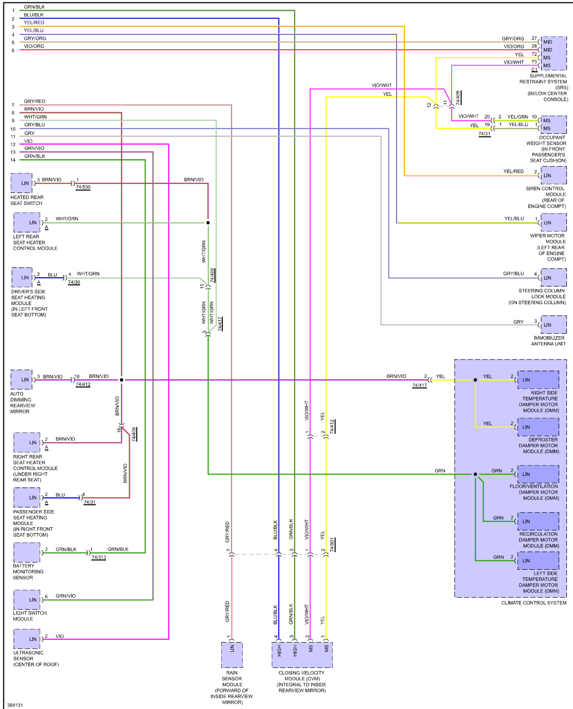
Fig 3: Computer Data Lines Circuit (3 of 3)
