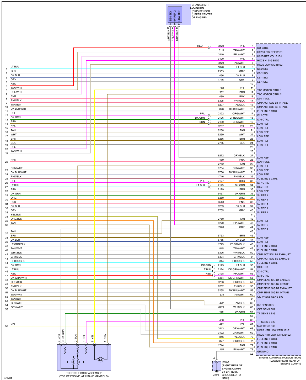
Fig 6: 4.6L VIN A, Engine Performance Circuit (6 of 6)
