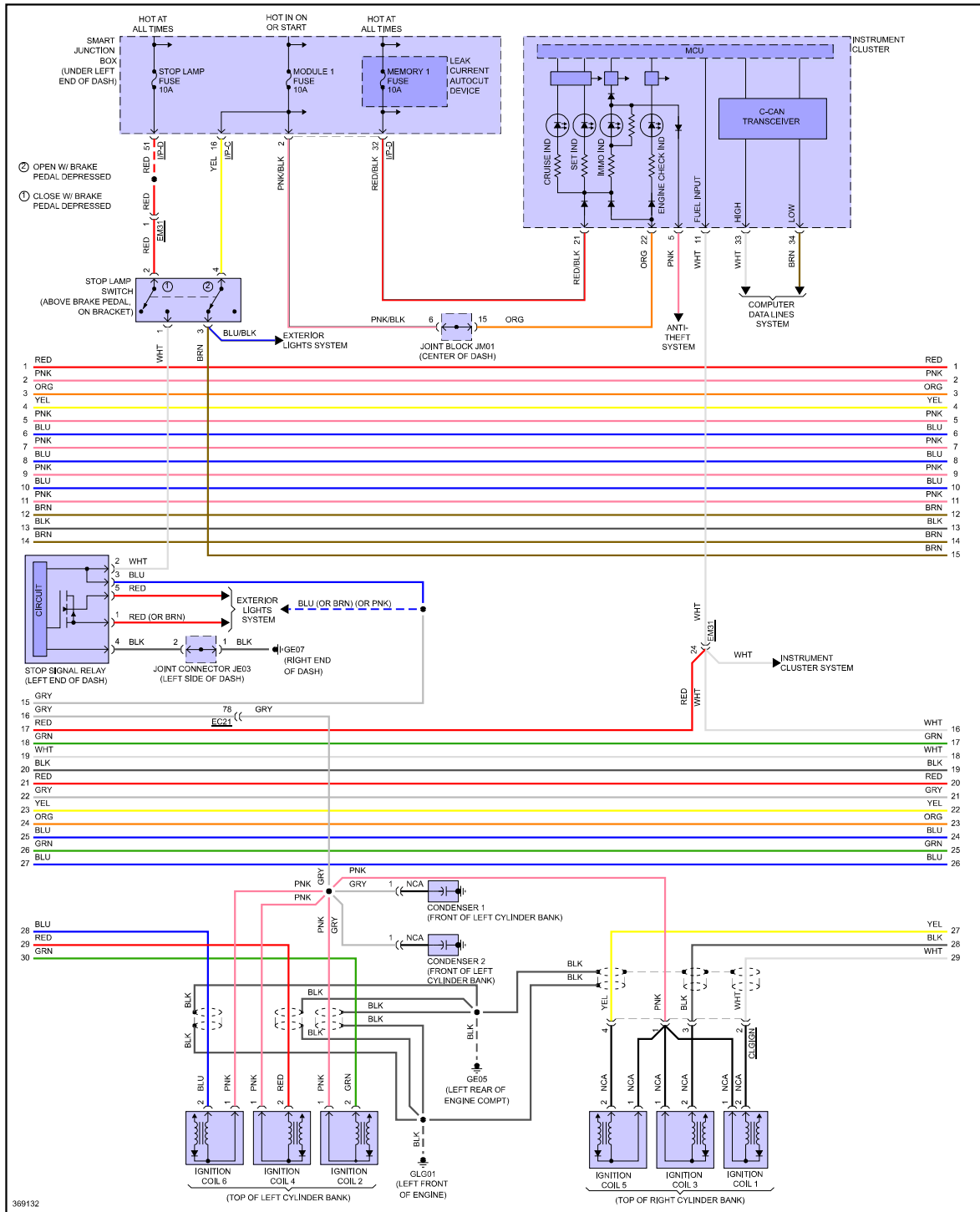
Fig 3: 3.3L, Engine Performance Circuit (3 of 7)
