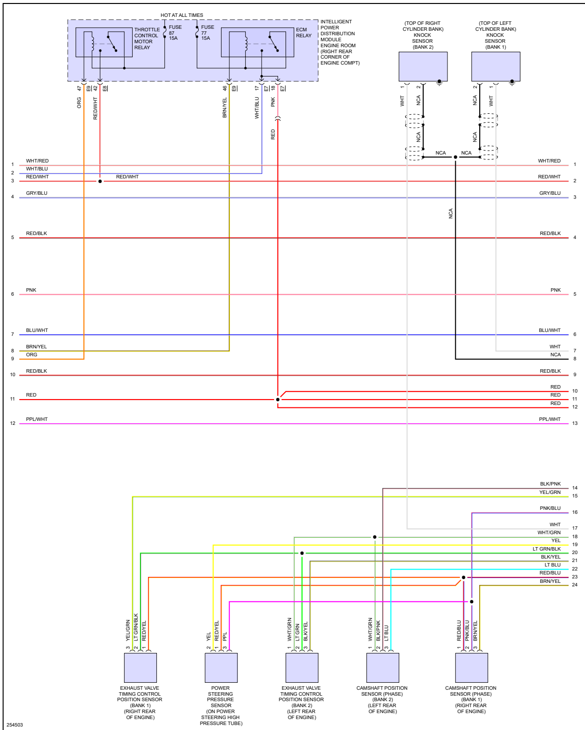
Fig 3: 3.5L, Engine Performance Circuit (3 of 6)
