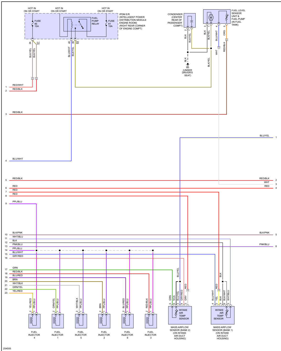
Fig 5: 3.5L, Engine Performance Circuit (5 of 6)
