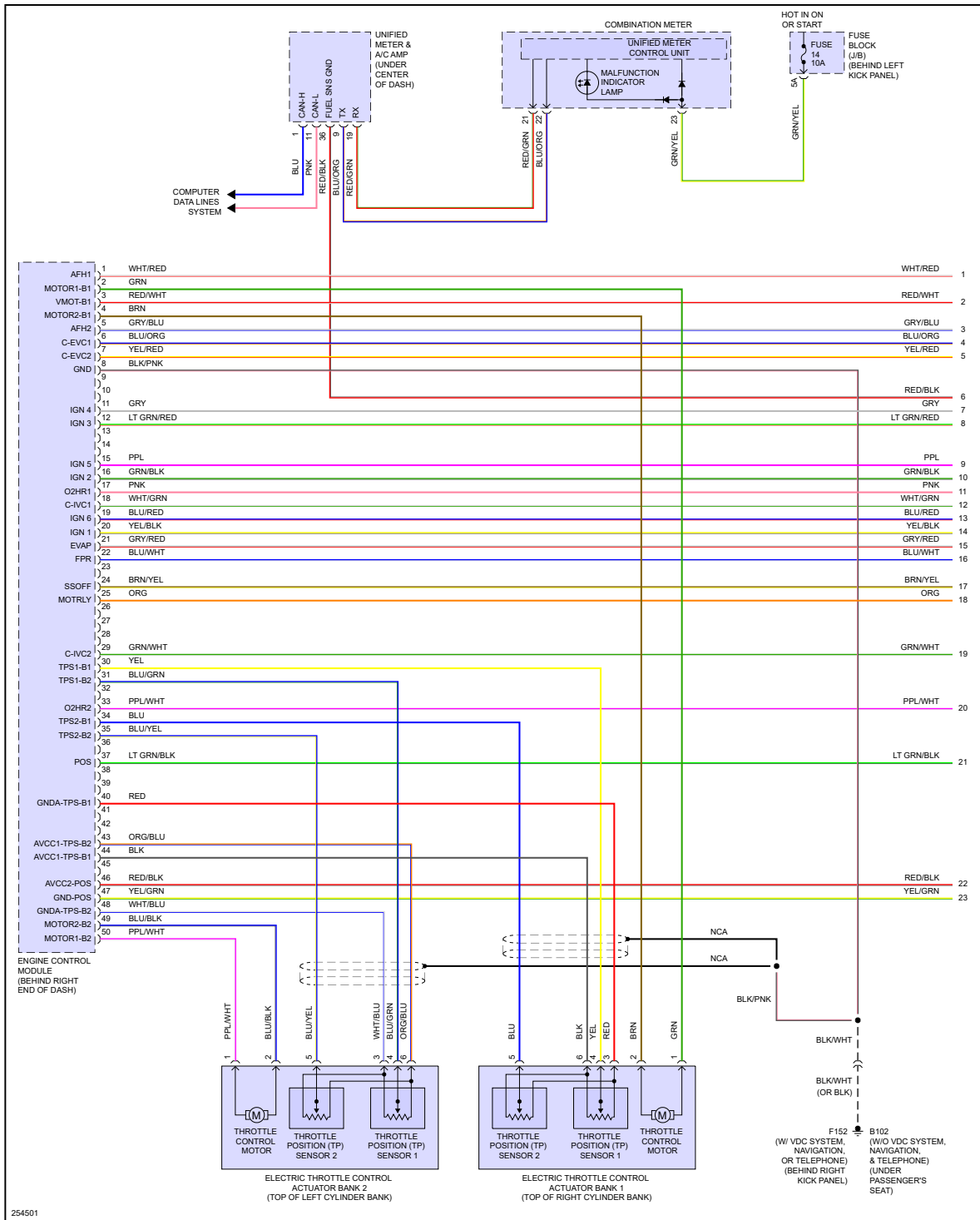
Fig 1: 3.5L, Engine Performance Circuit (1 of 6)
