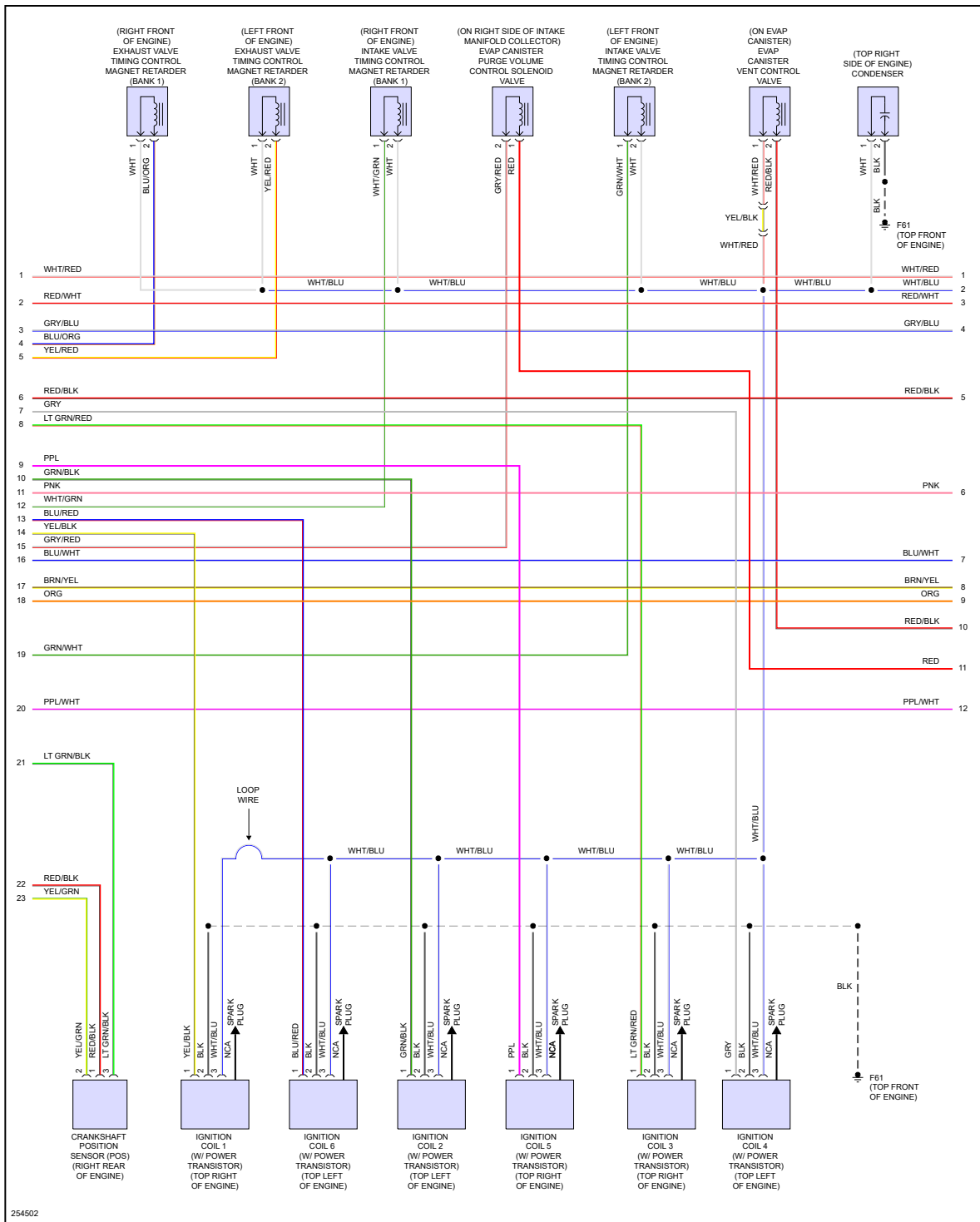
Fig 2: 3.5L, Engine Performance Circuit (2 of 6)
