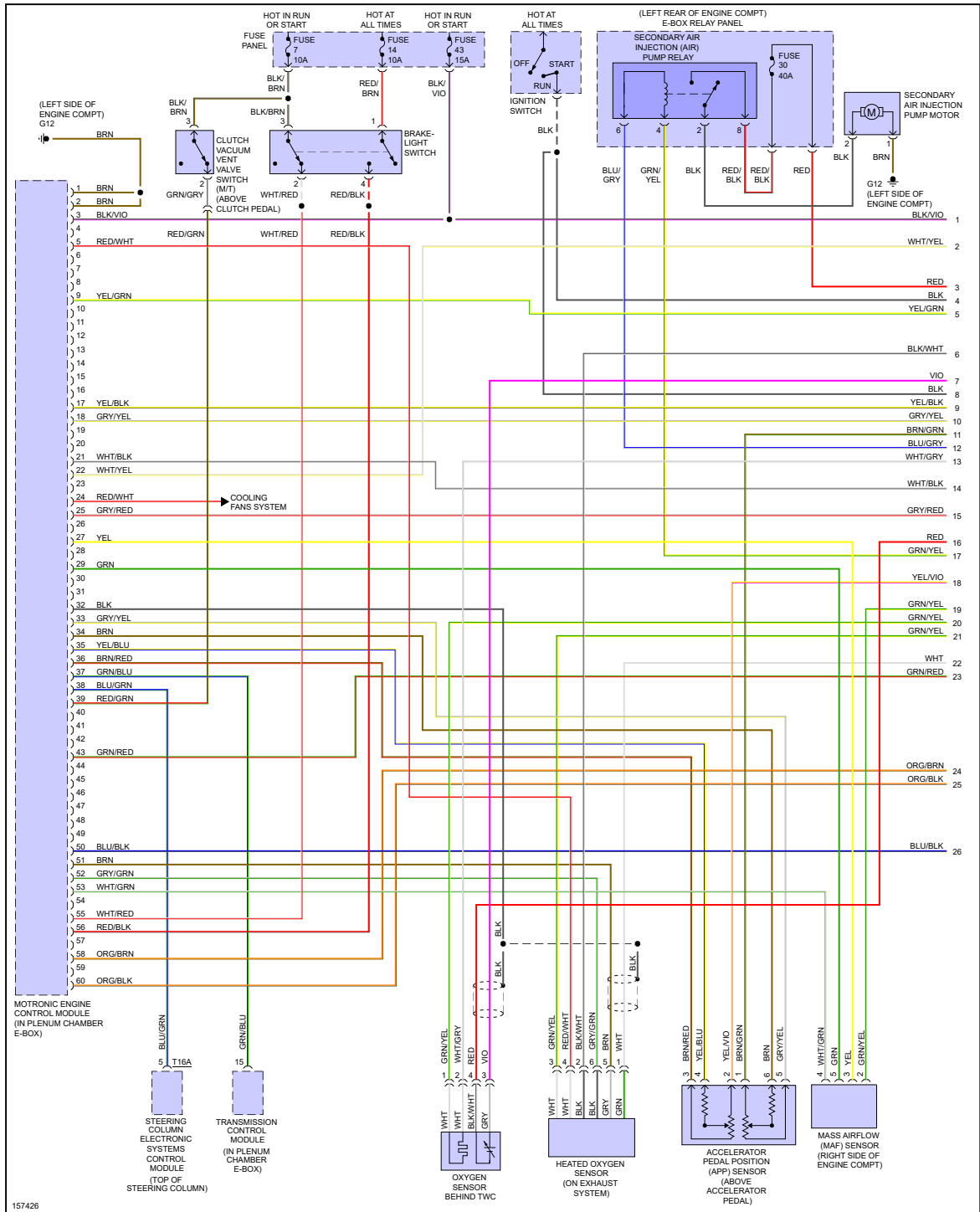
Fig 1: 1.8L, Engine Performance Circuit (1 of 4)
