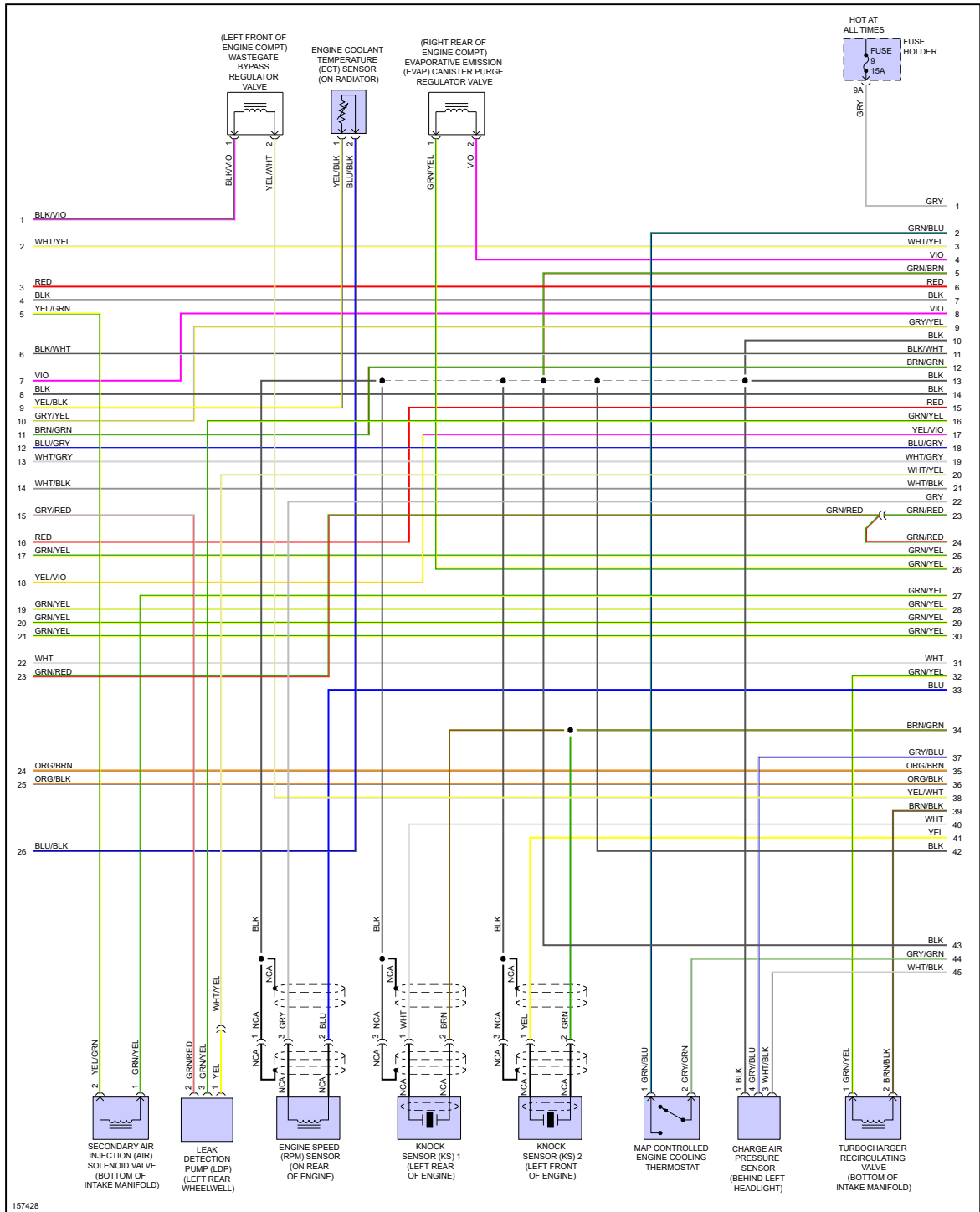
Fig 2: 1.8L, Engine Performance Circuit (2 of 4)
