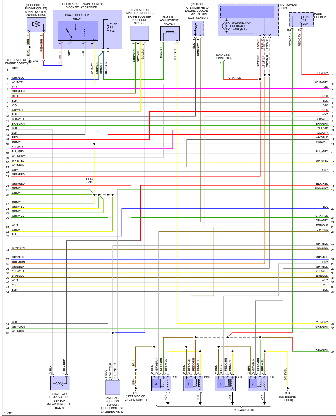
Fig 3: 1.8L, Engine Performance Circuit (3 of 4)
