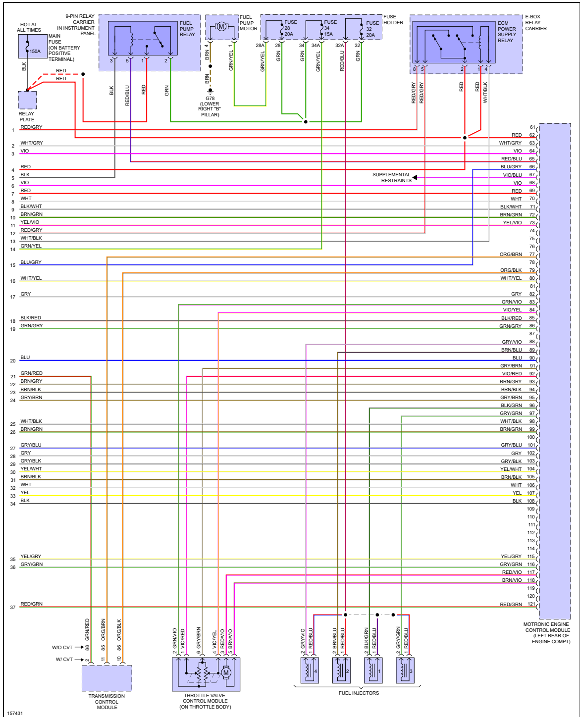
Fig 4: 1.8L, Engine Performance Circuit (4 of 4)
