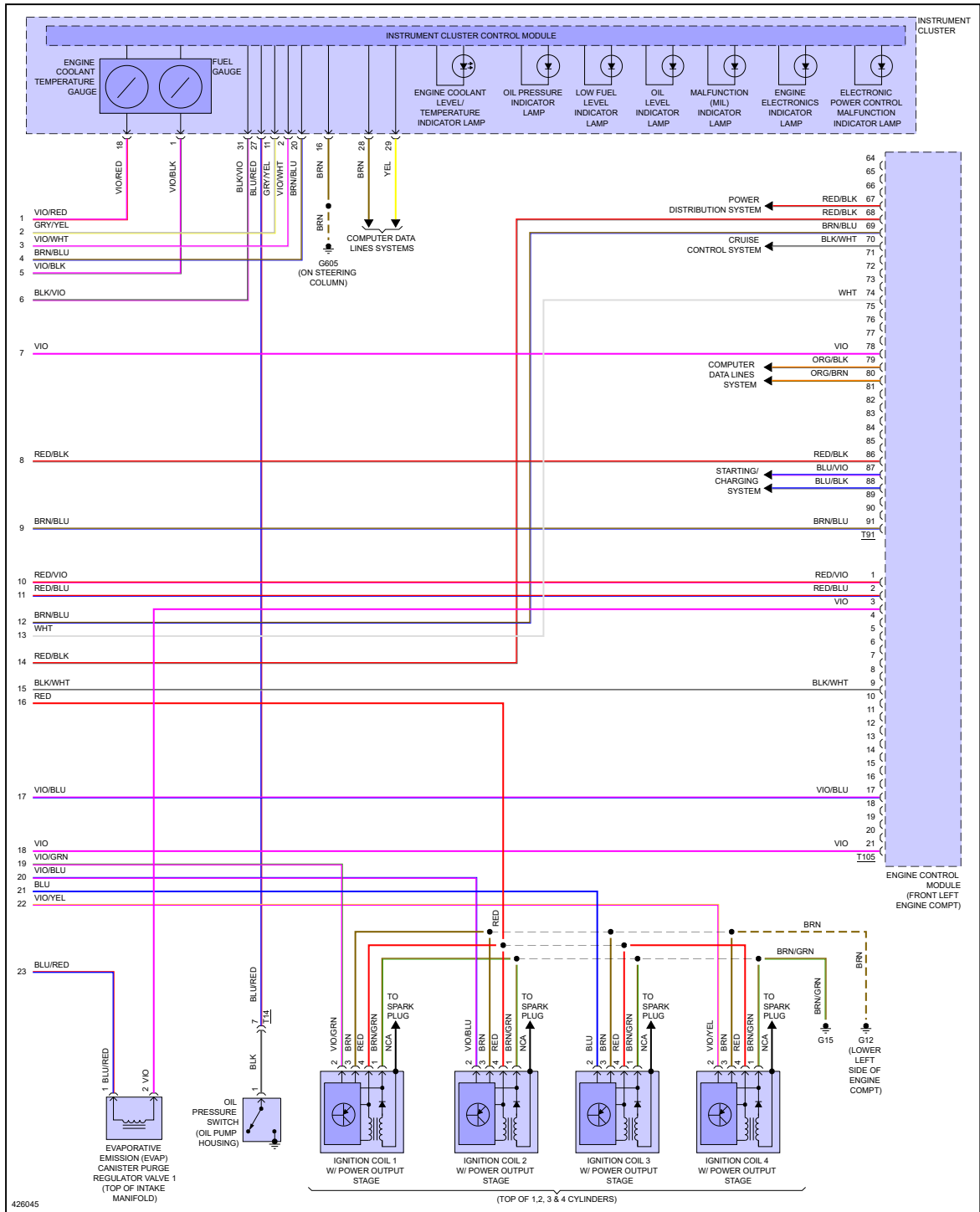
Fig 6: 2.0L Turbo, Engine Performance Circuit (6 of 6)
