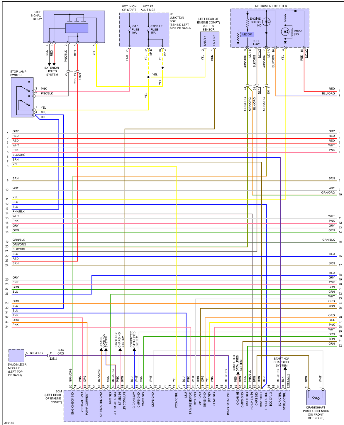
Fig 8: 1.6L, Engine Performance Circuit, M/T (3 of 4)
