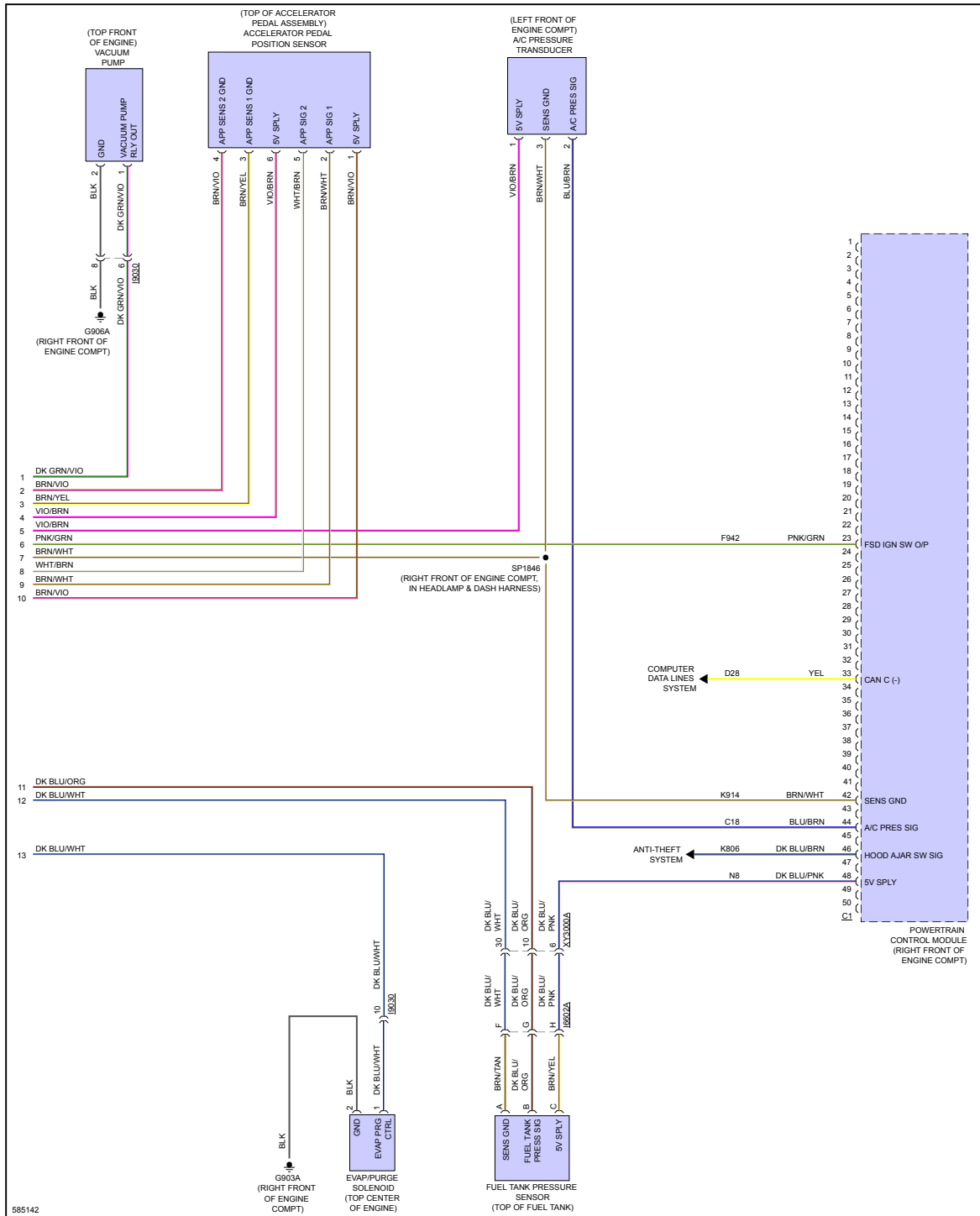
Fig 6: 3.6L, Engine Performance Circuit (6 of 6)
