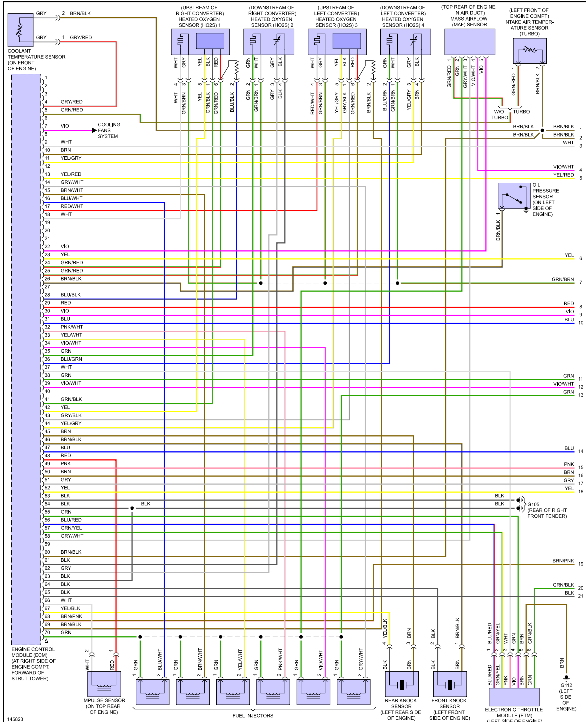
Fig 1: 2.8L Turbo, Engine Performance Circuits (1 of 3)
