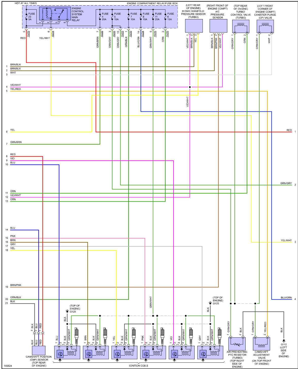
Fig 2: 2.8L Turbo, Engine Performance Circuits (2 of 3)
