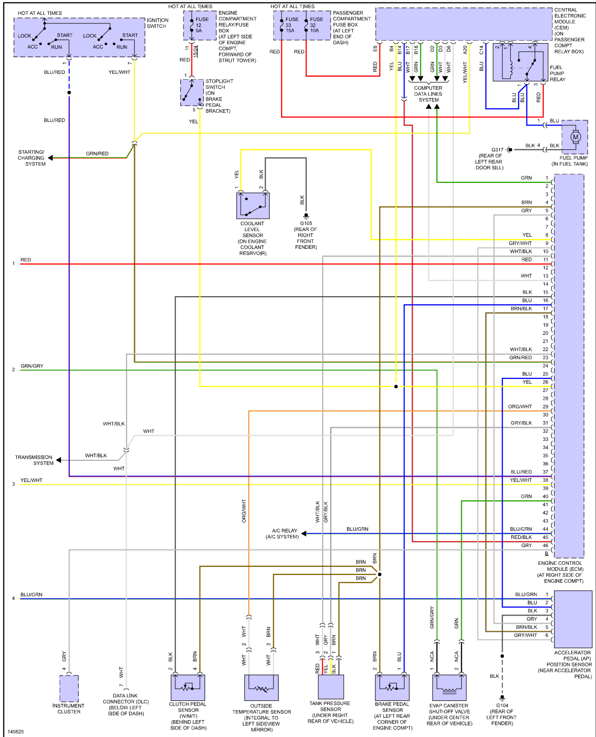
Fig 3: 2.8L Turbo, Engine Performance Circuits (3 of 3)
