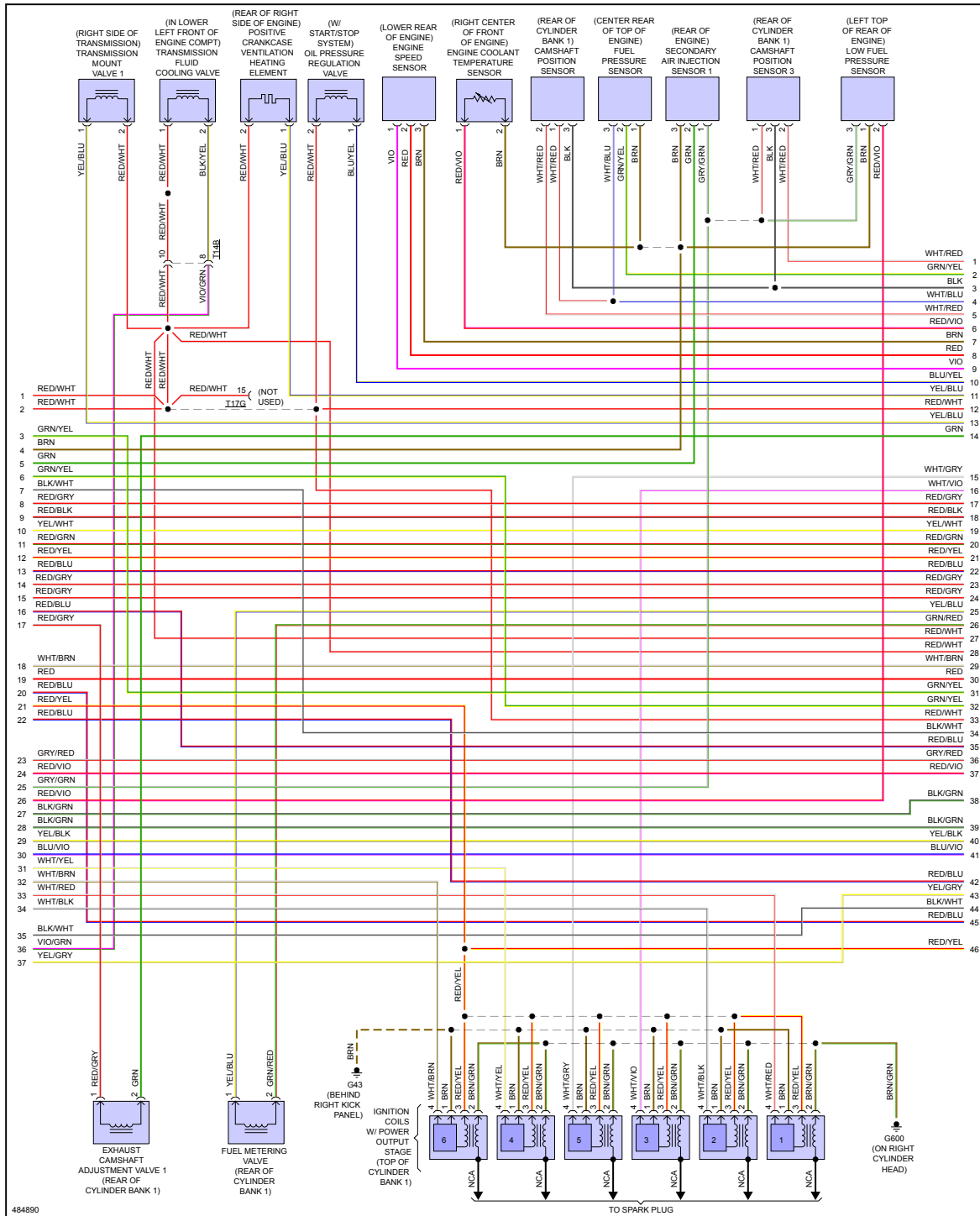
Fig 5: 6.3L, Engine Performance Circuit (5 of 11)
