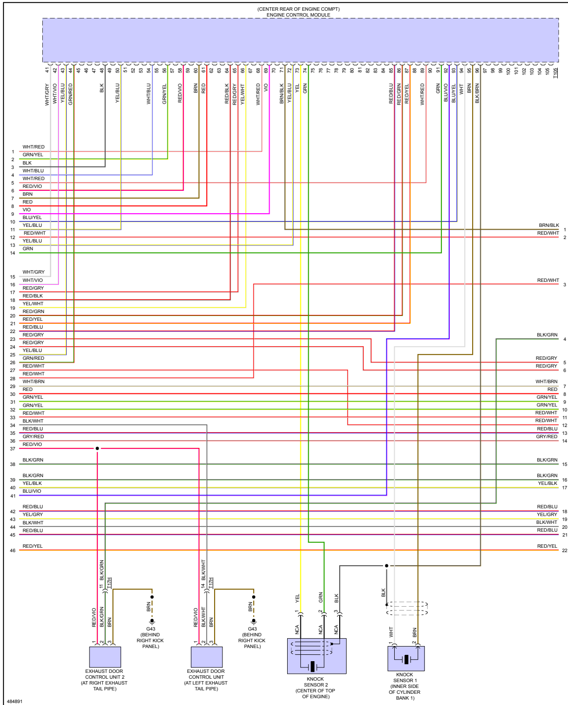
Fig 6: 6.3L, Engine Performance Circuit (6 of 11)
