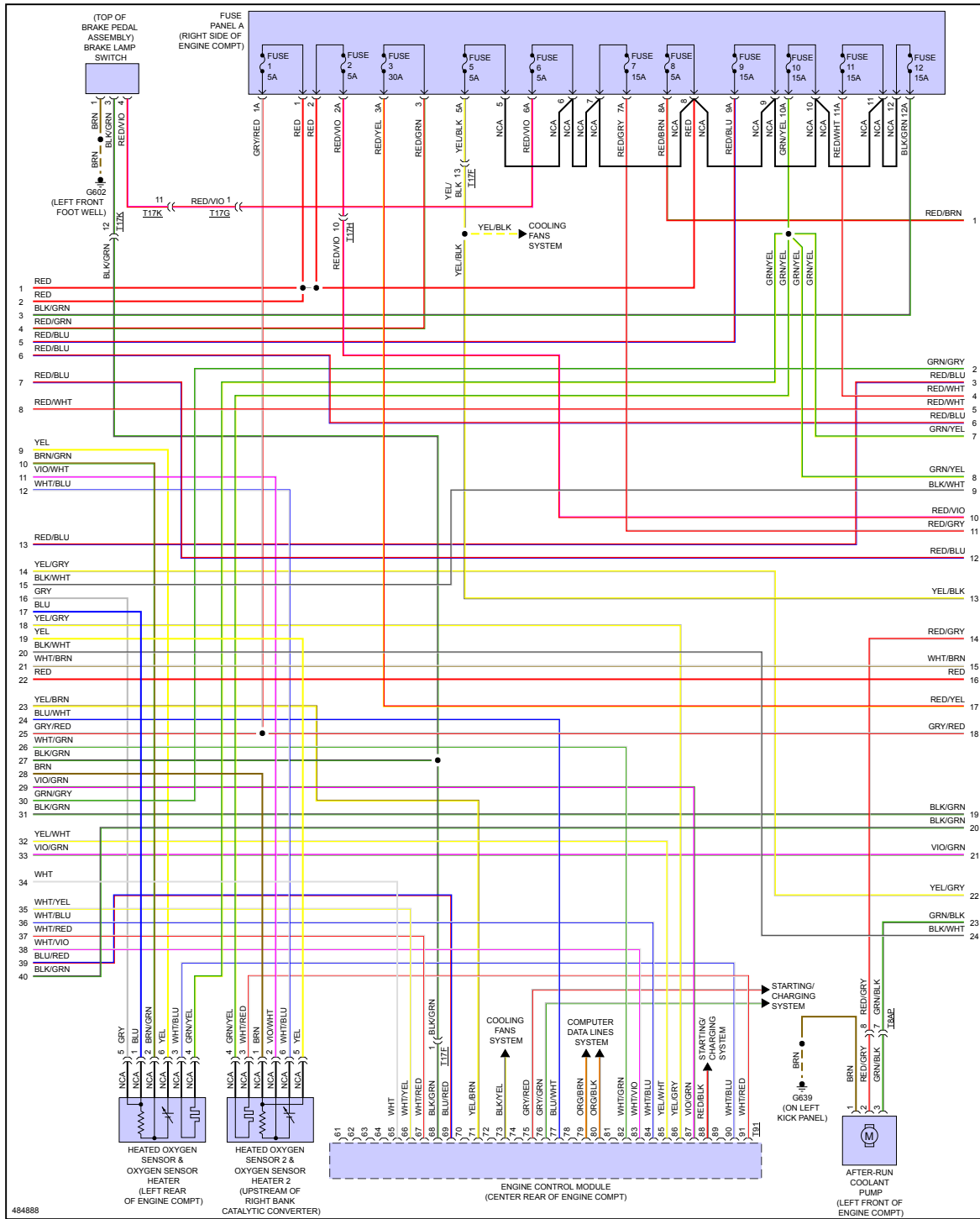
Fig 3: 6.3L, Engine Performance Circuit (3 of 11)
