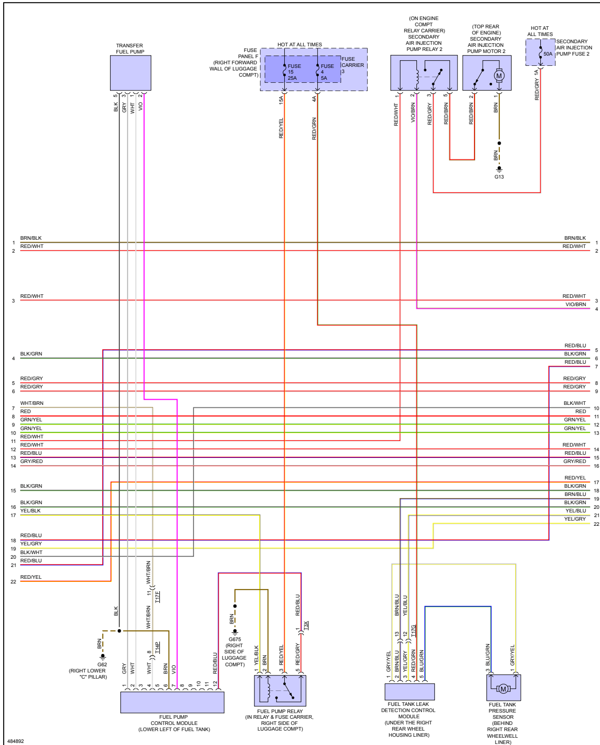
Fig 7: 6.3L, Engine Performance Circuit (7 of 11)
