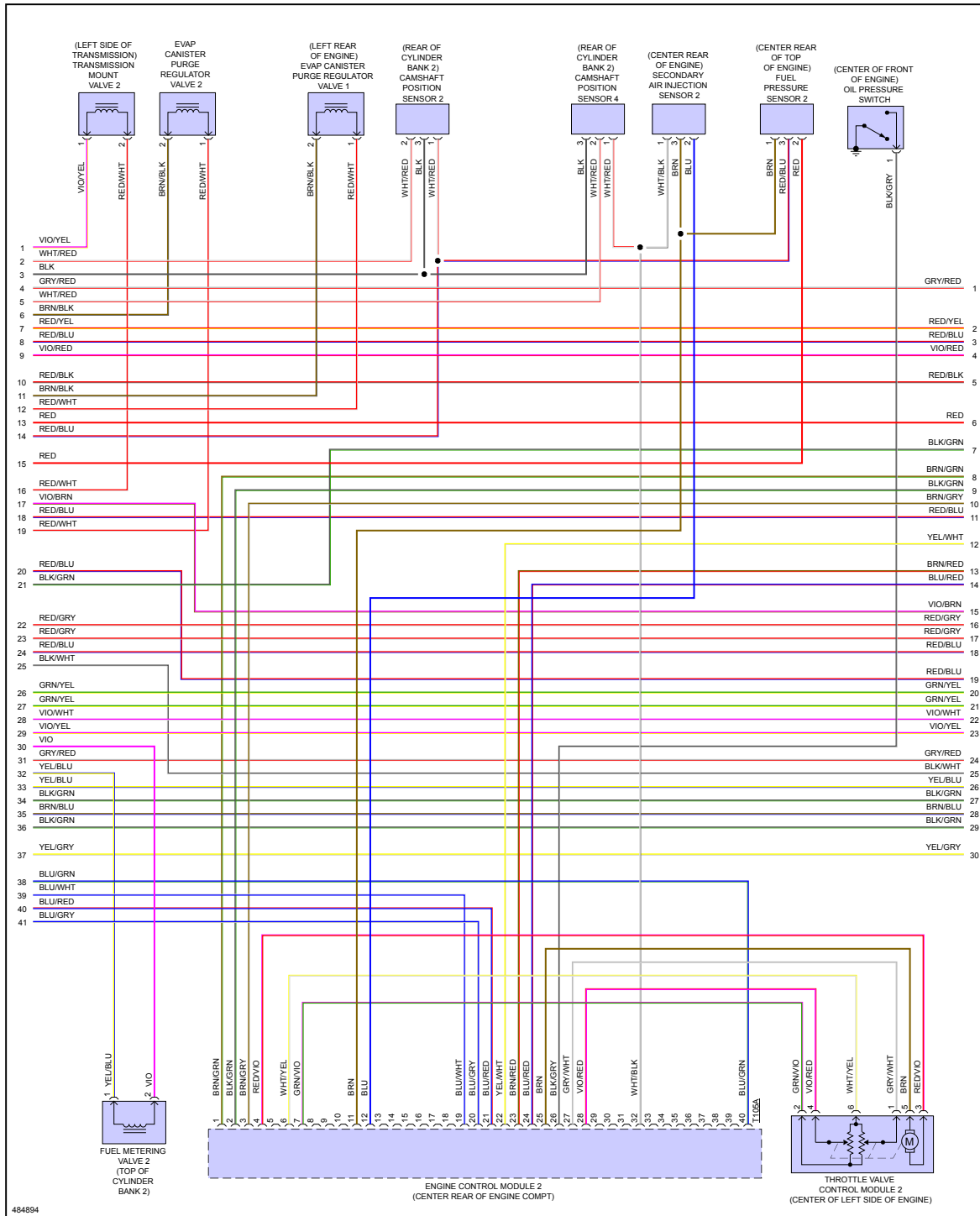
Fig 9: 6.3L, Engine Performance Circuit (9 of 11)
