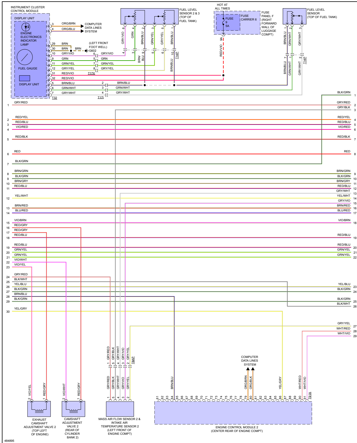
Fig 10: 6.3L, Engine Performance Circuit (10 of 11)
