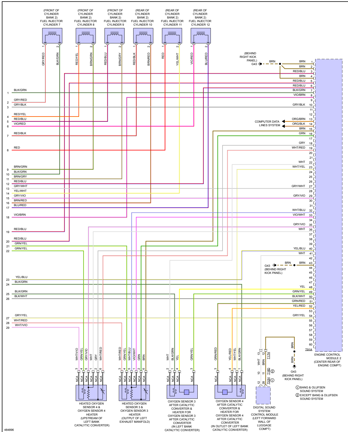
Fig 11: 6.3L, Engine Performance Circuit (11 of 11)
