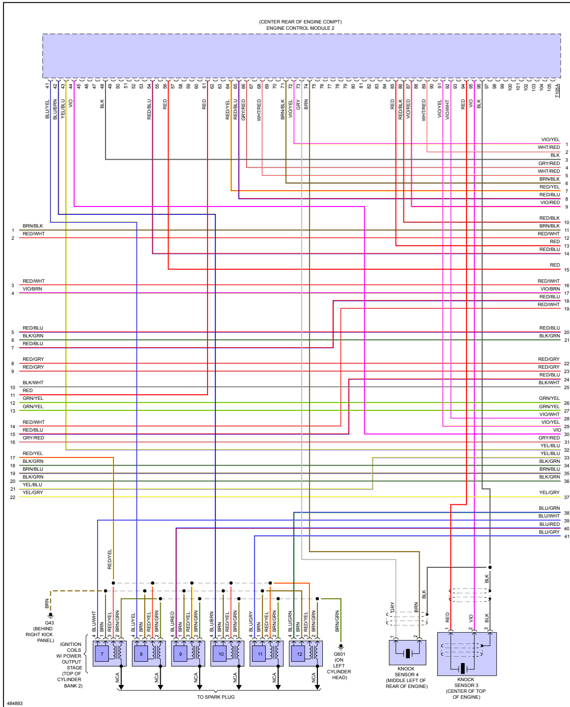
Fig 8: 6.3L, Engine Performance Circuit (8 of 11)
