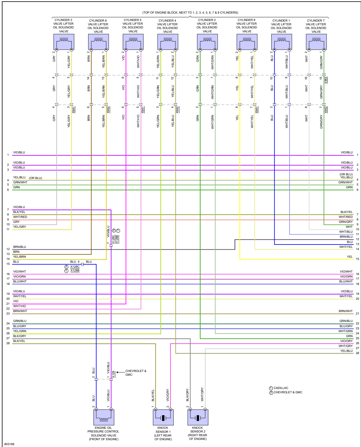
Fig 5: 6.2L VIN L, Engine Performance Circuit (5 of 7)
