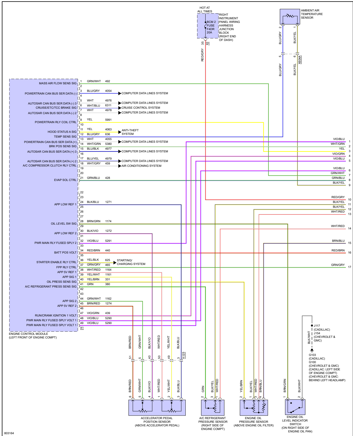
Fig 1: 6.2L VIN L, Engine Performance Circuit (1 of 7)
