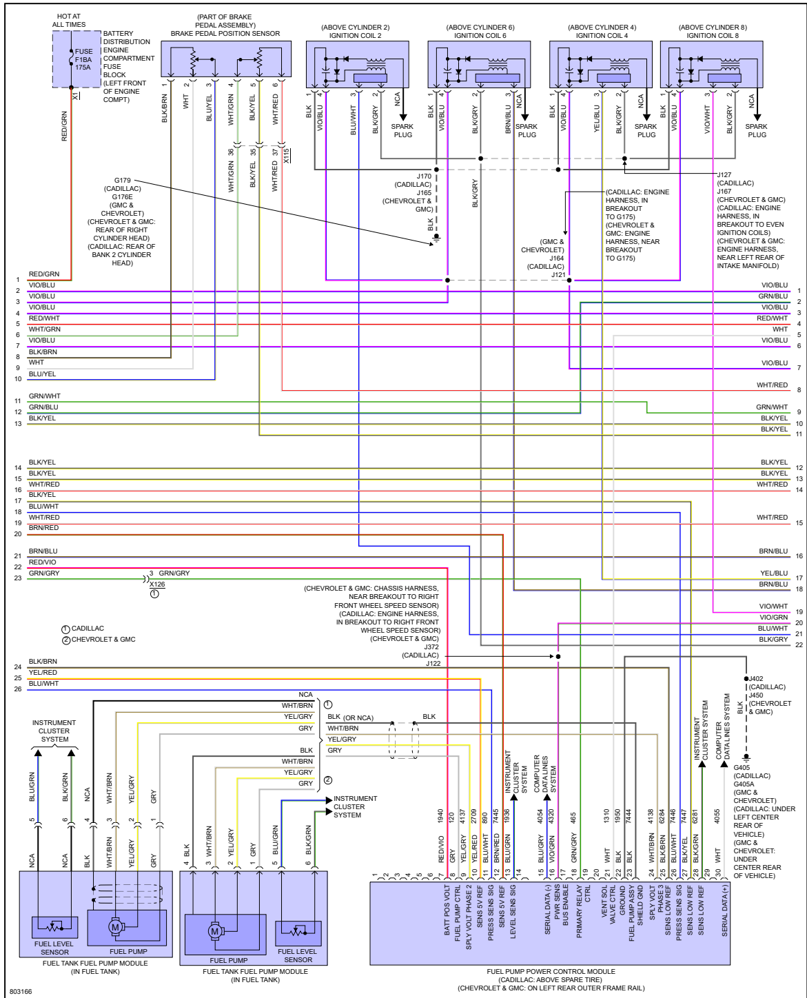
Fig 3: 6.2L VIN L, Engine Performance Circuit (3 of 7)
