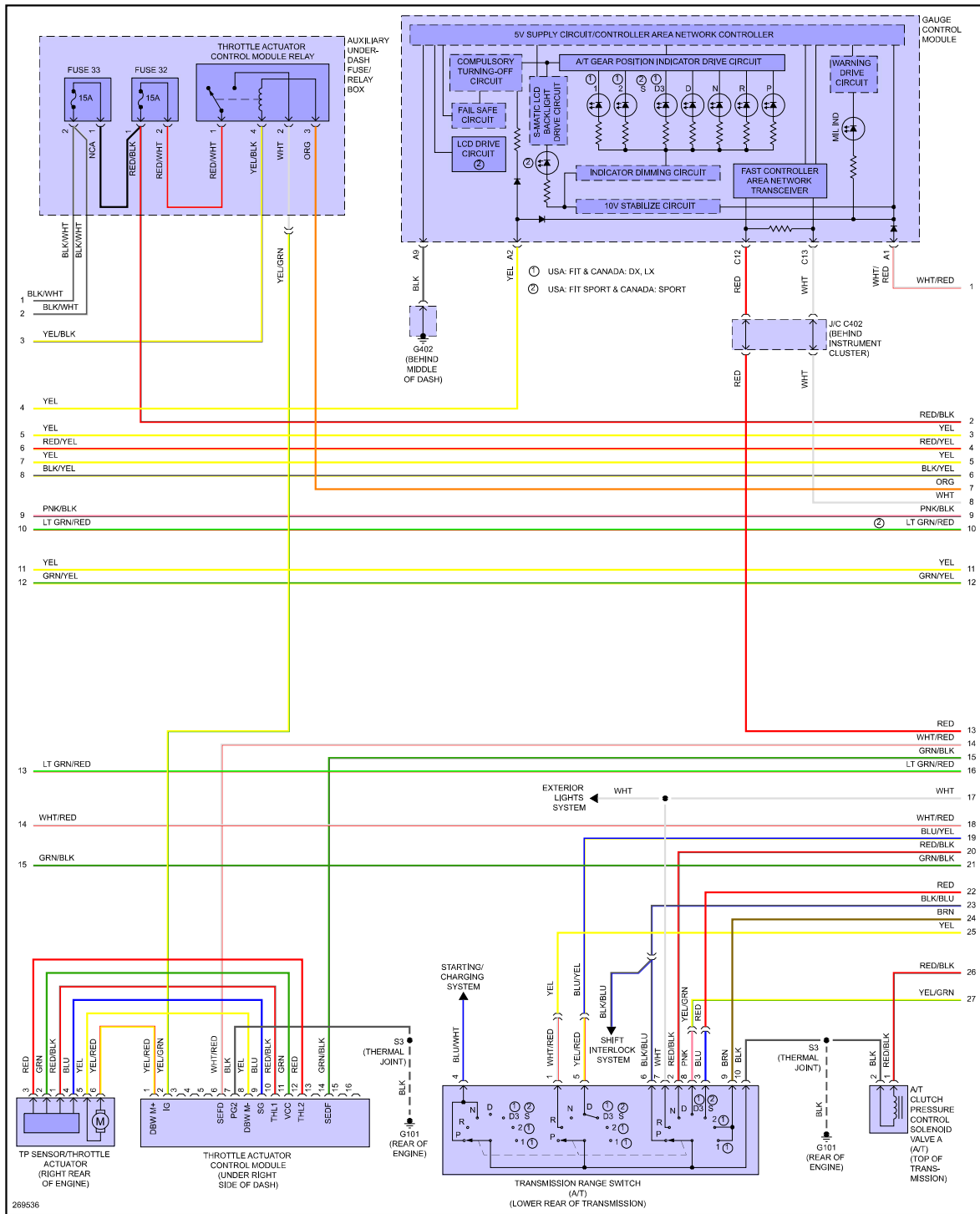
Fig 3: 1.5L, Engine Performance Circuit (3 of 4)
