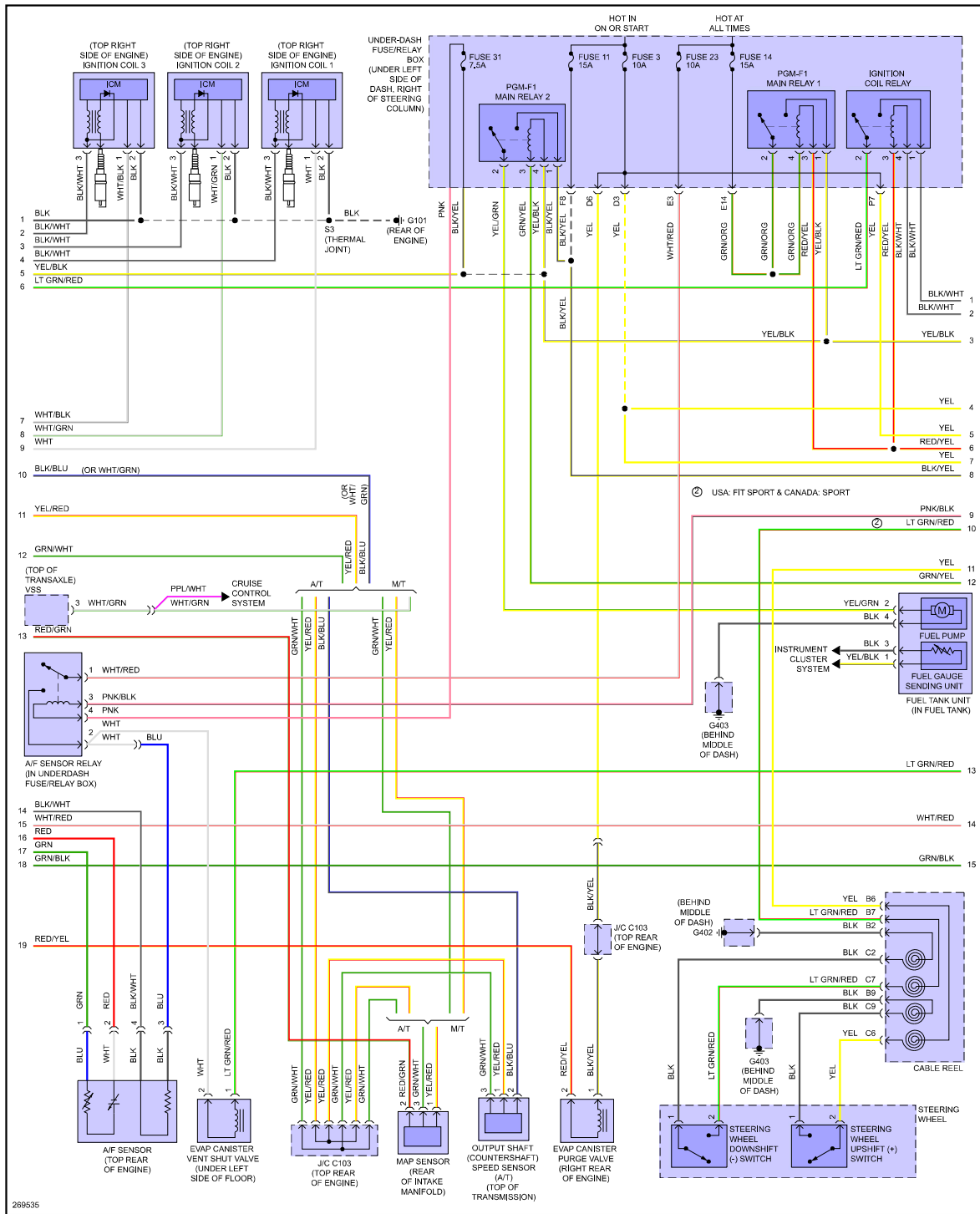
Fig 2: 1.5L, Engine Performance Circuit (2 of 4)
