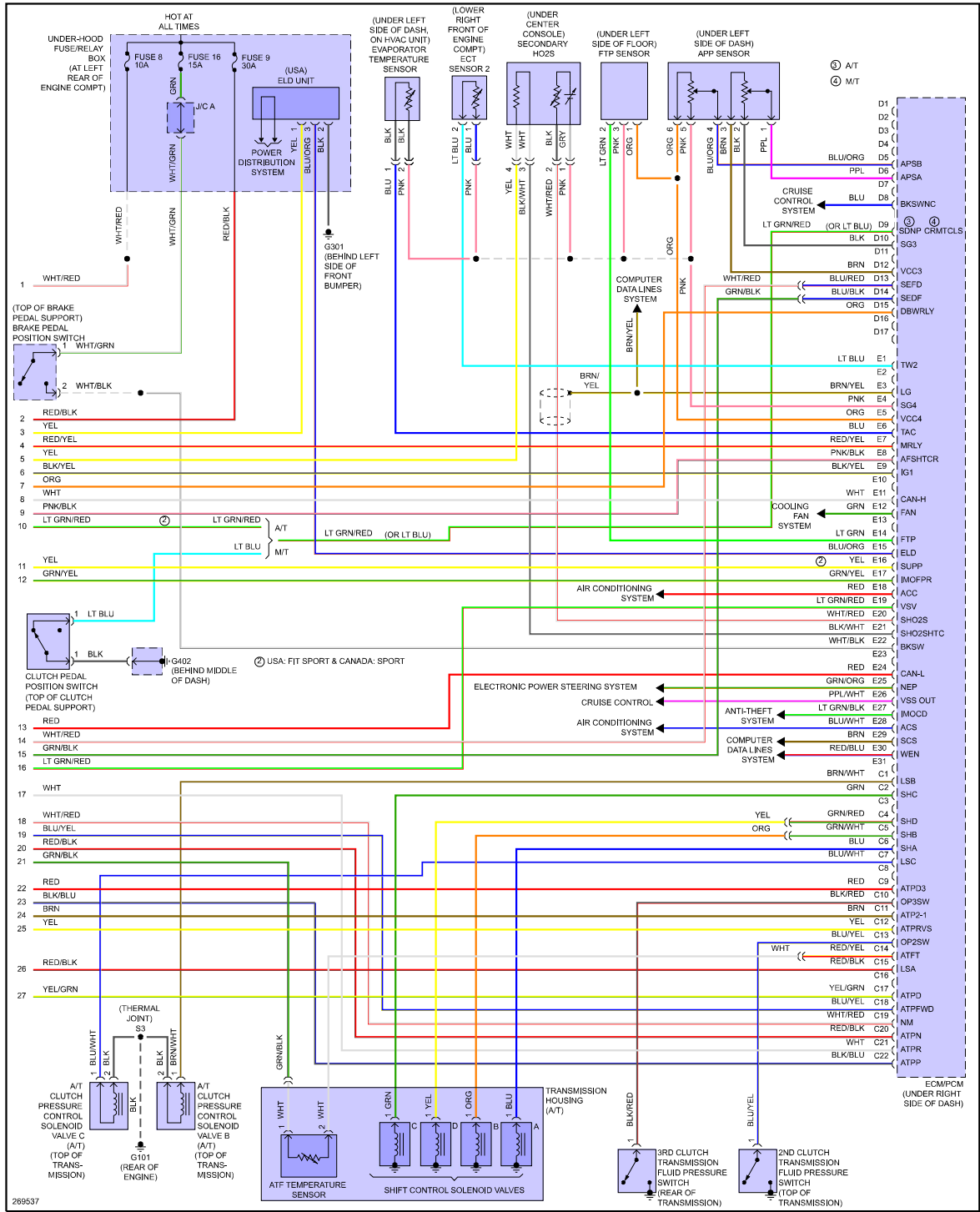
Fig 4: 1.5L, Engine Performance Circuit (4 of 4)
