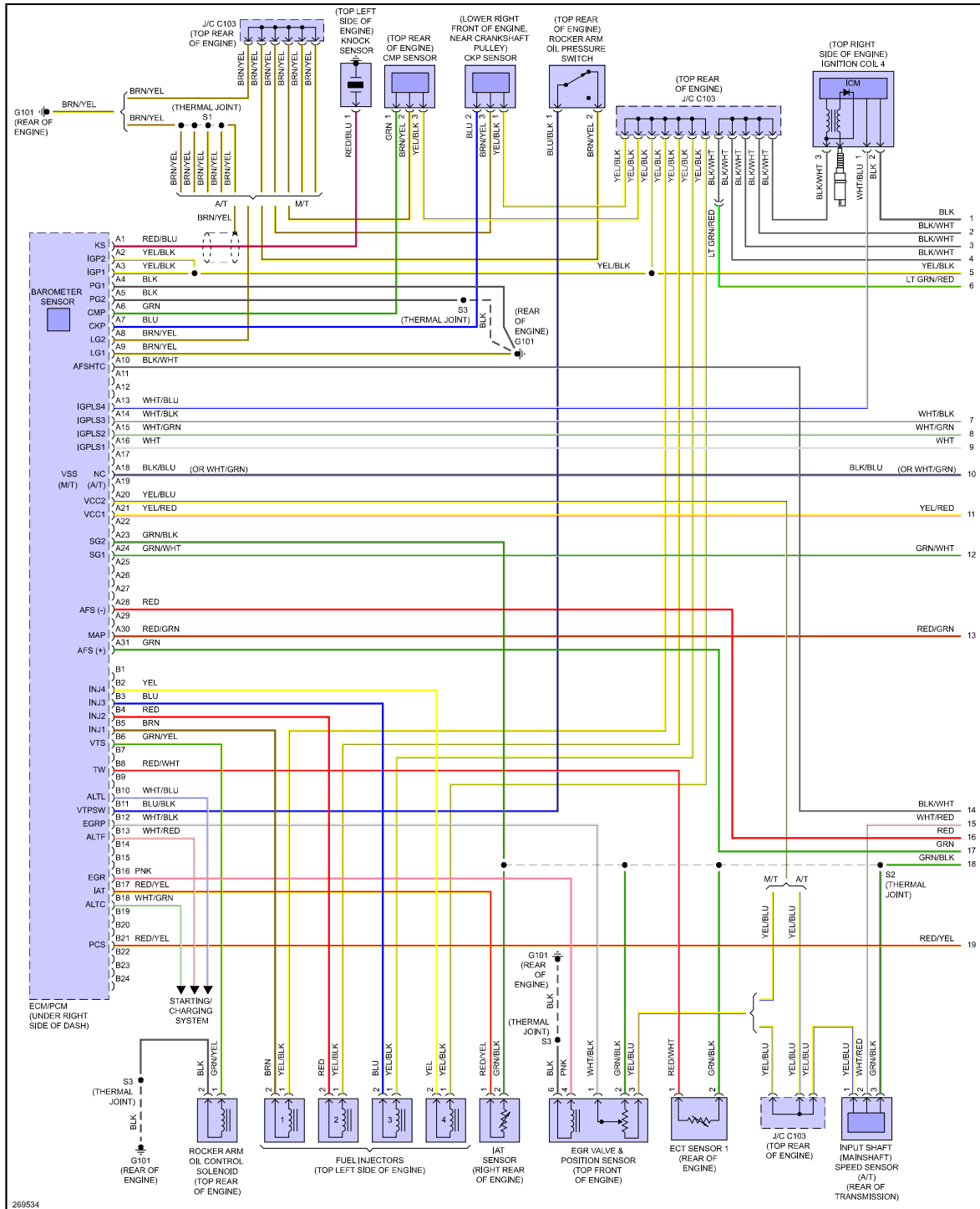
Fig 1: 1.5L, Engine Performance Circuit (1 of 4)
