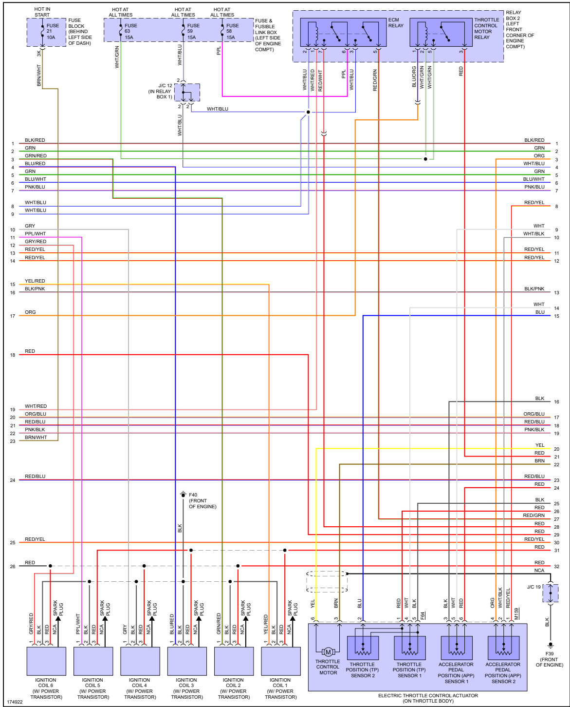
Fig 2: 3.5L, Engine Performance Circuit (2 of 4)
