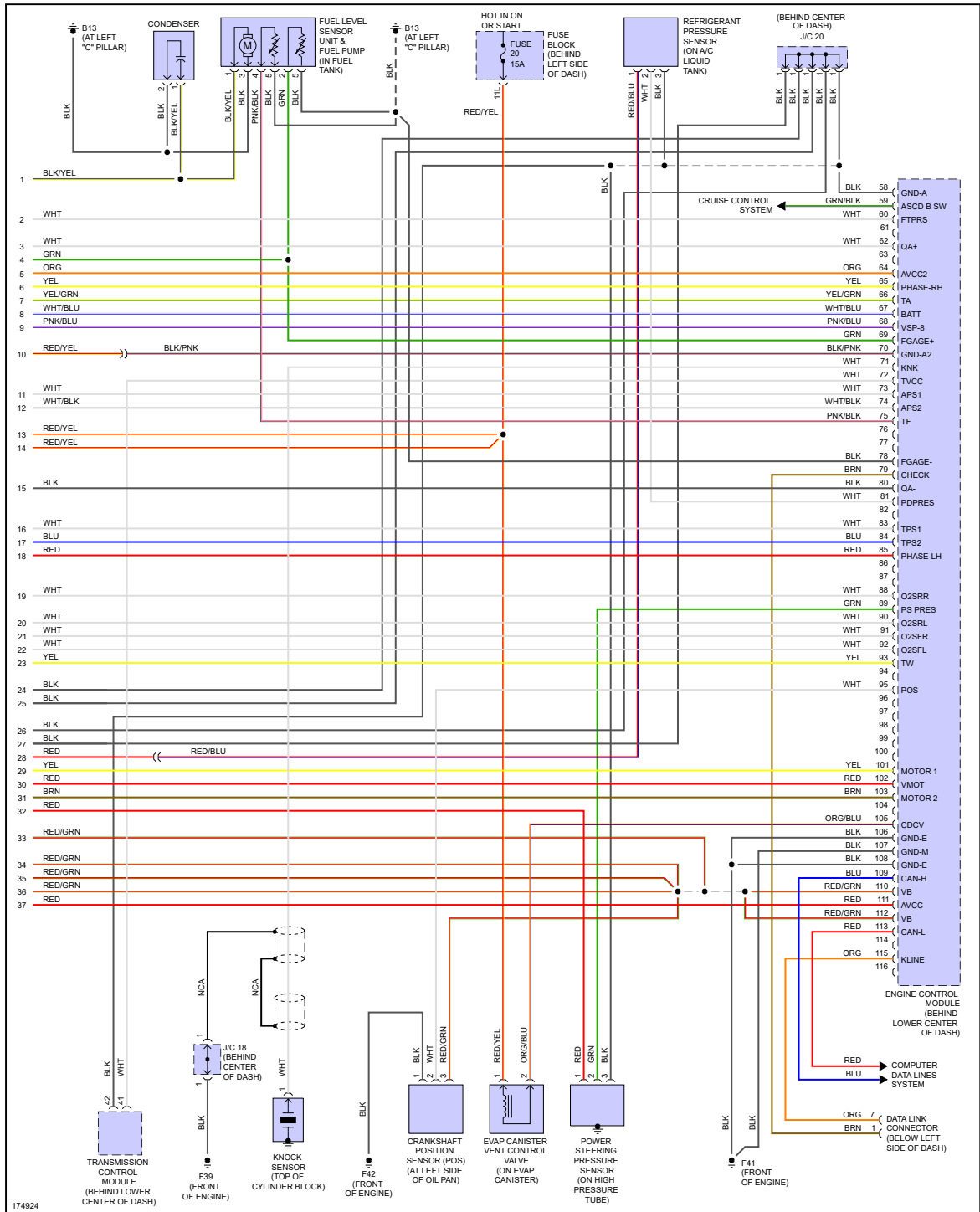
Fig 4: 3.5L, Engine Performance Circuit (4 of 4)
