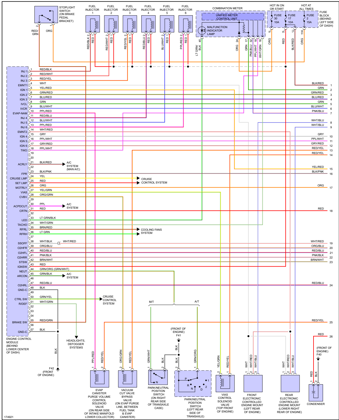
Fig 1: 3.5L, Engine Performance Circuit (1 of 4)
