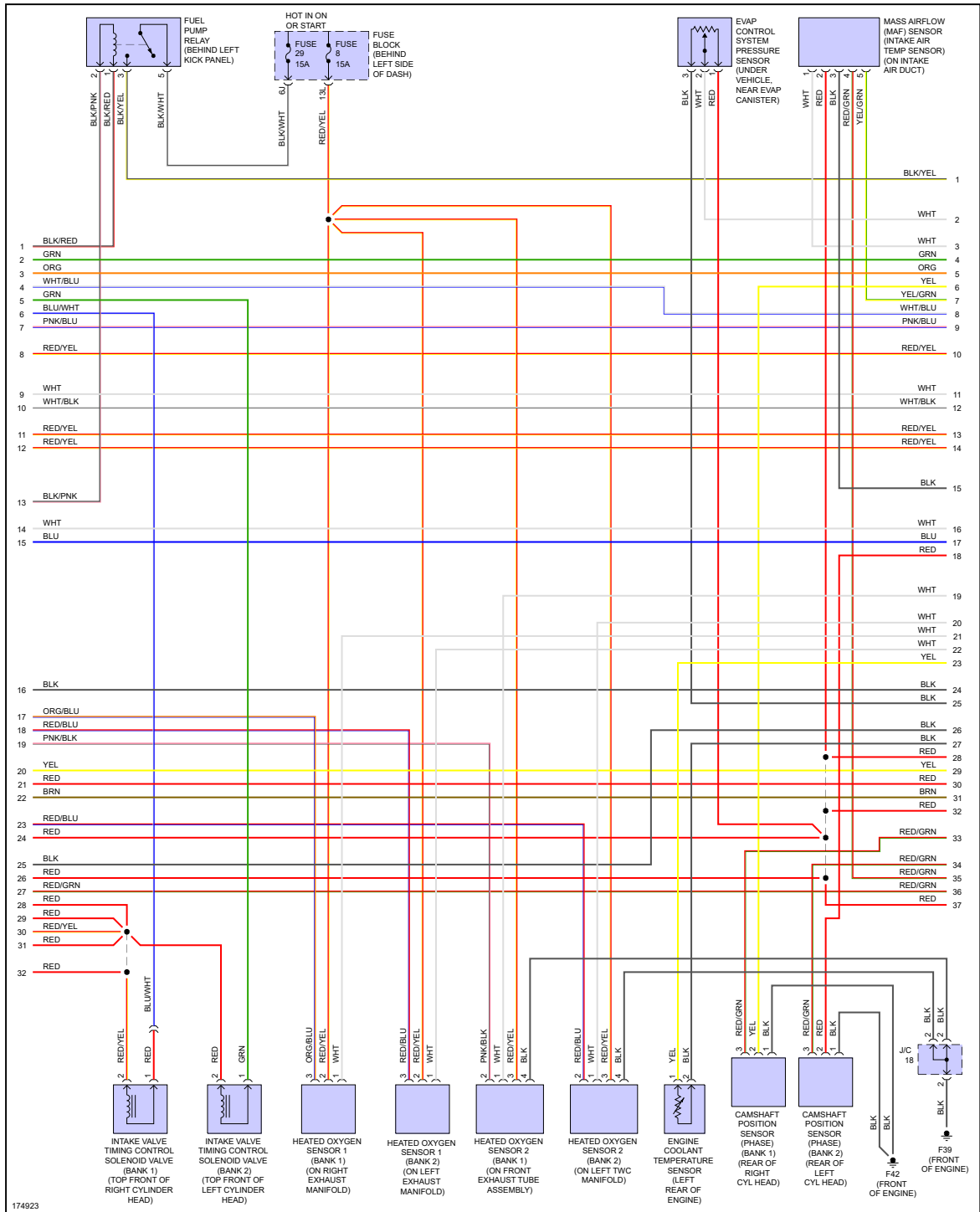
Fig 3: 3.5L, Engine Performance Circuit (3 of 4)
